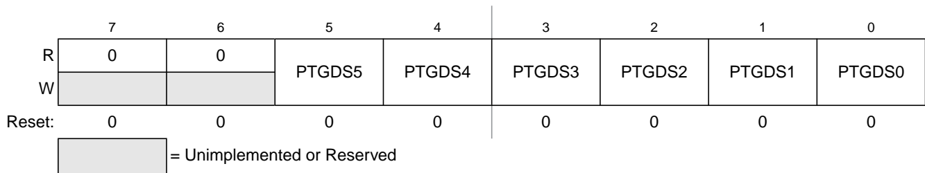
Figure 6-46. Drive Strength Selection for Port G Register (PTGDS)
