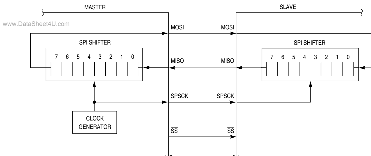
Figure 14-2. SPI System Connections
