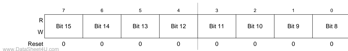
Figure 8-3. CRC High Register (CRCH)
