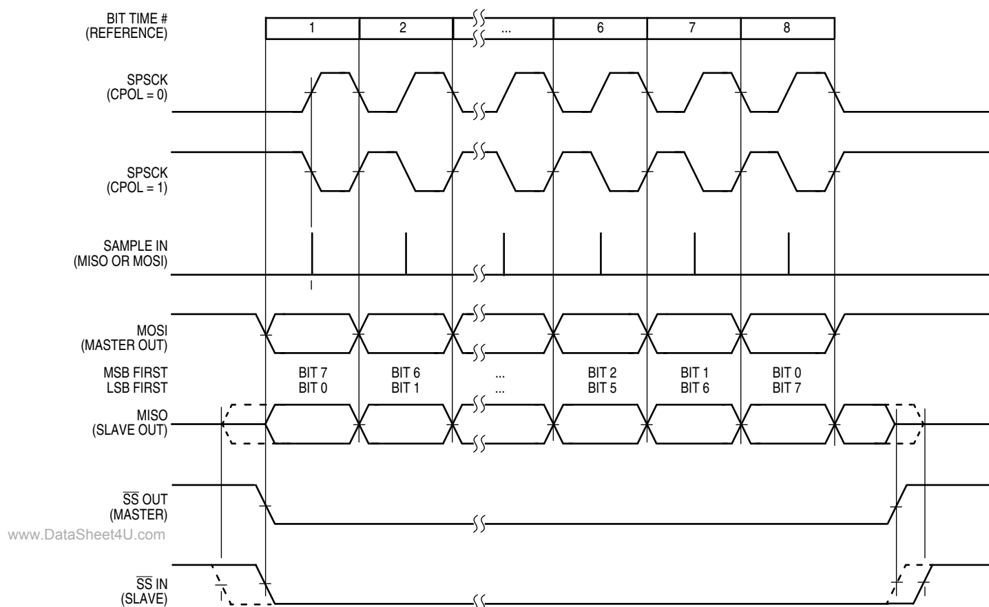
Figure 14-11. SPI Clock Formats (CPHA = 0)
