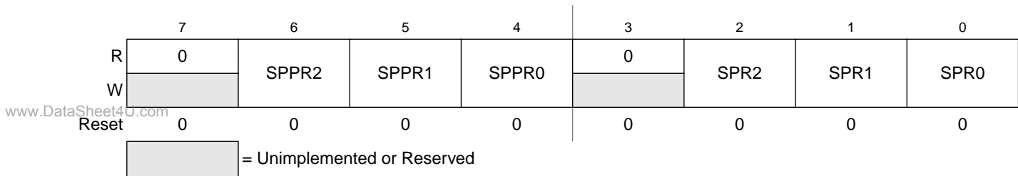
Figure 14-7. SPI Baud Rate Register (SPIBR)
