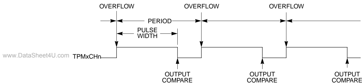
Figure 15-15. PWM Period and Pulse Width (ELSnA=0)
