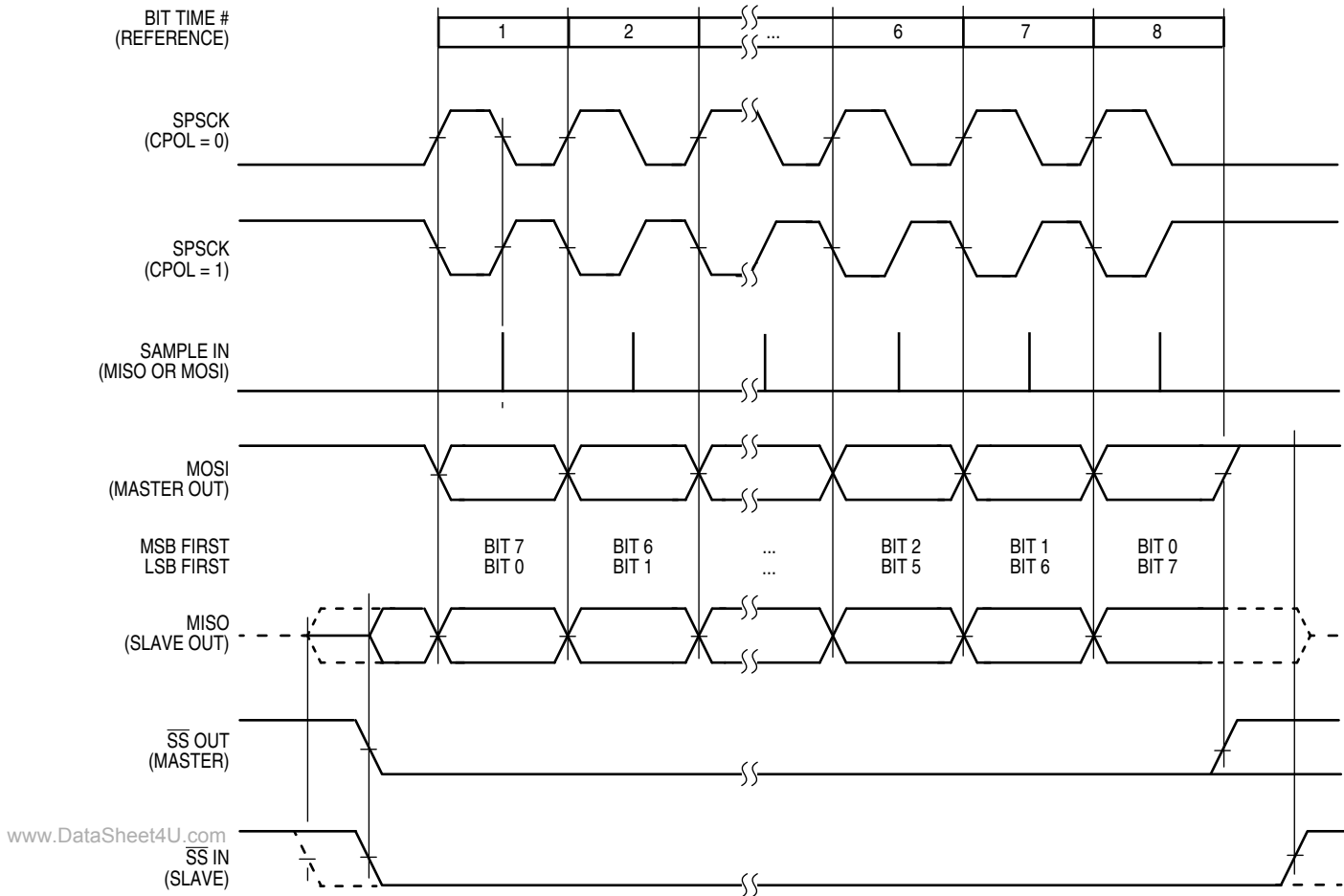
Figure 14-10. SPI Clock Formats (CPHA = 1)
