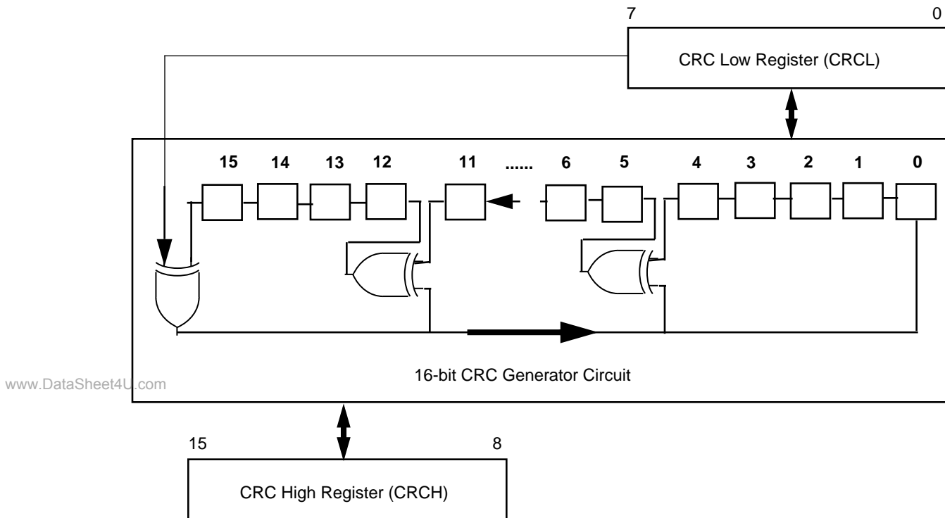
Figure 8-2. Cyclic Redundancy Check (CRC) Module Block Diagram
