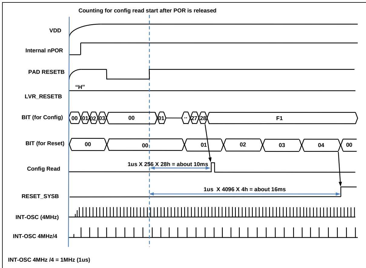
Figure 14.5 Configuration Timing when Power-on
