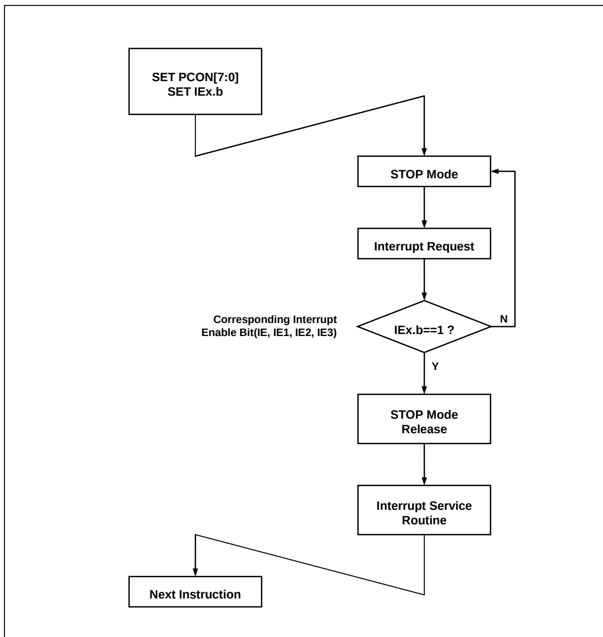
Figure 13.3 STOP Mode Release Flow
