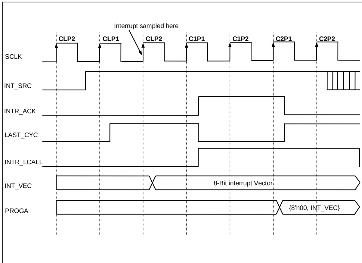
Figure 11.10 Timing Chart of Interrupt Acceptance and Interrupt Return Instruction
