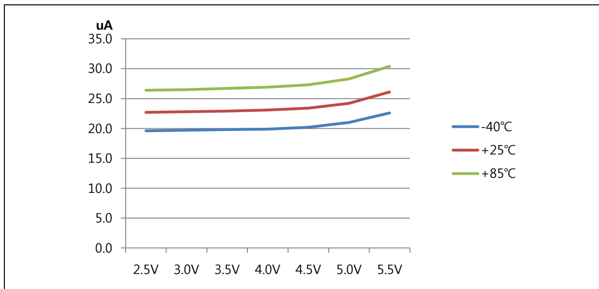
Figure 8.19 SUB RUN (IDD3) Current
