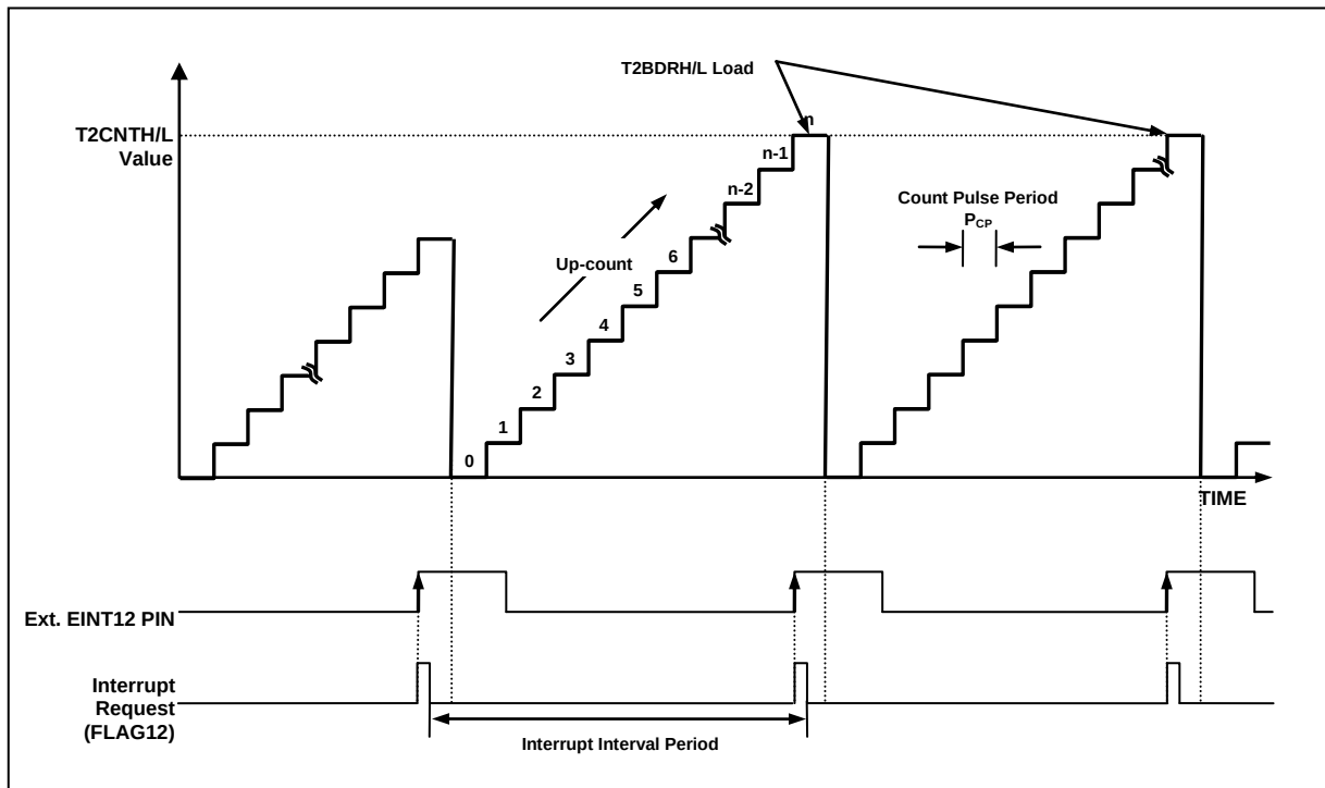
Figure 12.23 Input Capture Mode Operation for Timer 2
