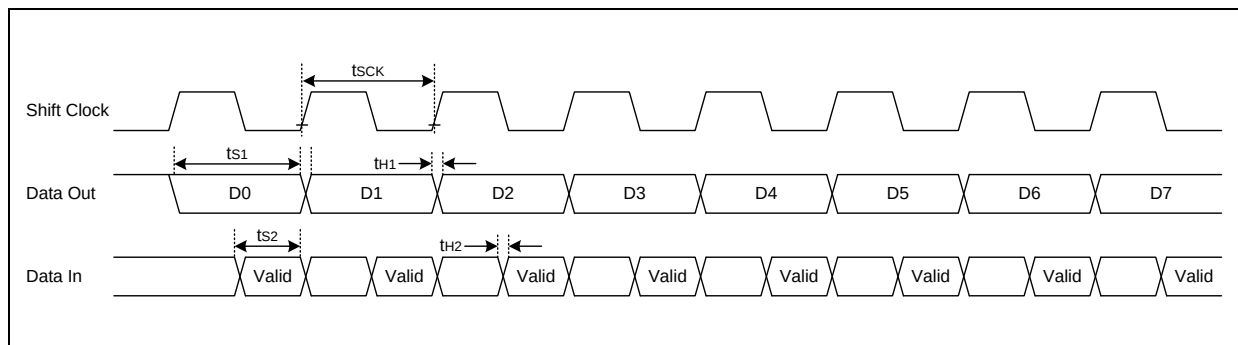
Figure 8.6 Timing Waveform for the UART Module
