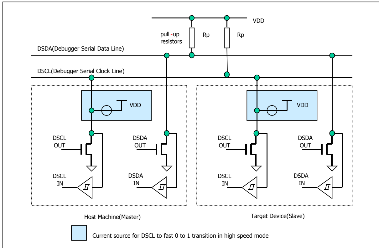
Figure 15.8 Connection of Transmission
