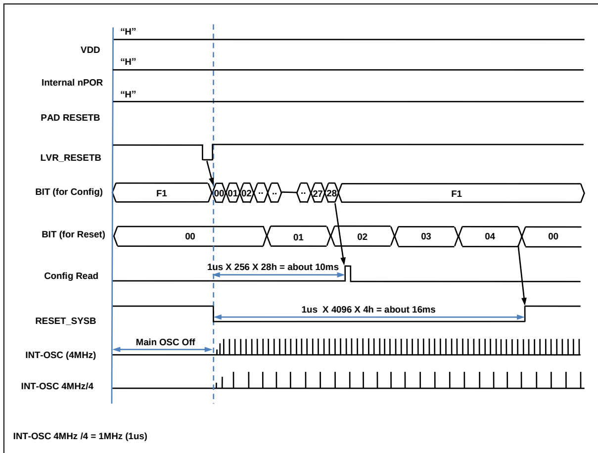
Figure 14.11 Configuration timing when BOD RESET
