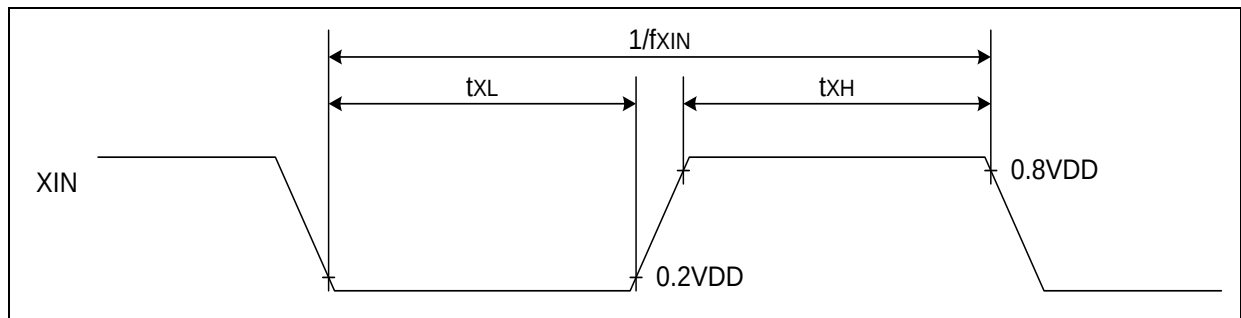
Figure 8.13 Clock Timing Measurement at XIN
