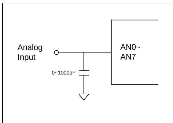
Figure 12.42 A/D Analog Input Pin with Capacitor
