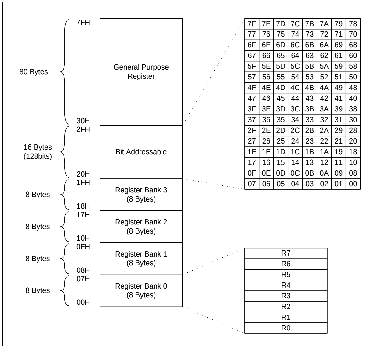
Figure 9.3 Lower 128 Bytes RAM
