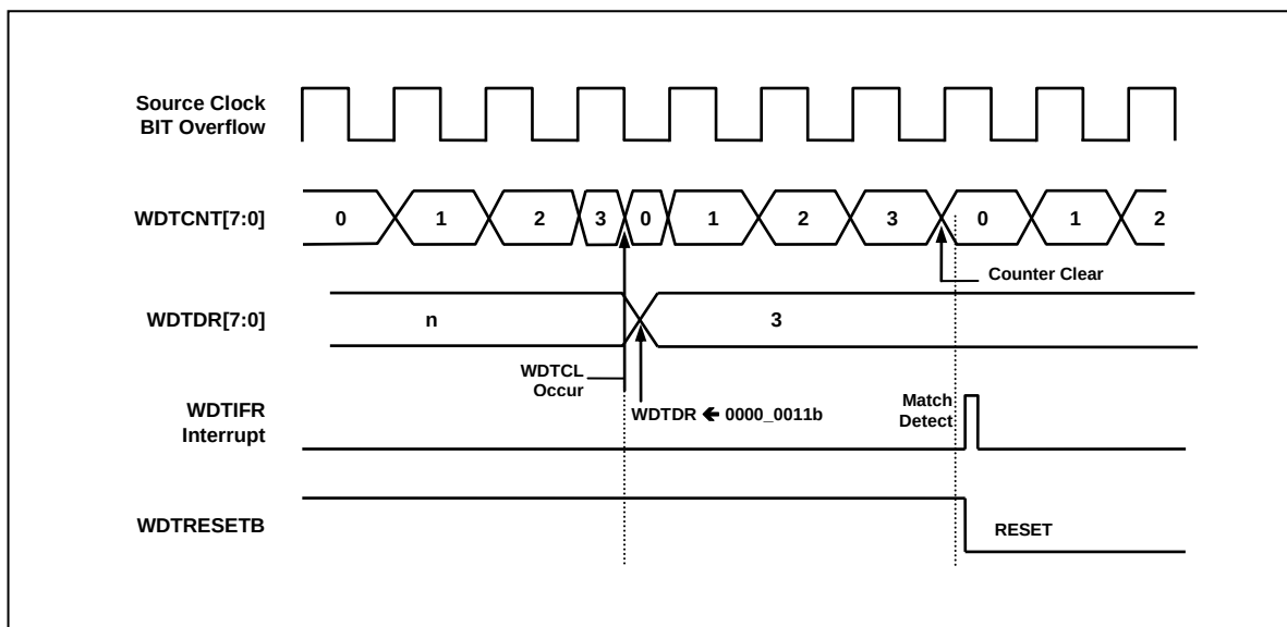
Figure 12.3 Watch Dog Timer Interrupt Timing Waveform
