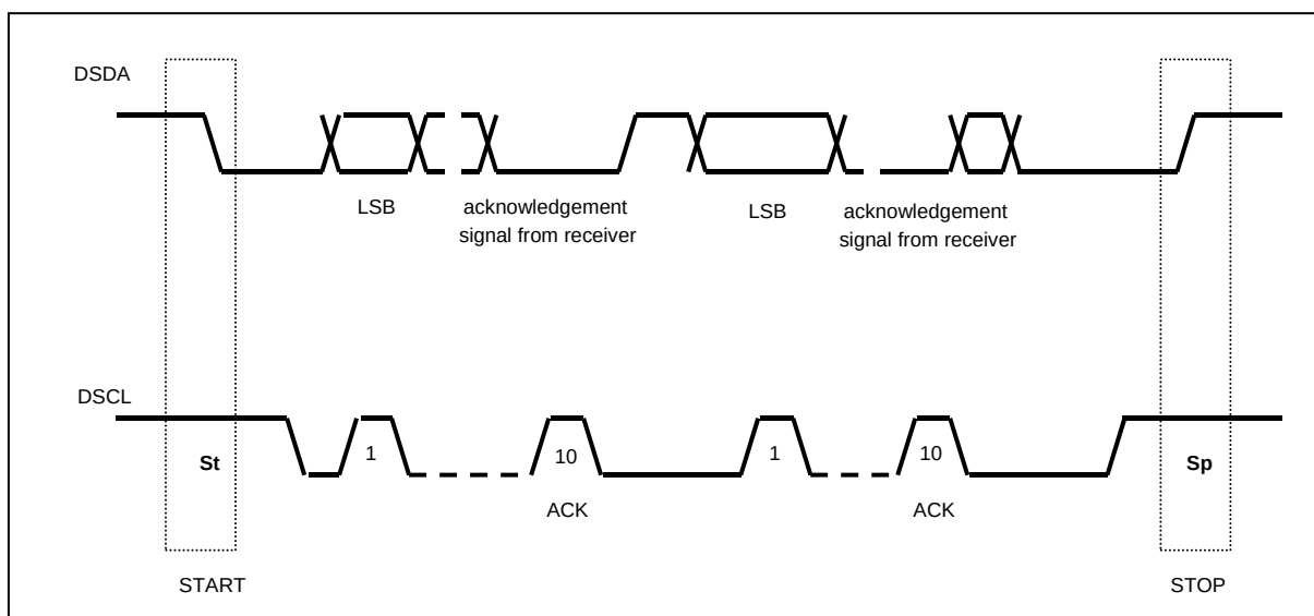
Figure 15.3 Data Transfer on the Twin Bus
