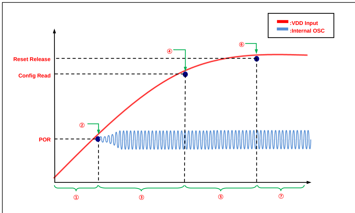
Figure 14.6 Boot Process Wave Form
