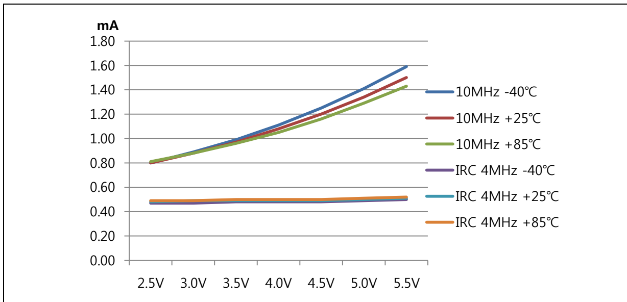
Figure 8.18 IDLE (IDD2) Current
