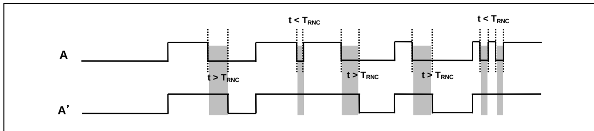
Figure 14.2 Reset noise canceller timer diagram
