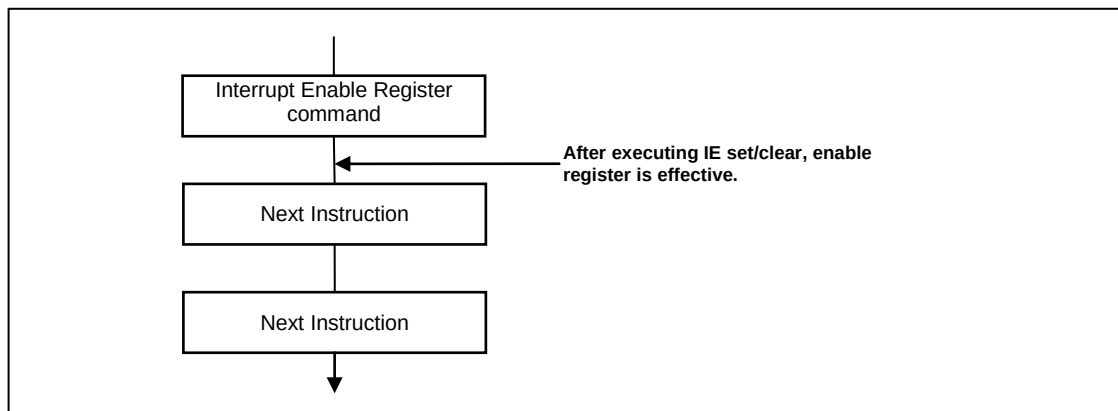
Figure 11.4 Effective Timing of Interrupt Enable Register
