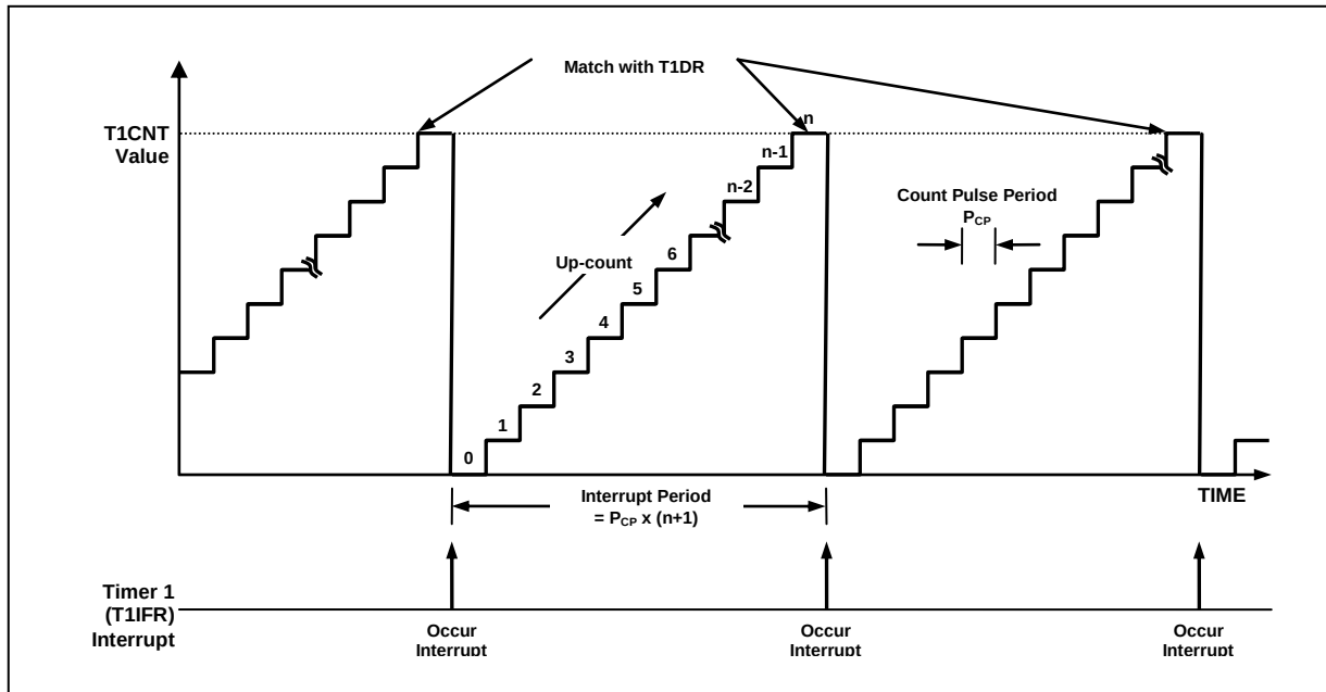
Figure 12.15 8-Bit Timer/Counter 1 Example
