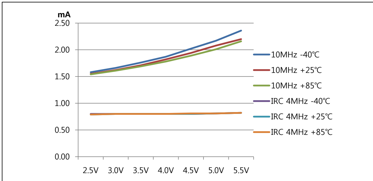
Figure 8.17 RUN (IDD1) Current
