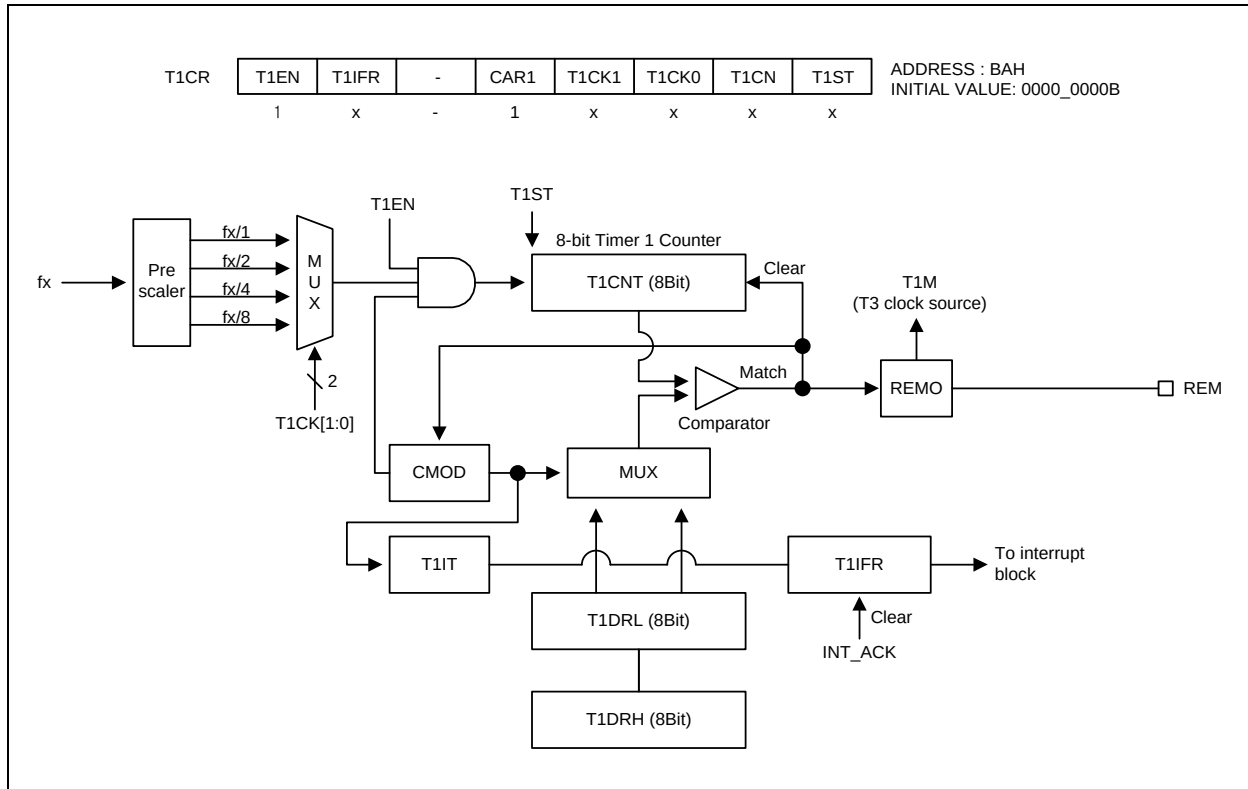
Figure 12.17 Carrier Mode for Timer 1
