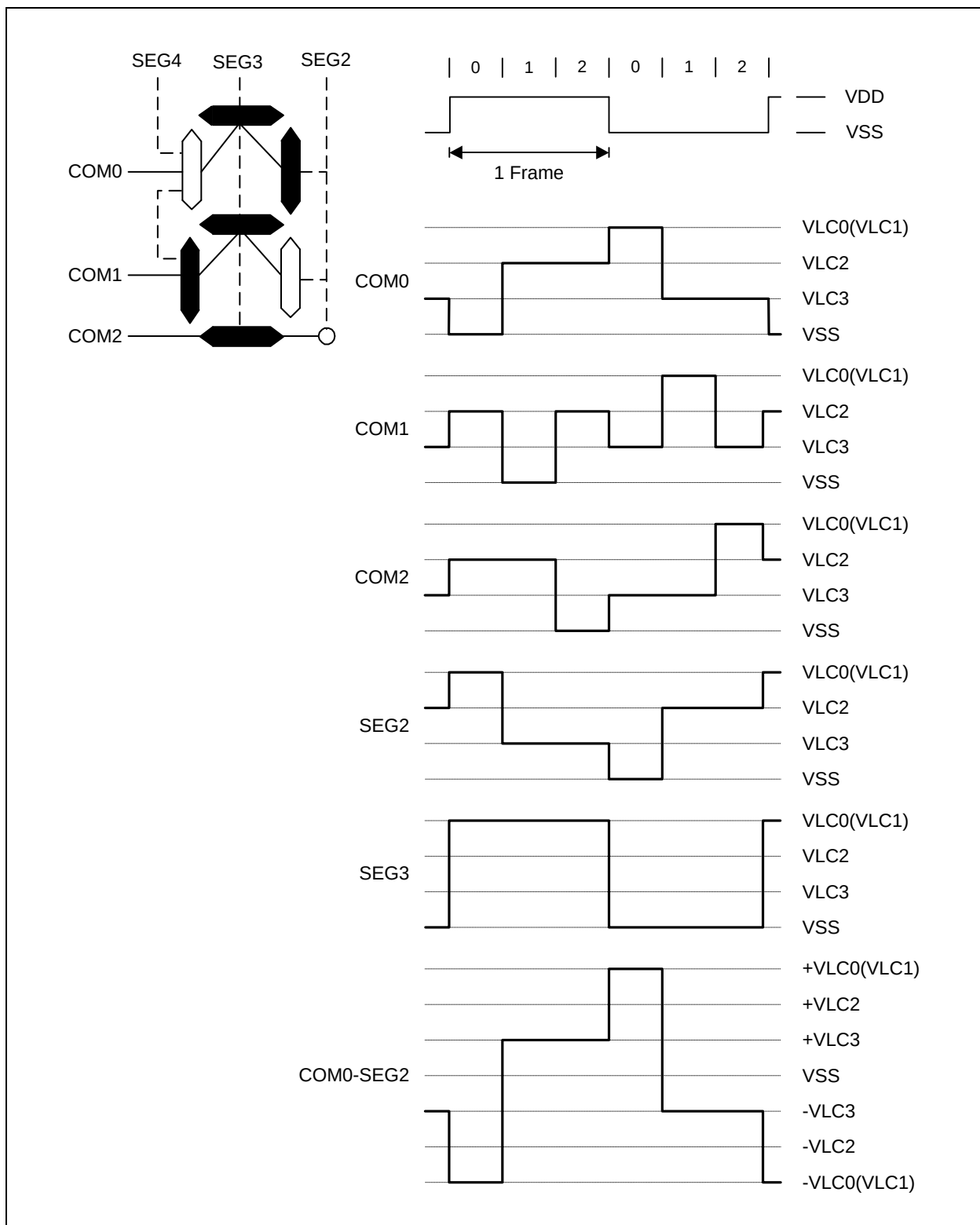
Figure 12.55 LCD Signal Waveforms (1/3Duty, 1/3Bias)
