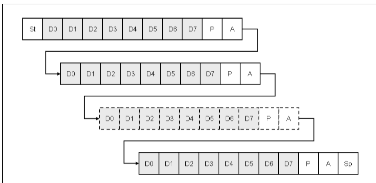
Figure 15.2 10-bit Transmission Packet
