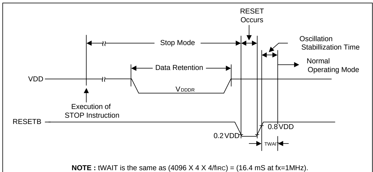
Figure 8.8 Stop Mode Release Timing when Initiated by RESETB
