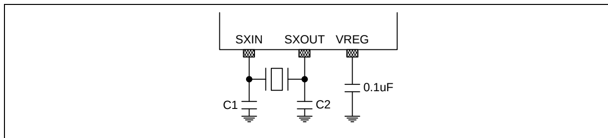
Figure 7.11 Crystal Oscillator
