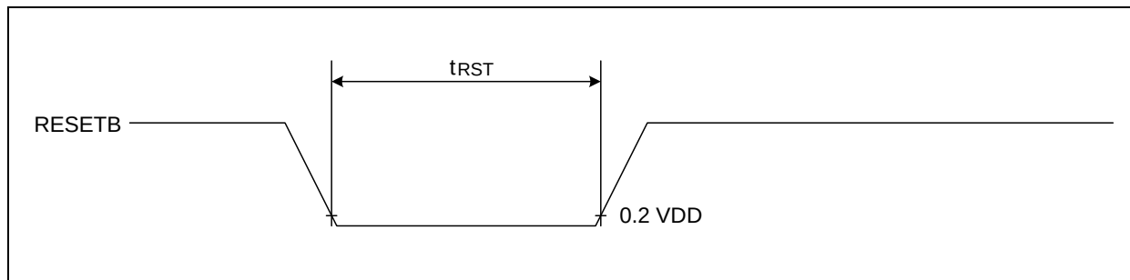
Figure 8.1 Input Timing for RESETB
