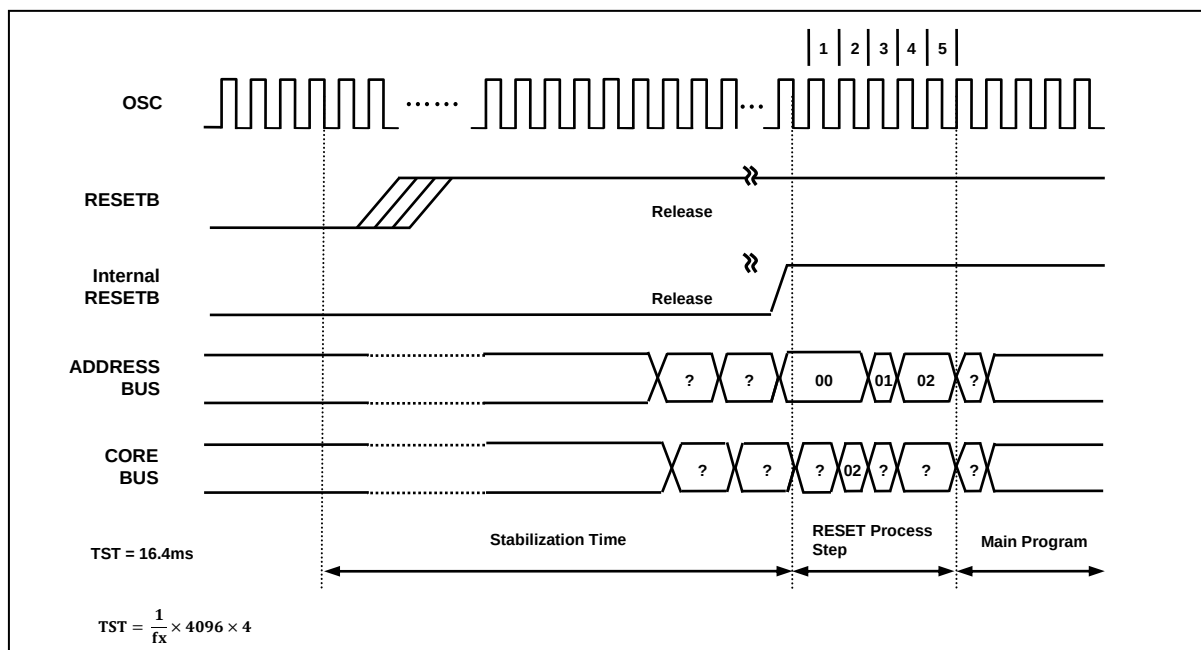
Figure 14.7 Timing Diagram after RESET
