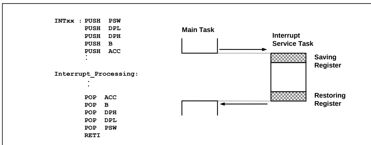
Figure 11.9 Saving/Restore Process Diagram and Sample Source
