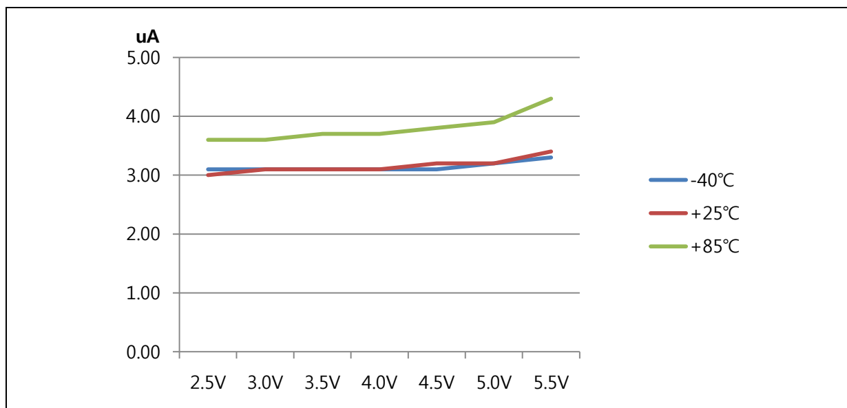
Figure 8.20 SUB IDLE (IDD4) Current
