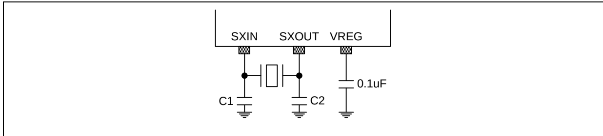
Figure 8.11 Crystal Oscillator
