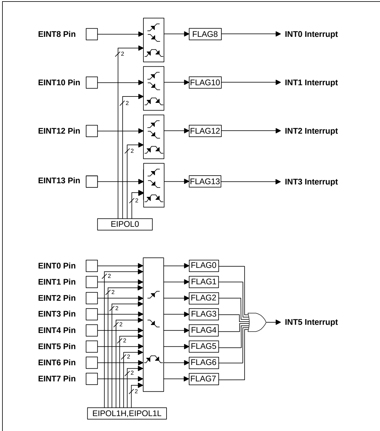
Figure 11.1 External Interrupt Description
