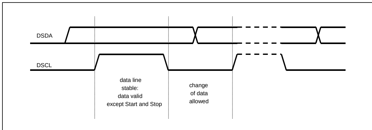
Figure 15.4 Bit Transfer on the Serial Bus
