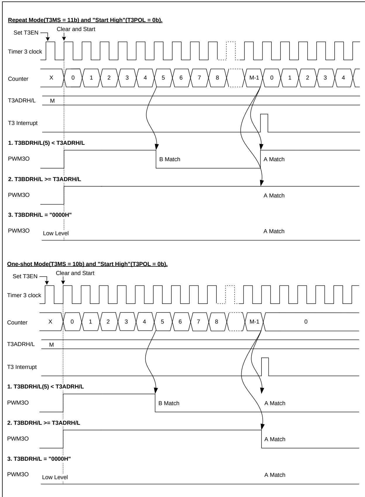
Figure 12.34 16-Bit PPG Mode Timing chart for Timer 3
