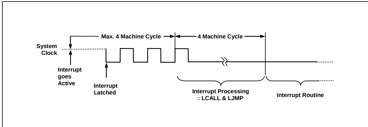
Figure 11.7 Interrupt Response Timing Diagram
