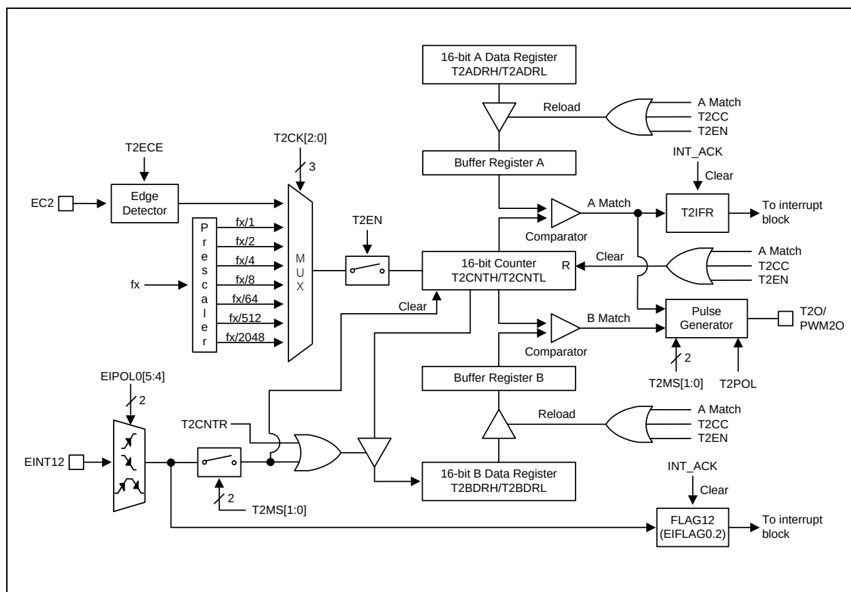
Figure 12.27 16-Bit Timer/Counter Mode for Timer 2 and Block Diagram
