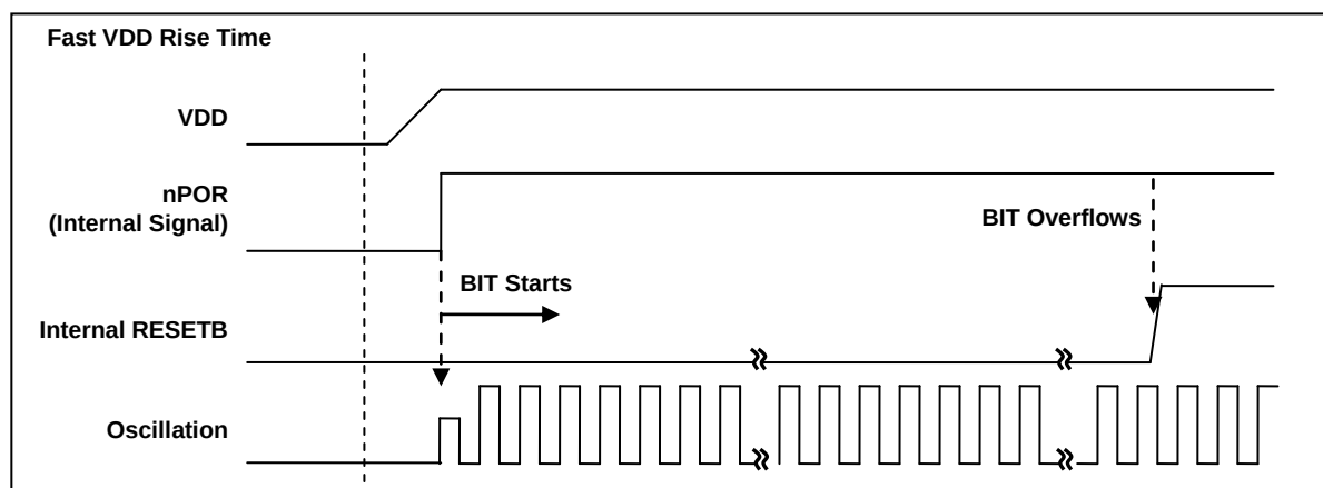
Figure 14.3 Fast VDD Rising Time
