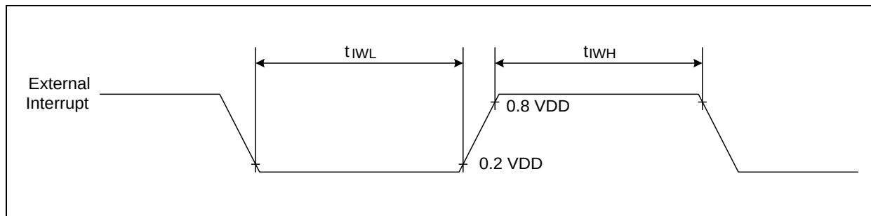
Figure 8.2 Input Timing for External Interrupts
