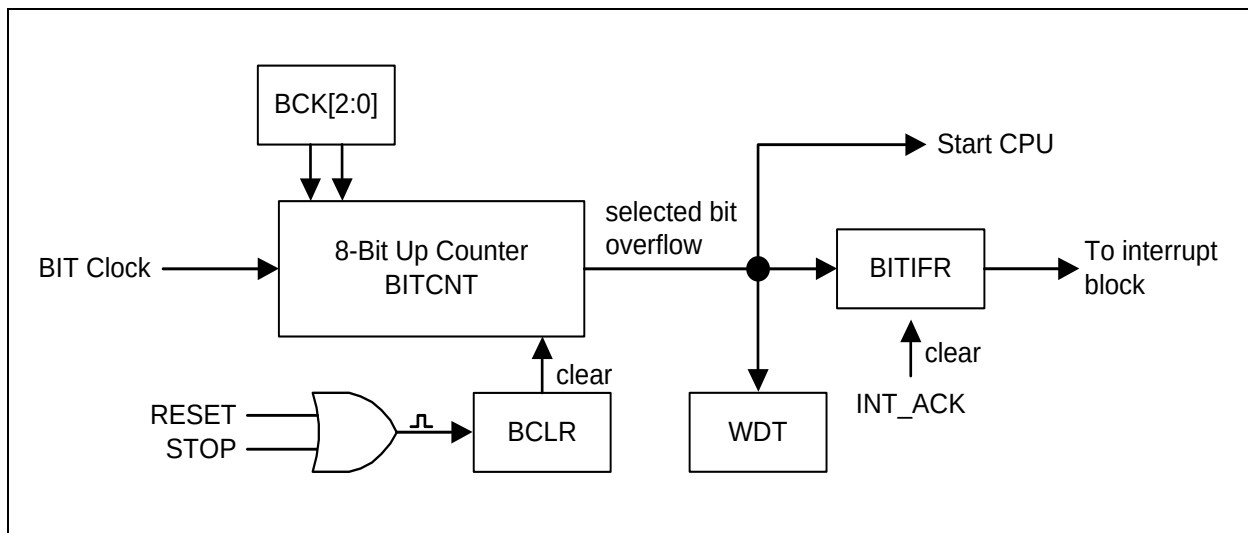
Figure 12.2 Basic Interval Timer Block Diagram
