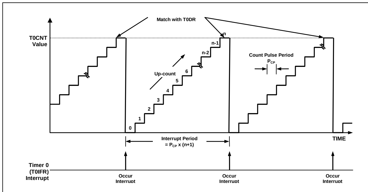
Figure 12.7 8-Bit Timer/Counter 0 Example
