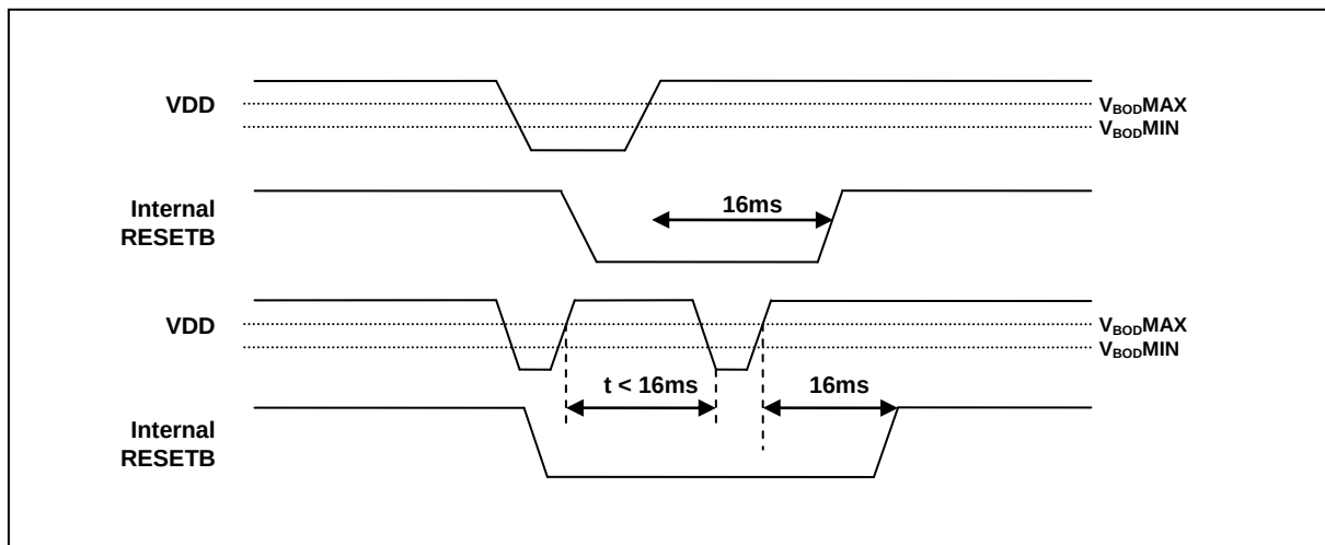
Figure 14.10 Internal Reset at the power fail situation
