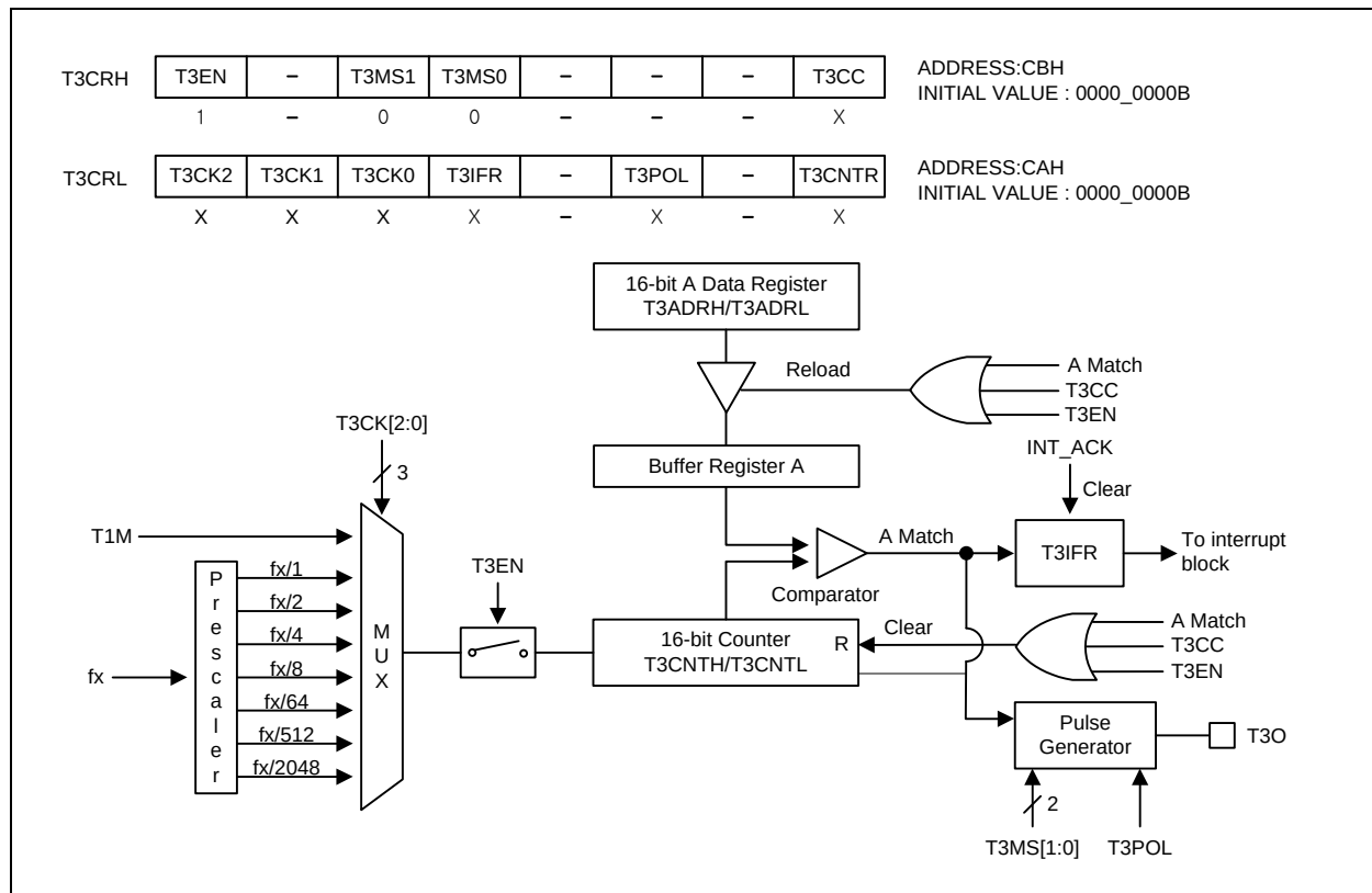
Figure 12.28 16-Bit Timer/Counter Mode for Timer 3
