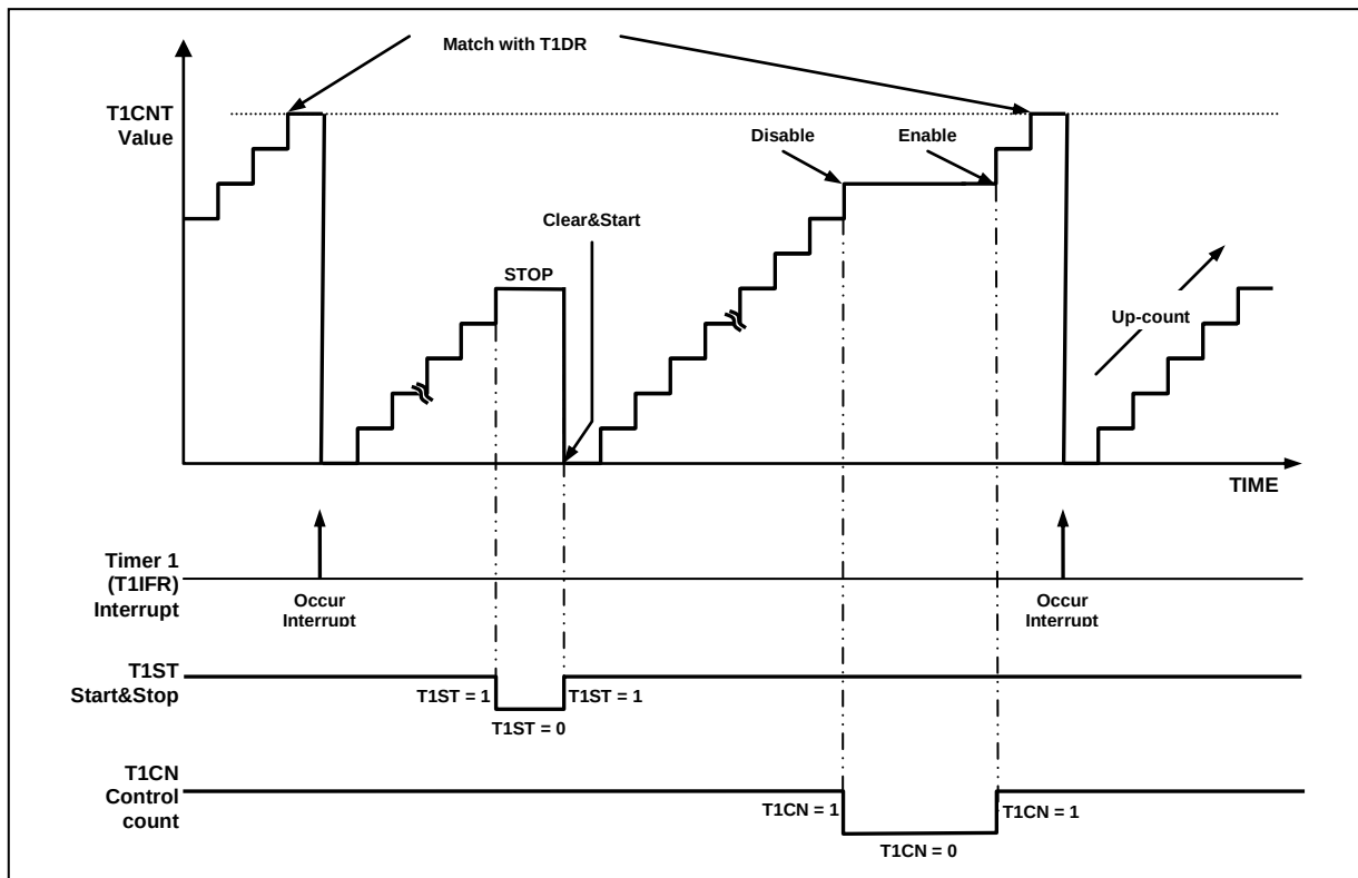
Figure 12.16 8-Bit Timer/Counter 1 Counter Operation
