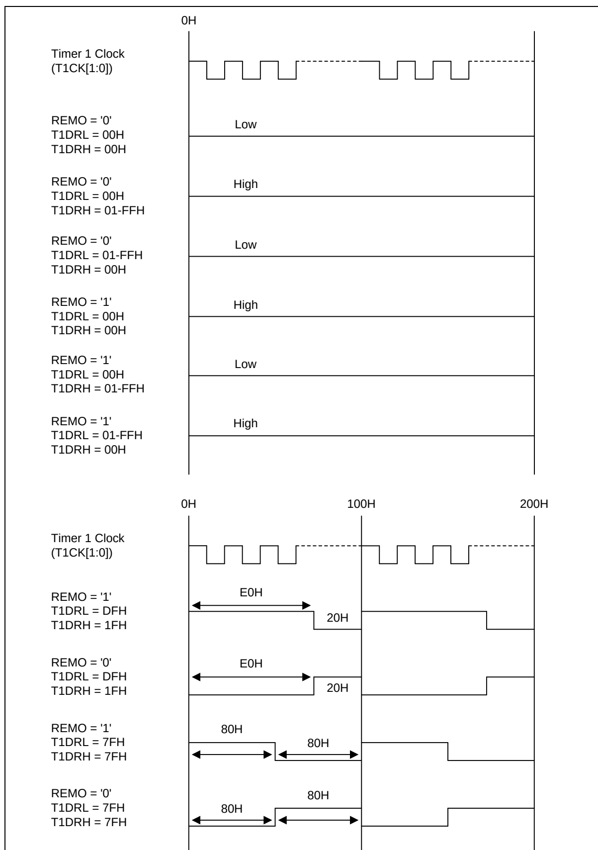
Figure 12.18 Carrier Output Waveforms in Repeat Mode for Timer 1
