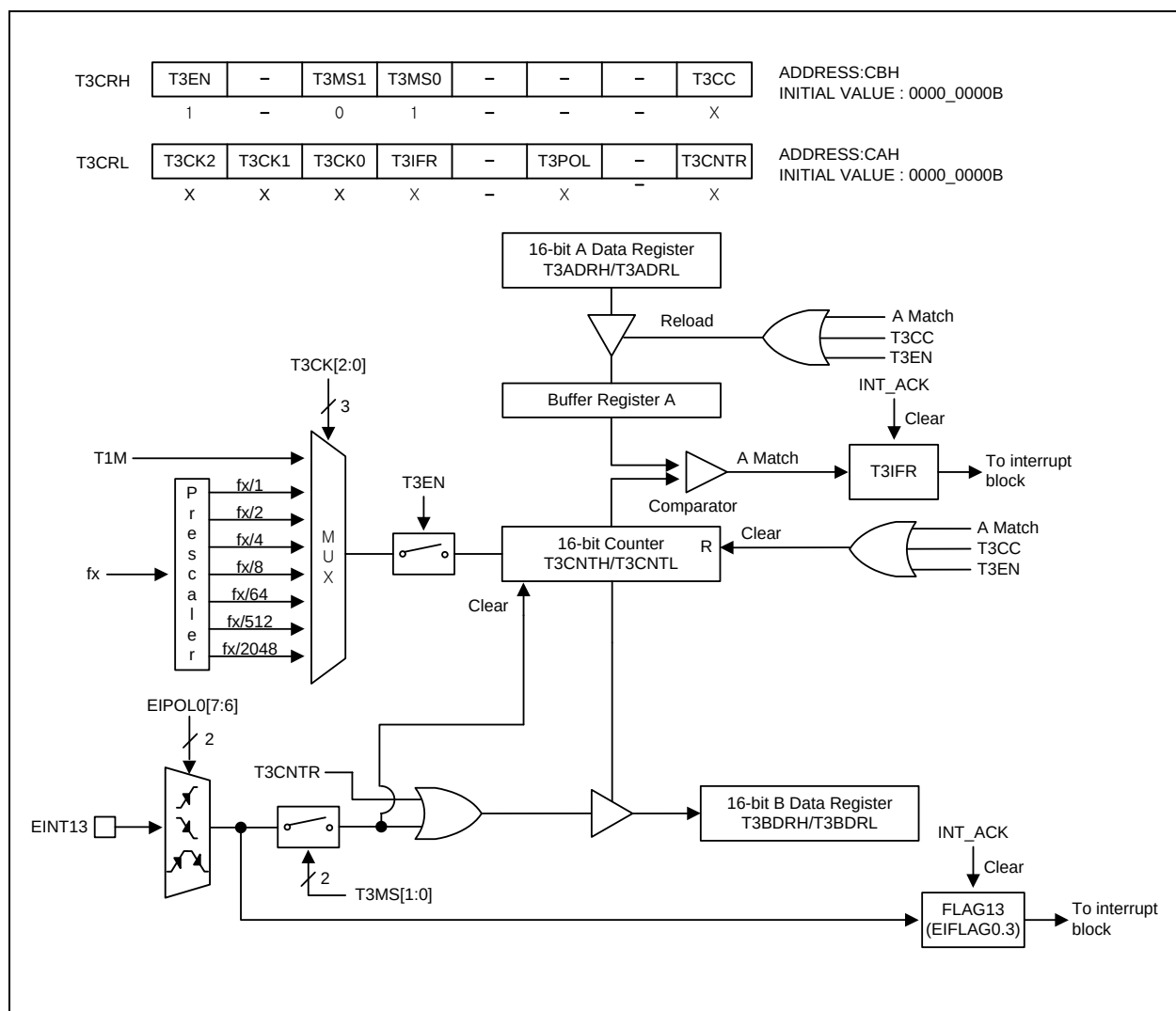
Figure 12.30 16-Bit Capture Mode for Timer 3
