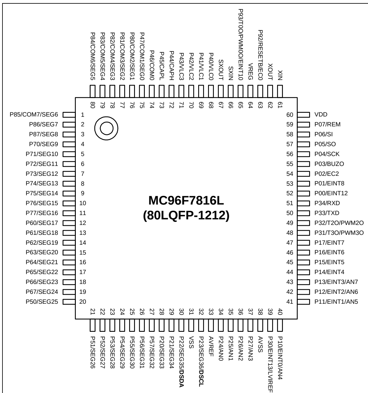
Figure 3.2 MC96F7816 80LQFP-1212 Pin Assignment
