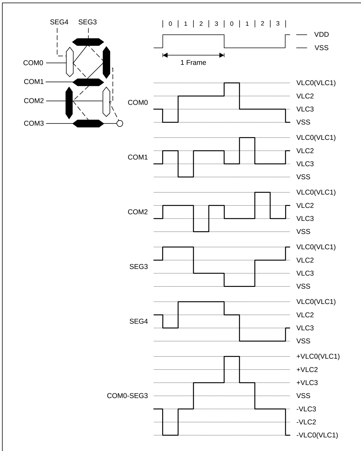
Figure 12.56 LCD Signal Waveforms (1/4Duty, 1/3Bias)
