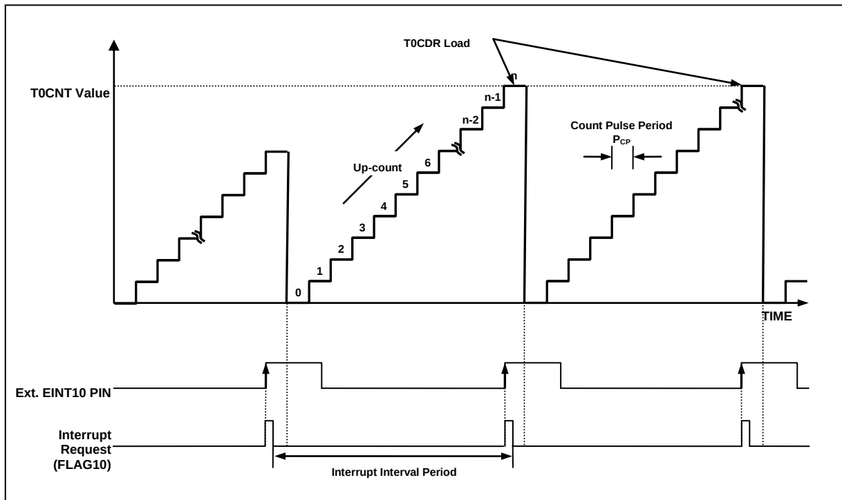
Figure 12.11 Input Capture Mode Operation for Timer 0
