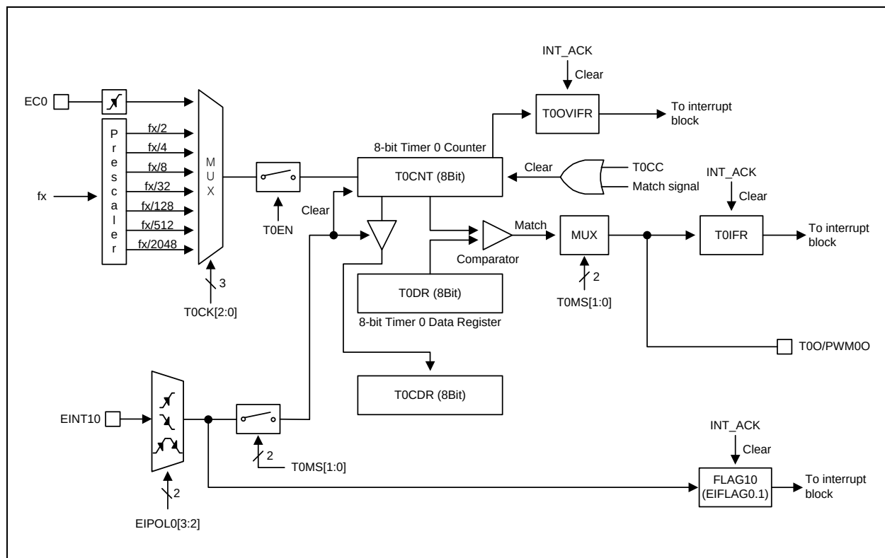
Figure 12.13 8-Bit Timer 0 Block Diagram
