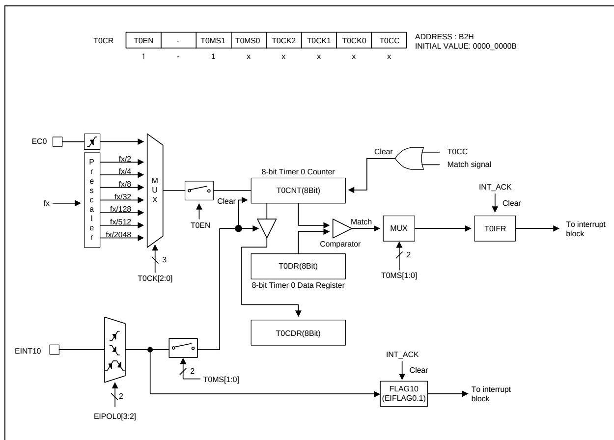
Figure 12.10 8-Bit Capture Mode for Timer 0
