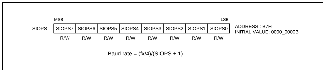
Figure 12.38 SIO Pre-Scaler Register (SIOPS)
