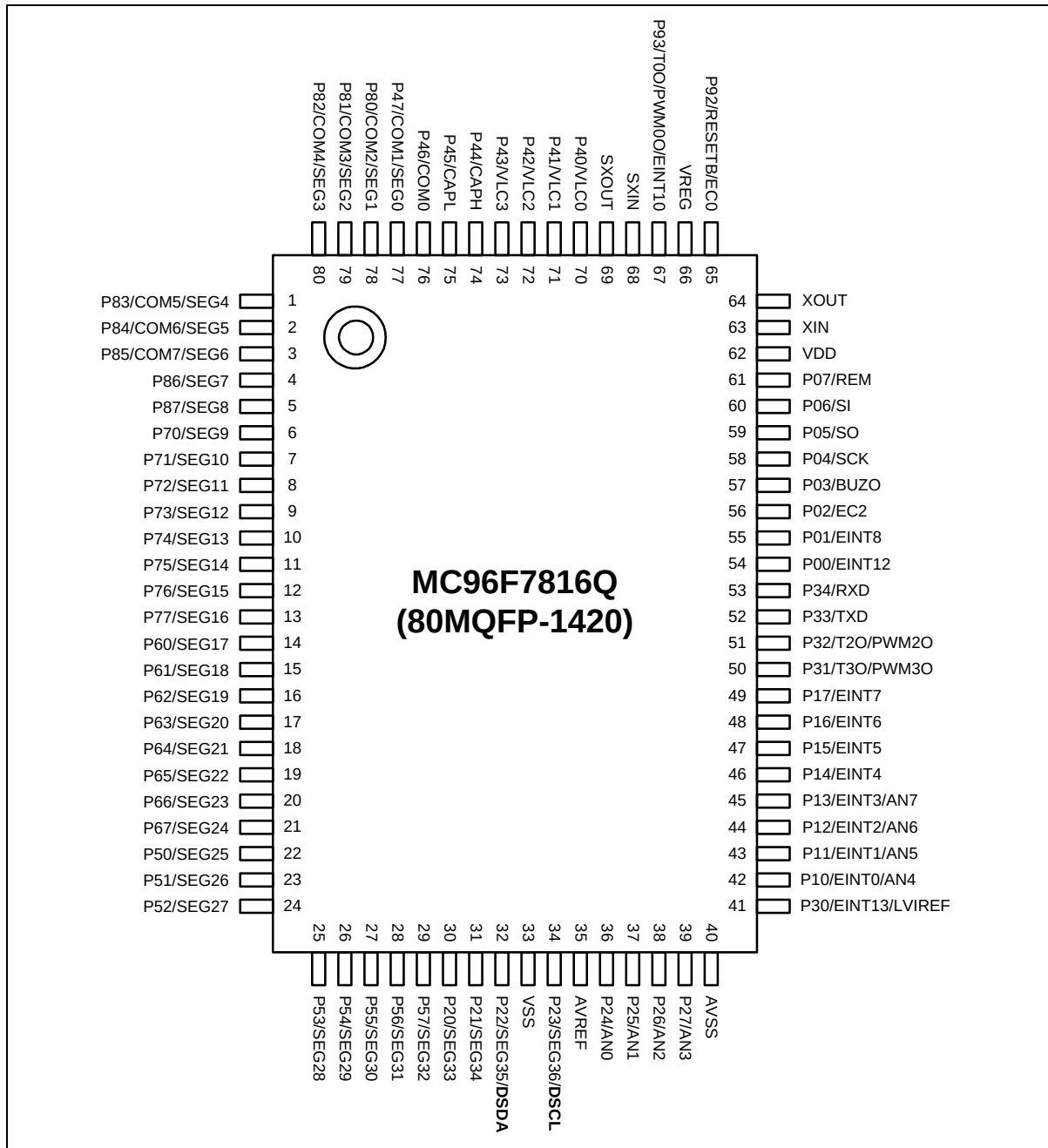
Figure 3.1 MC96F7816 80MQFP-1420 Pin Assignment
