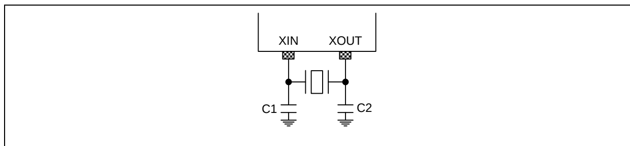
Figure 8.9 Crystal/Ceramic Oscillator
