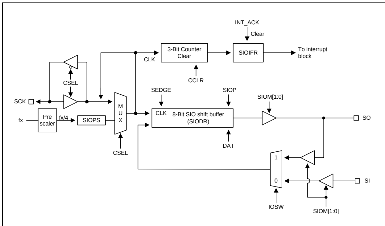
Figure 12.37 SIO Block Diagram
