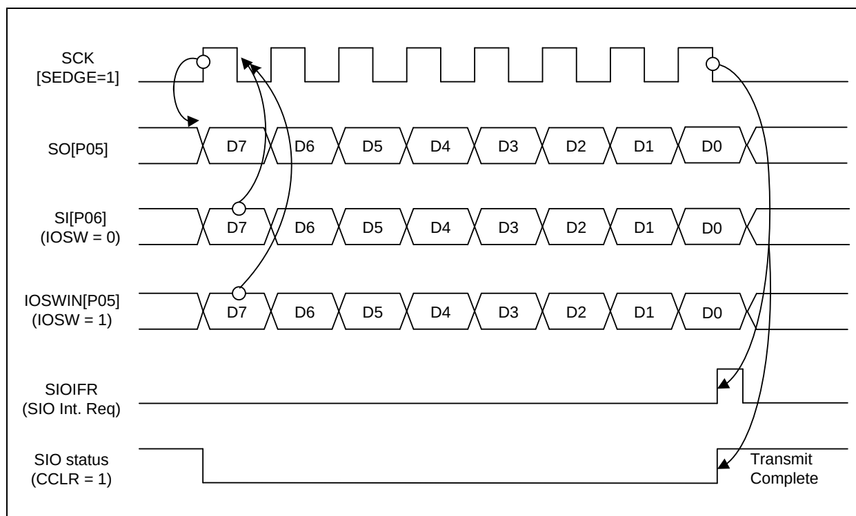
Figure 12.40 SIO Timing Diagram at SEDGE=1
