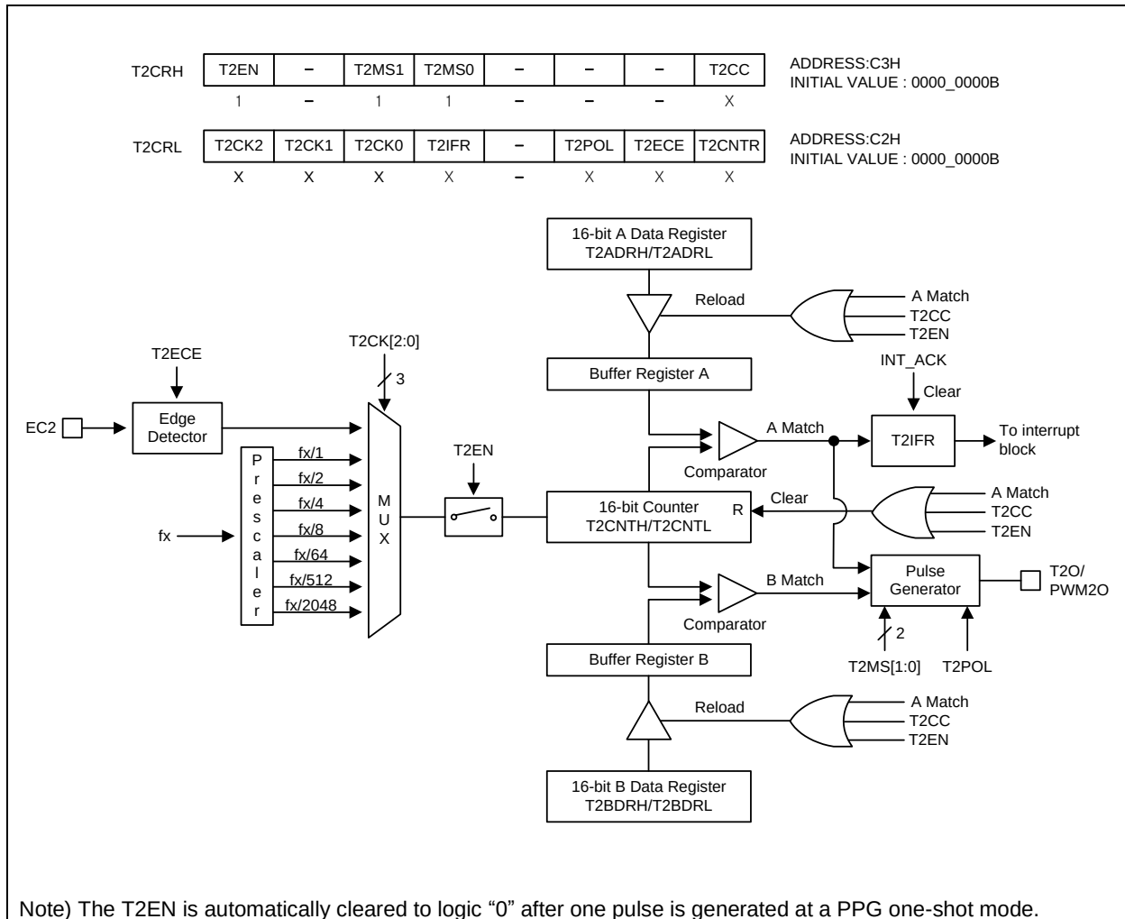
Figure 12.25 16-Bit PPG Mode for Timer 2
