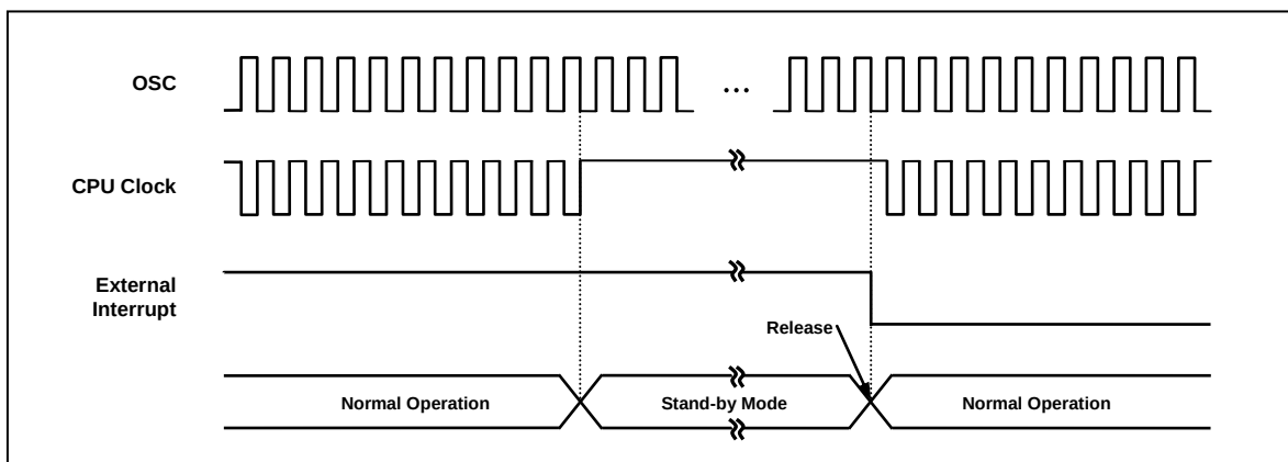
Figure 13.1 IDLE Mode Release Timing by External Interrupt
