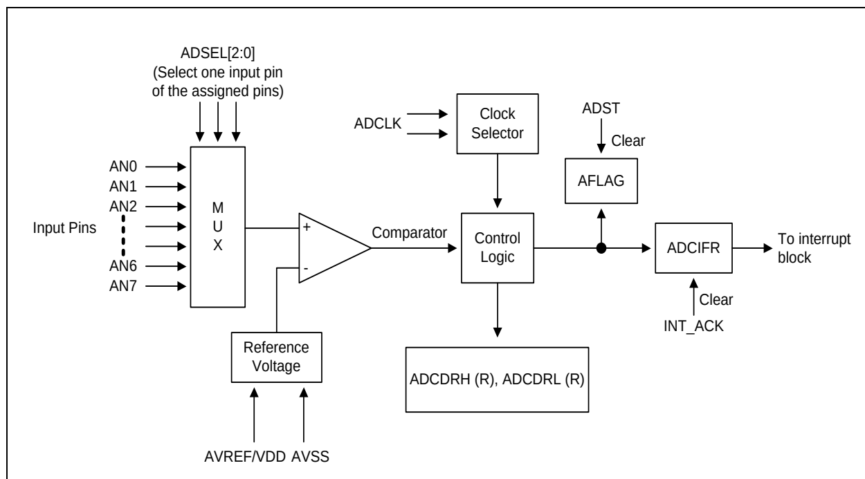
Figure 12.41 12-bit ADC Block Diagram
