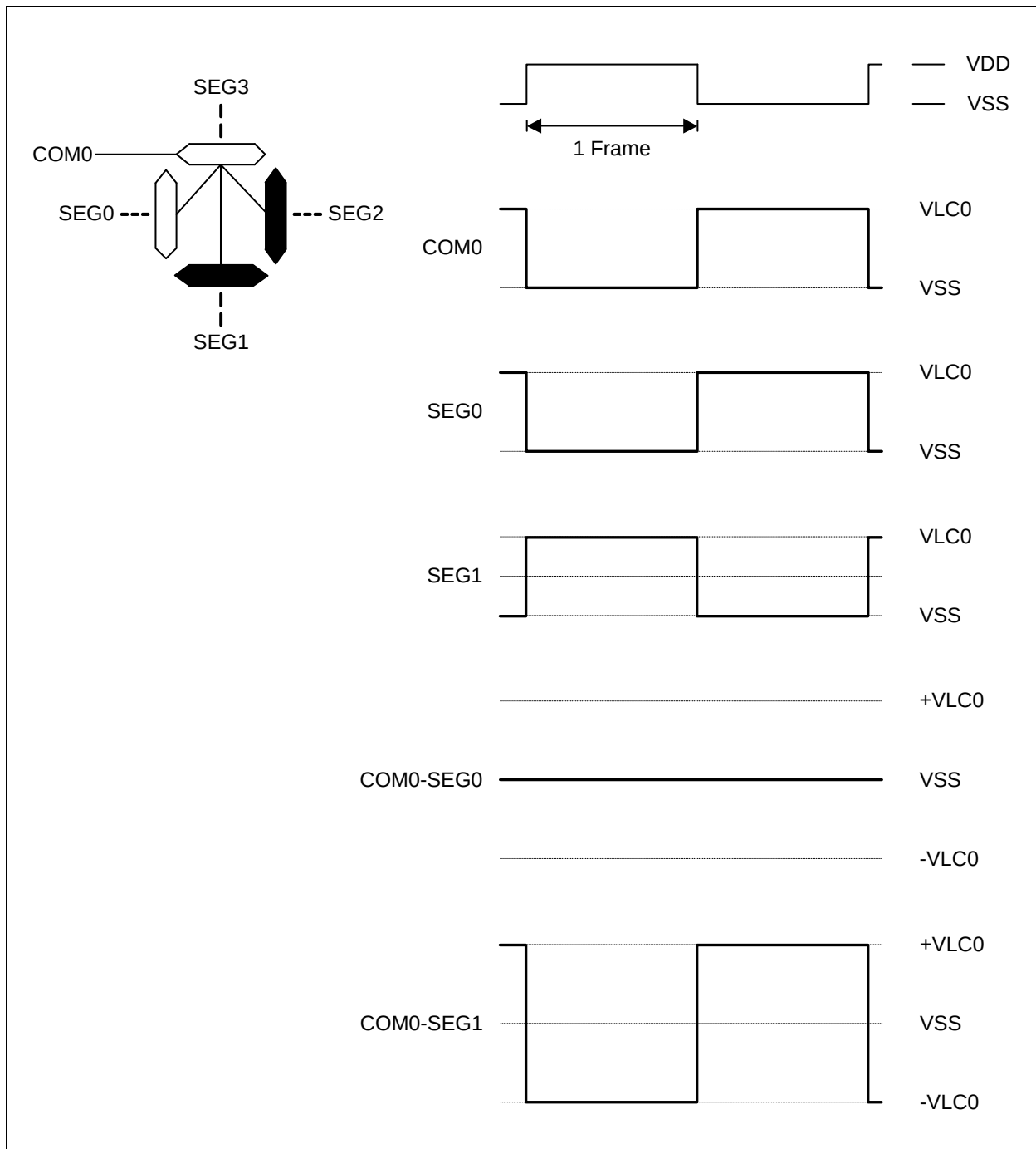
Figure 12.53 LCD Signal Waveforms (Static)
