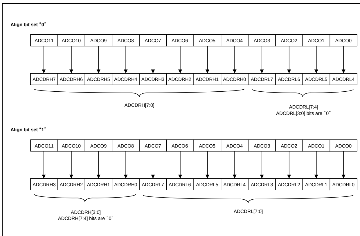
Figure 12.44 ADC Operation for Align Bit
