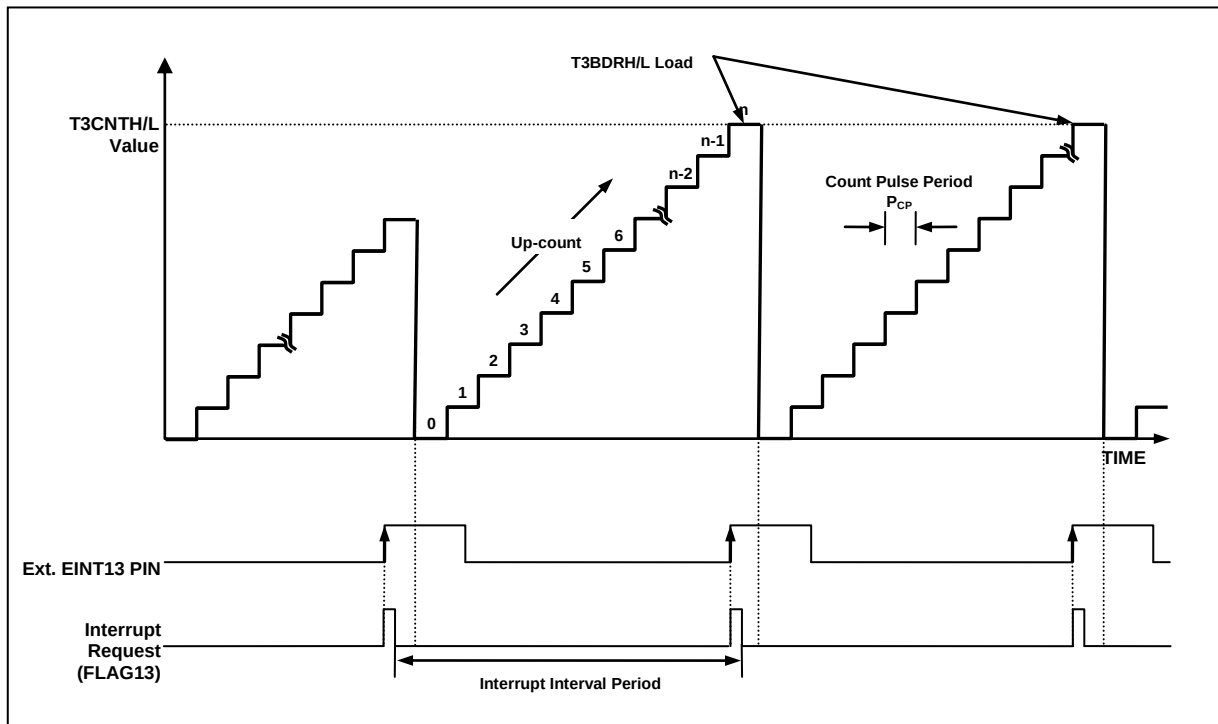
Figure 12.31 Input Capture Mode Operation for Timer 3
