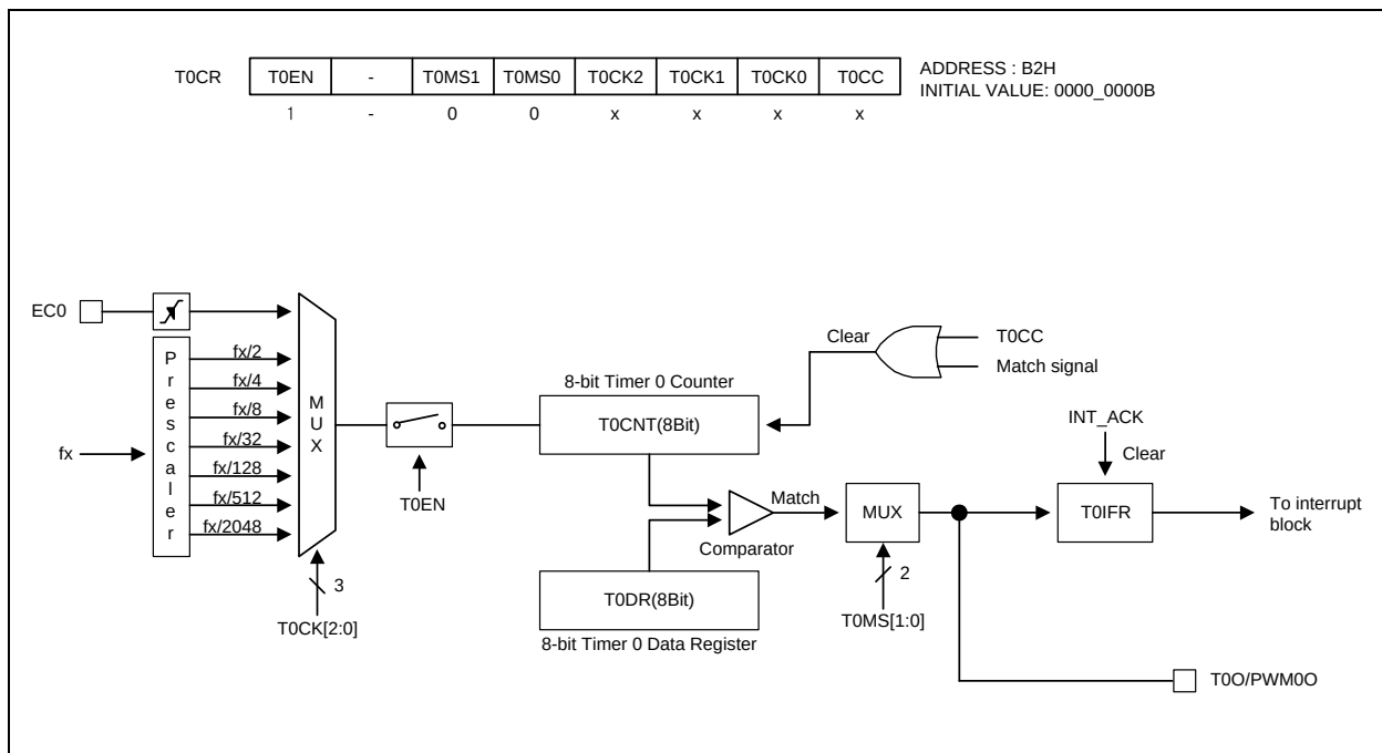
Figure 12.6 8-Bit Timer/Counter Mode for Timer 0
