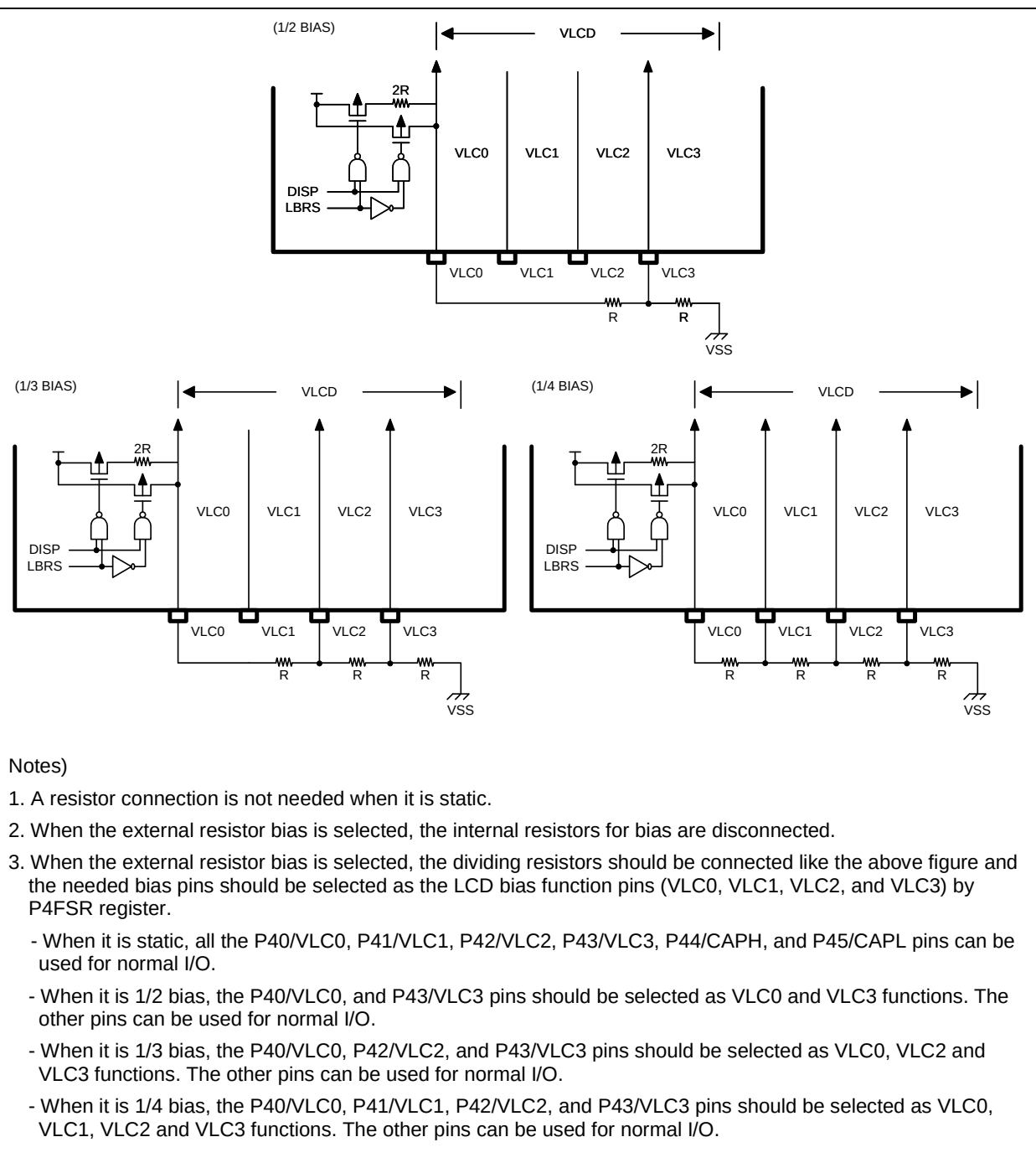
Figure 12.59 External Resistor Bias Connection
