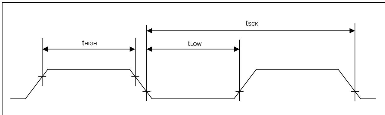
Figure 8.5 Waveform for UART Timing Characteristics
