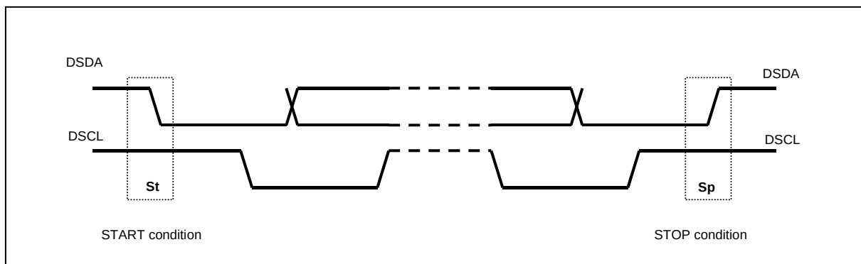
Figure 15.5 Start and Stop Condition
