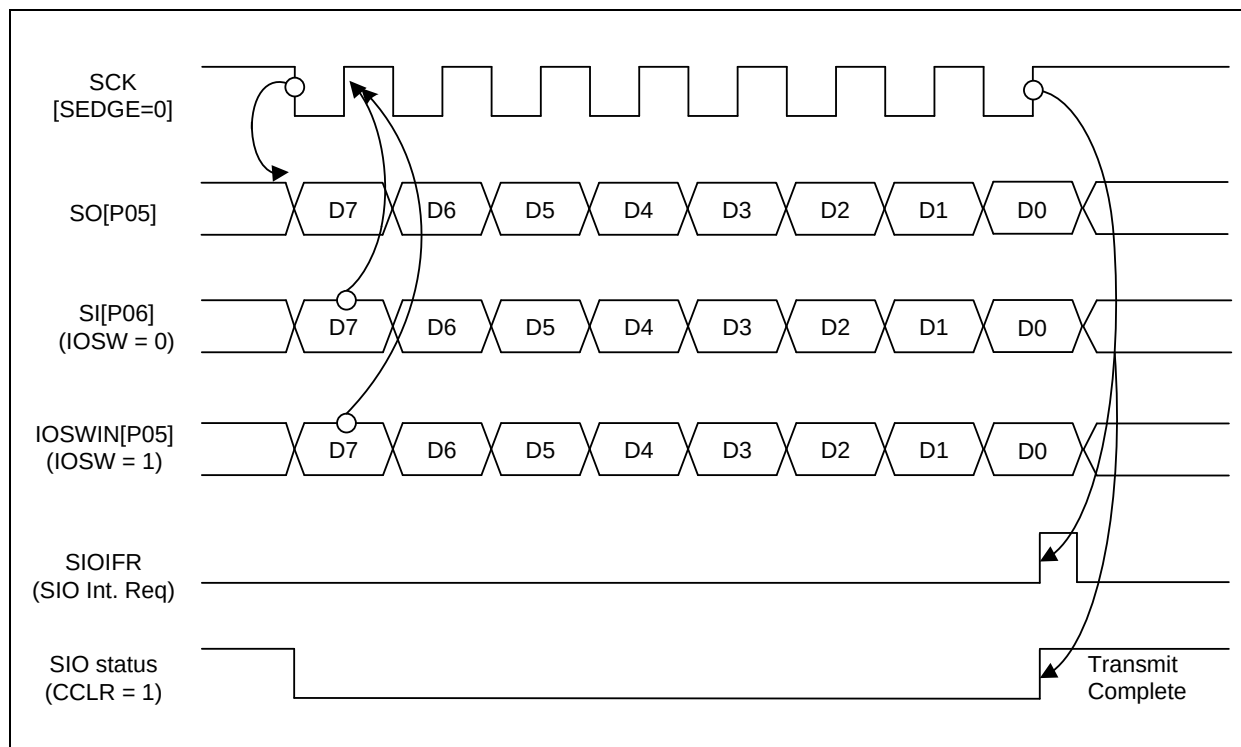
Figure 12.39 SIO Timing Diagram at SEDGE=0
