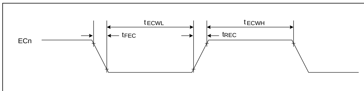
Figure 8.3 Input Timing for EC0, EC2
