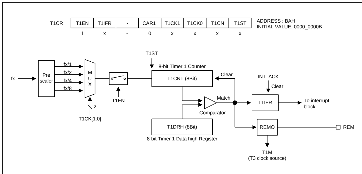
Figure 12.14 8-Bit Timer/Counter Mode for Timer 1
