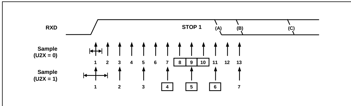
Figure 12.51 Stop Bit Sampling and Next Start Bit Sampling
