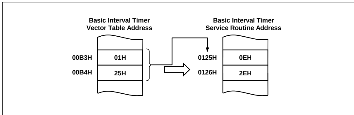
Figure 11.8 Correspondence between Vector Table Address and the Entry Address of ISP
