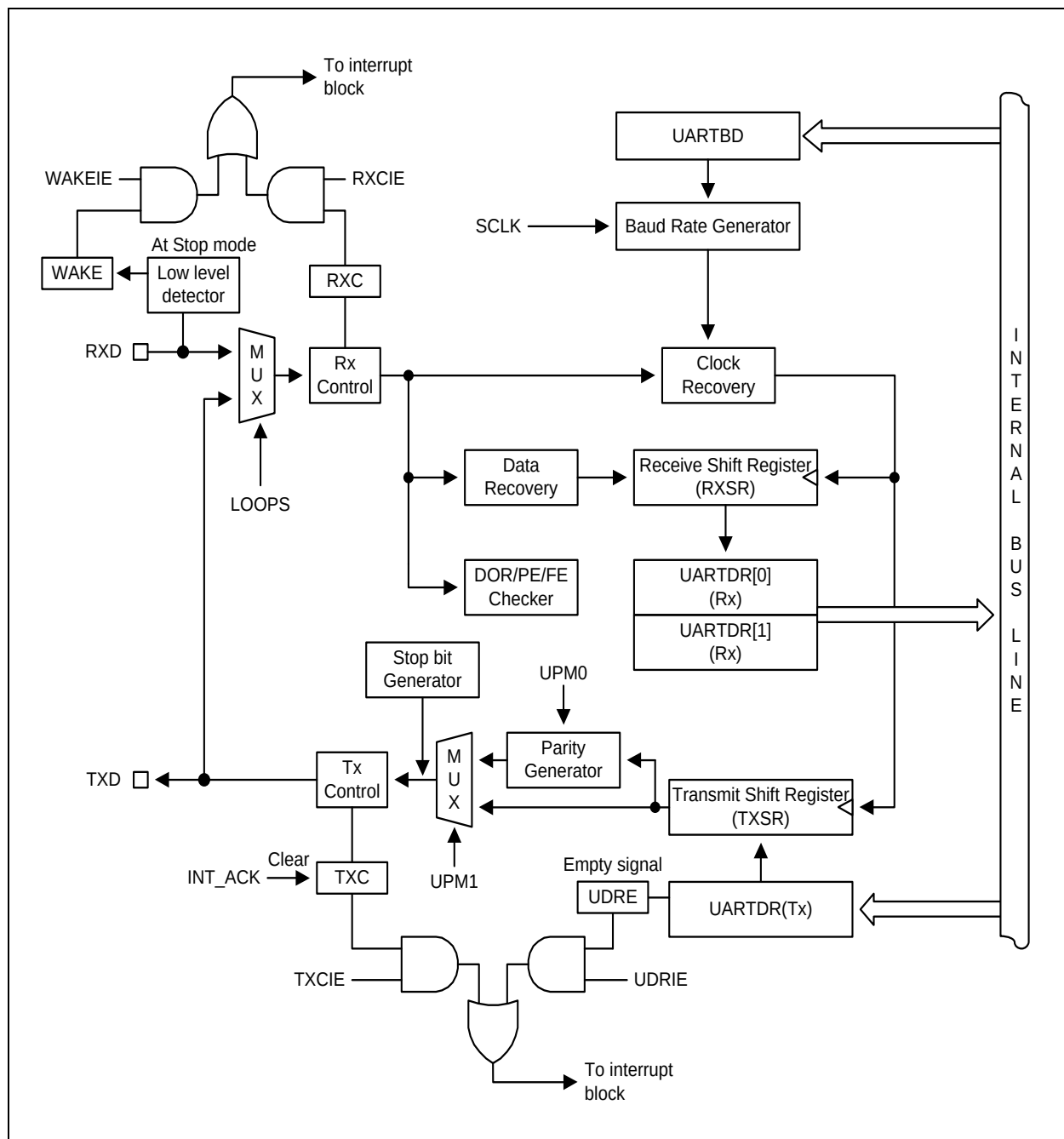
Figure 12.46 UART Block Diagram
