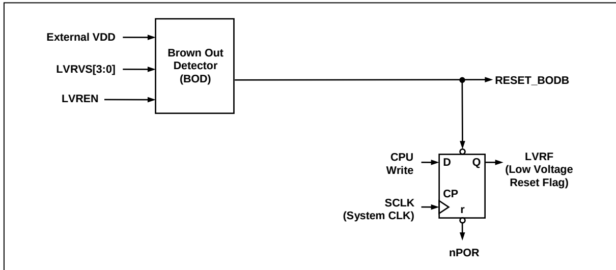
Figure 14.9 Block Diagram of BOD
