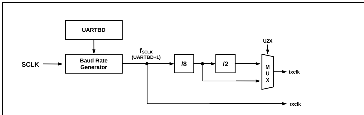
Figure 12.47 Clock Generation Block Diagram
