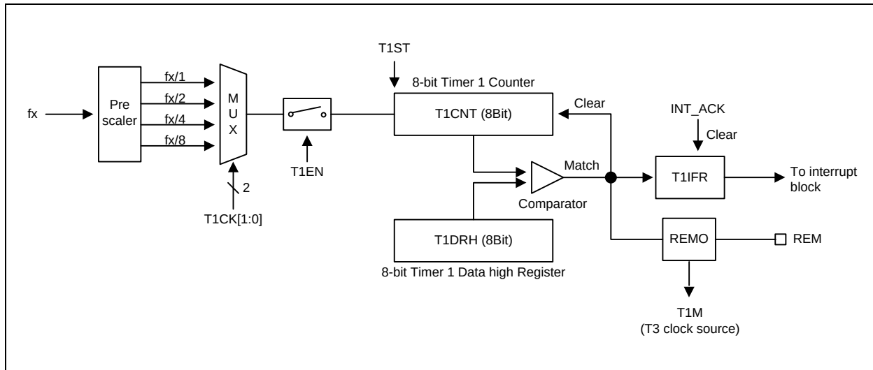
Figure 12.19 8-Bit Timer 1 Block Diagram
