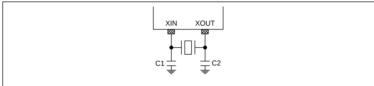
Figure 7.9 Crystal/Ceramic Oscillator
