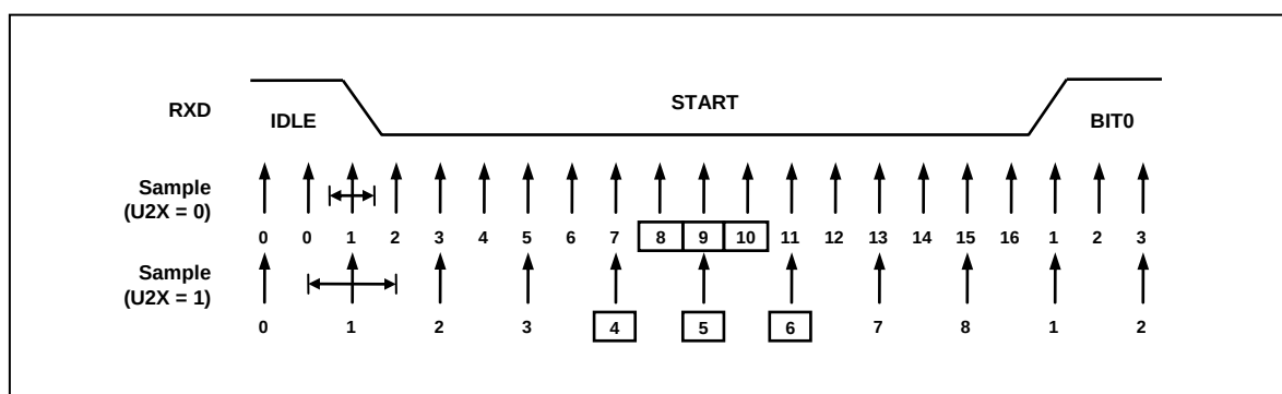
Figure 12.49 Start Bit Sampling
