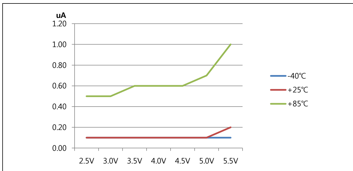
Figure 8.21 STOP (IDD5) Current
