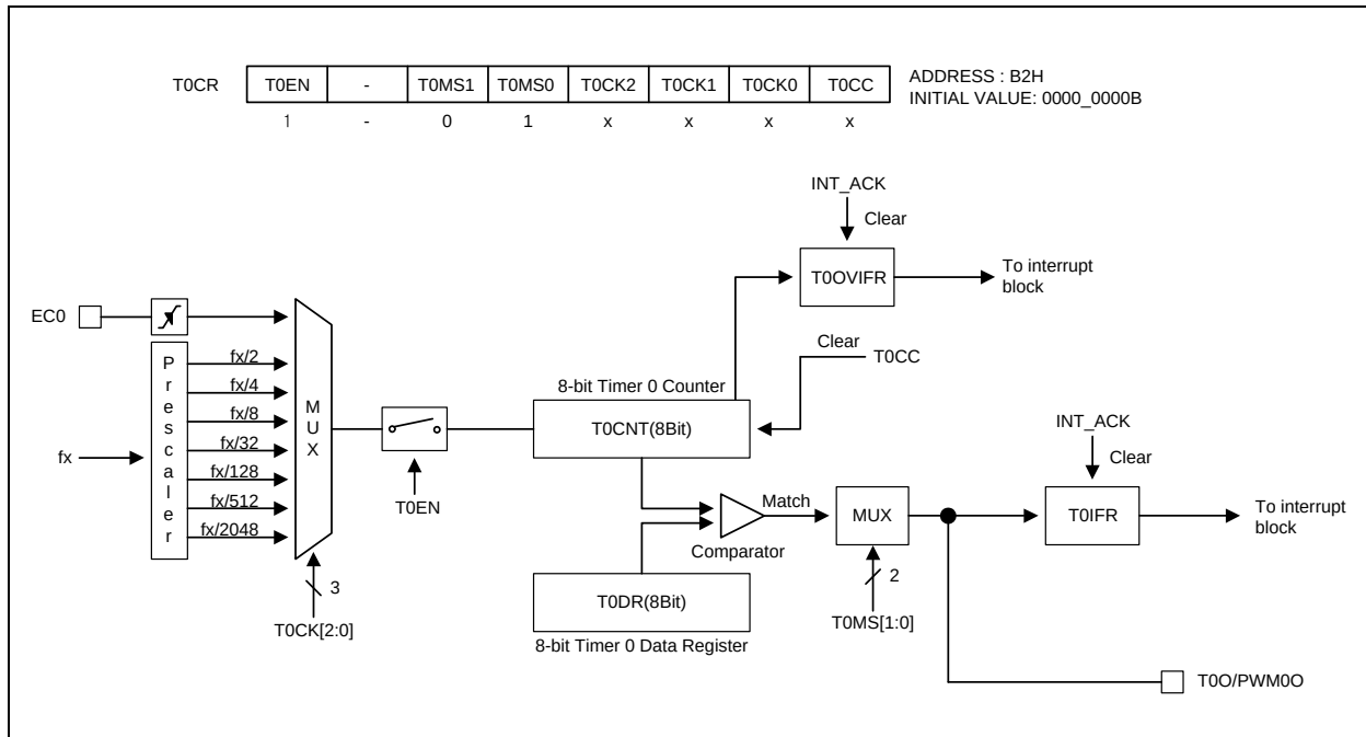
Figure 12.8 8-Bit PWM Mode for Timer 0
