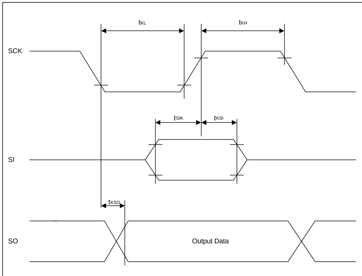
Figure 7.4 Serial Interface Data Transfer Timing
