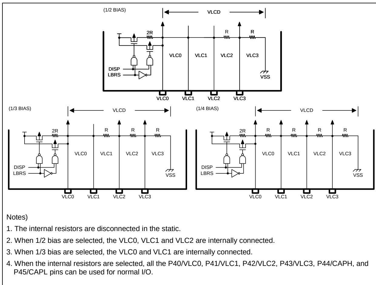
Figure 12.58 Internal Resistor Bias Connection
