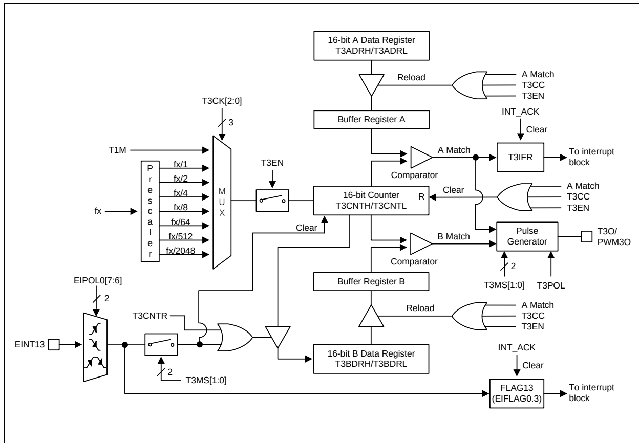
Figure 12.35 16-Bit Timer 3 Block Diagram
