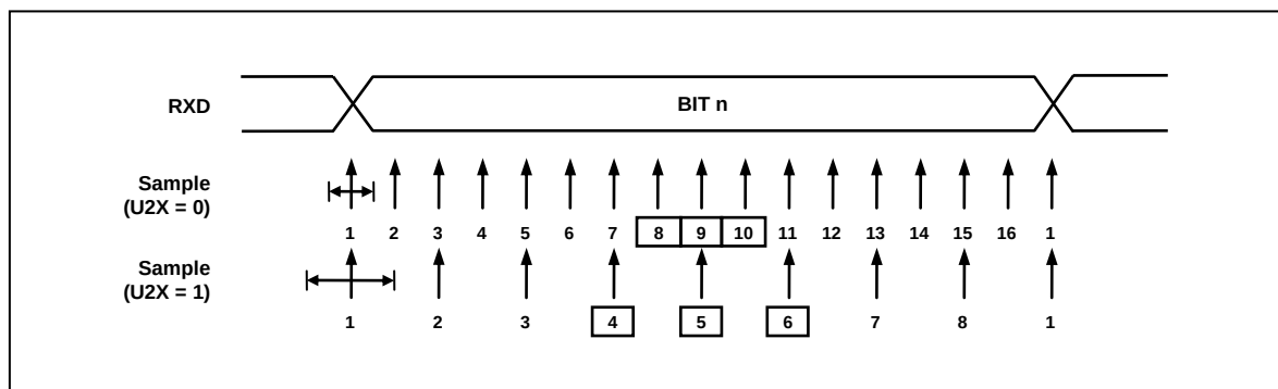
Figure 12.50 Sampling of Data and Parity Bit
