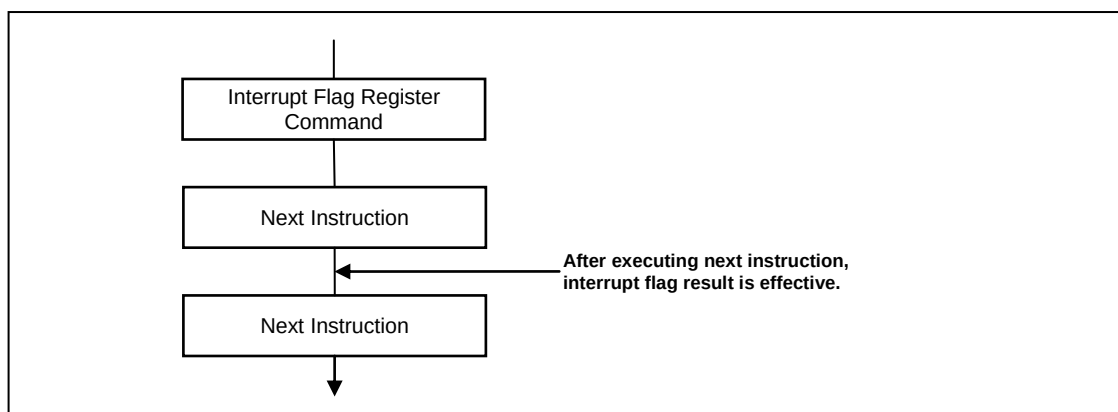
Figure 11.5 Effective Timing of Interrupt Flag Register
