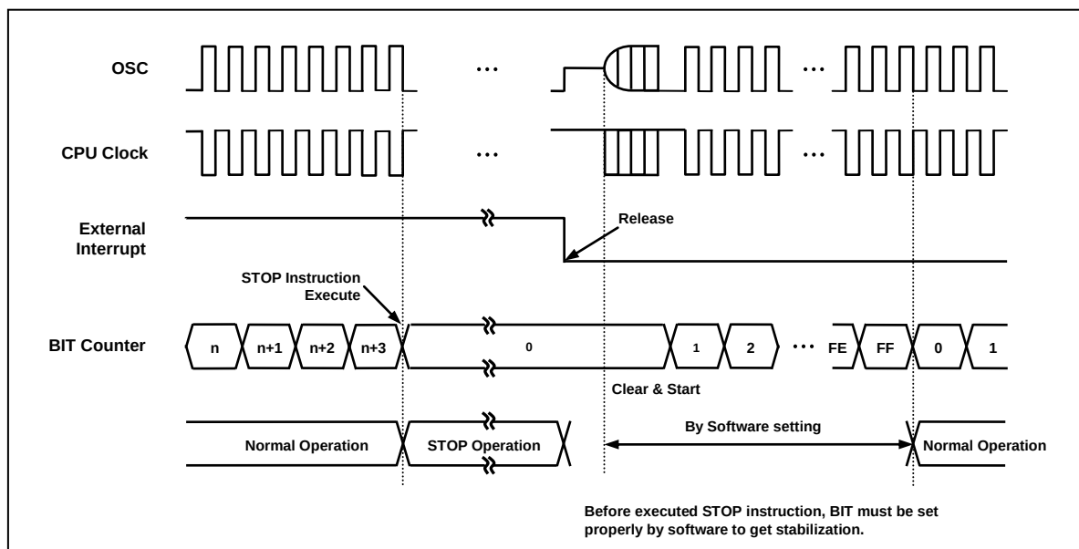
Figure 13.2 STOP Mode Release Timing by External Interrupt
