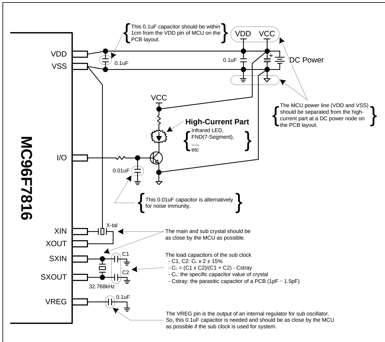
Figure 8.16 Recommended Circuit and Layout
