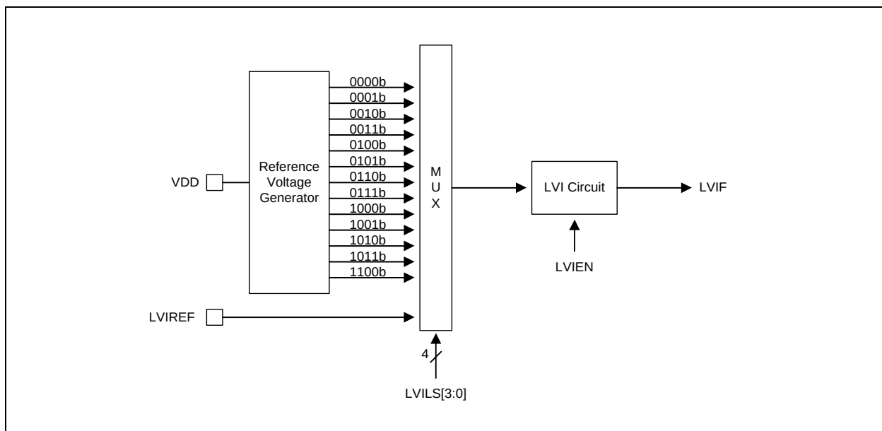
Figure 14.12 LVI Diagram
