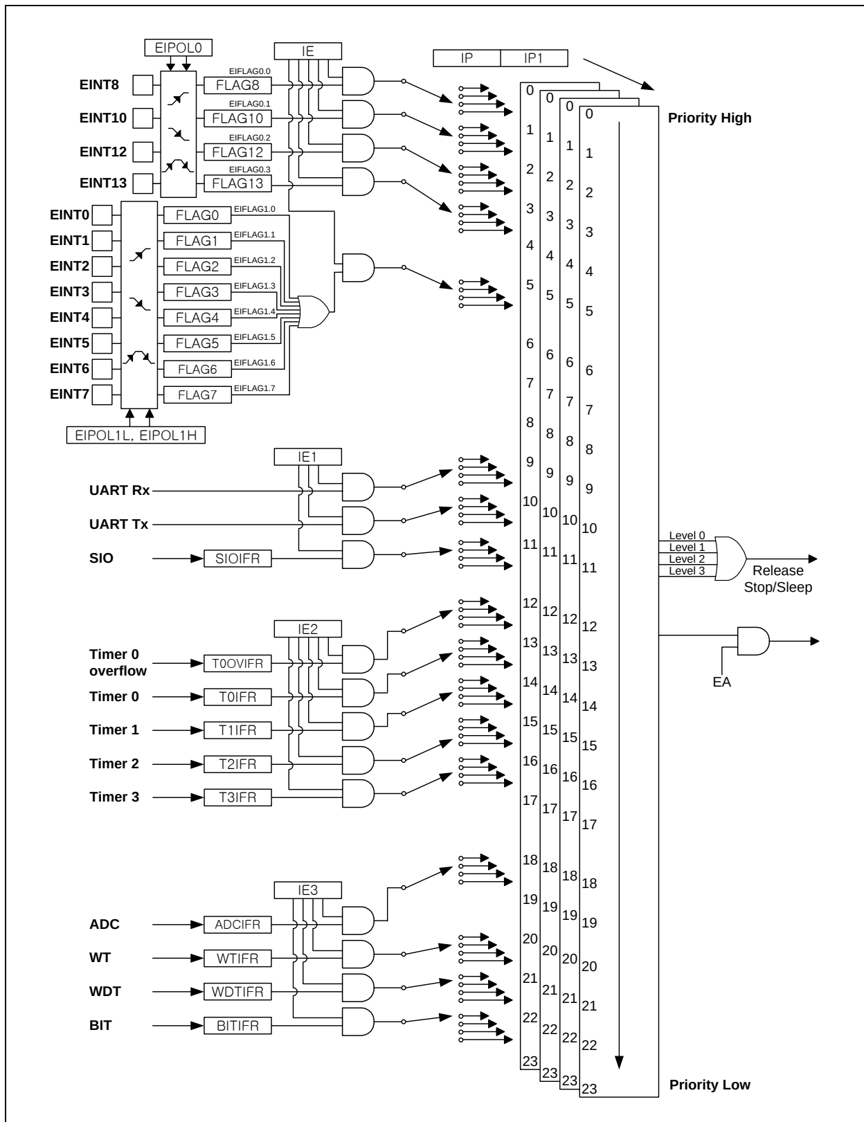
Figure 11.2 Block Diagram of Interrupt
