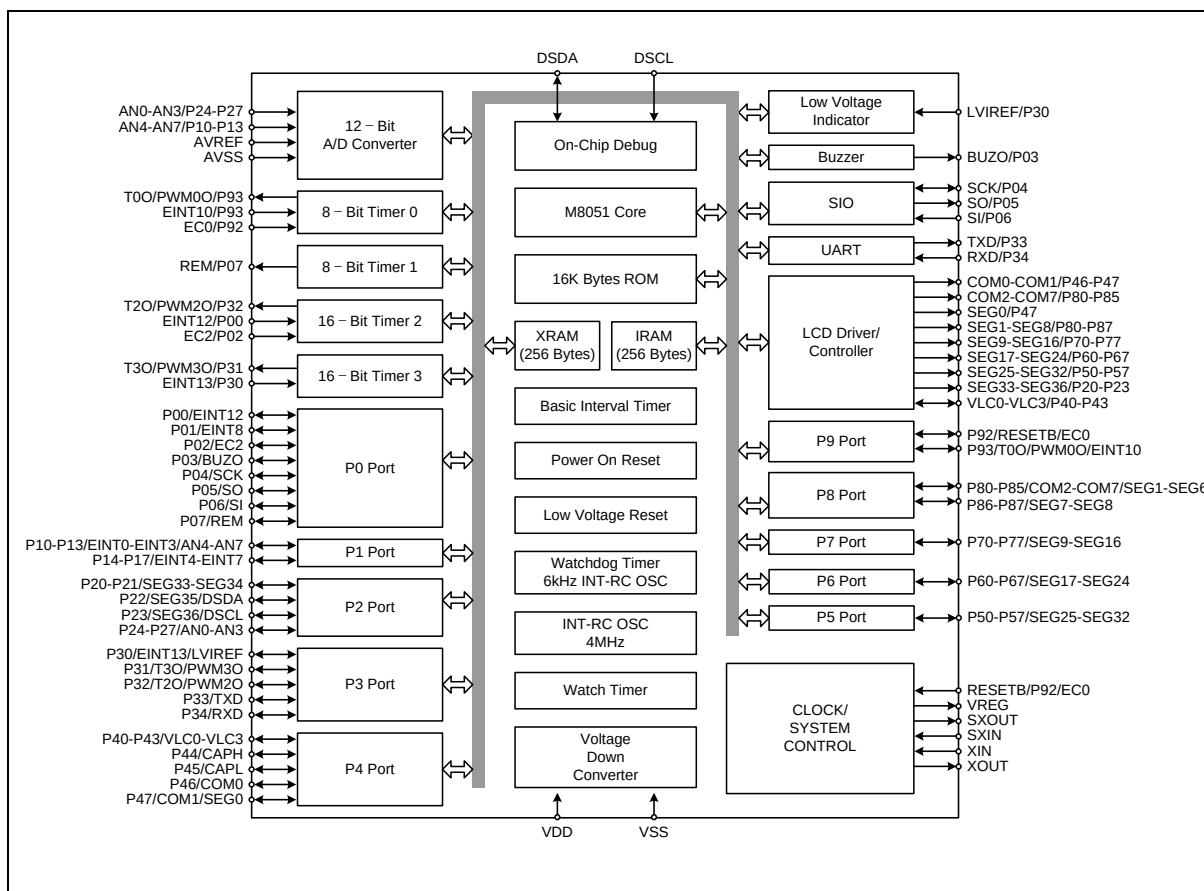
Figure 2.1 MC96F7816 Block Diagram
