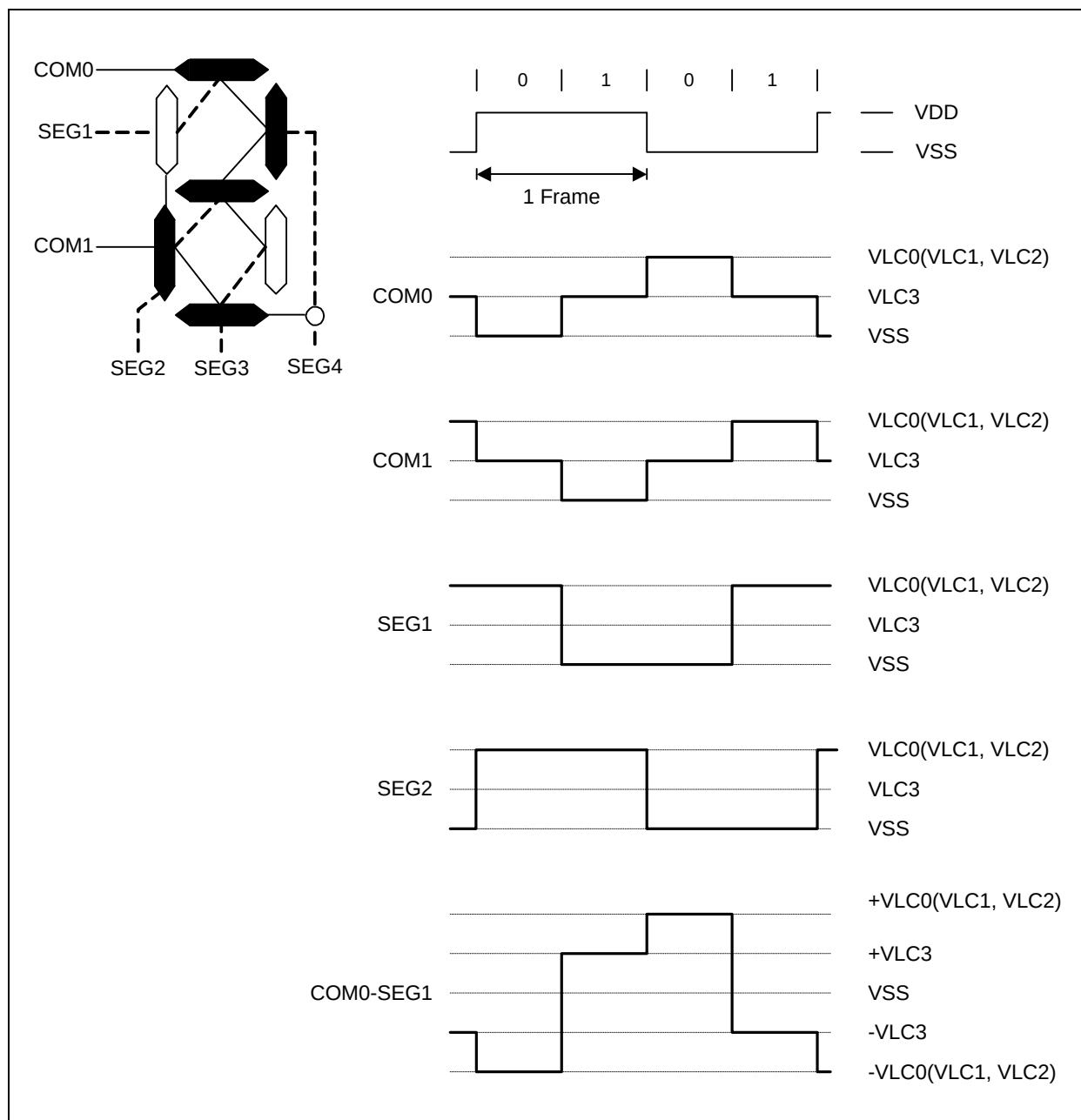
Figure 12.54 LCD Signal Waveforms (1/2Duty, 1/2Bias)
