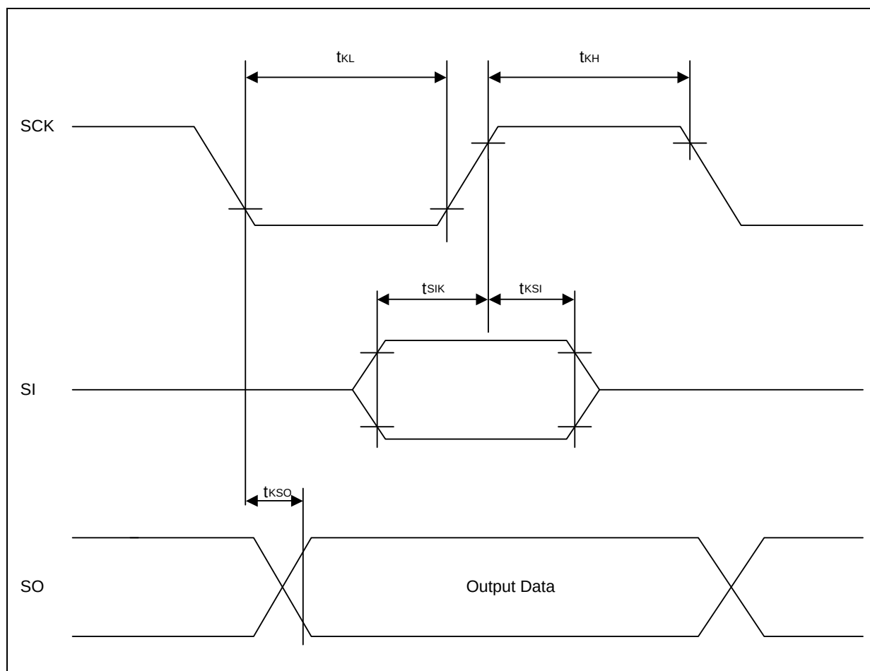
Figure 8.4 Serial Interface Data Transfer Timing
