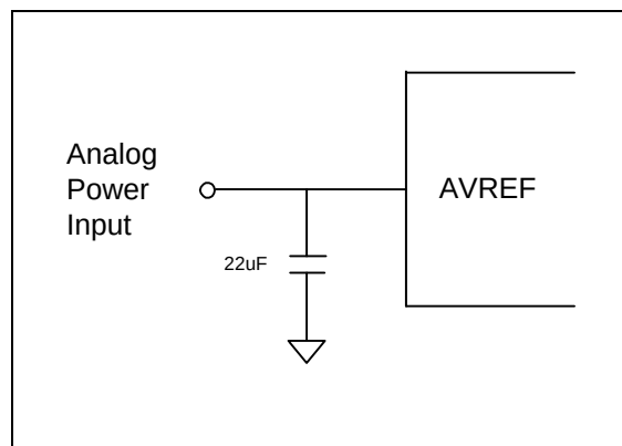
Figure 12.43 A/D Power (AVDD) Pin with Capacitor
