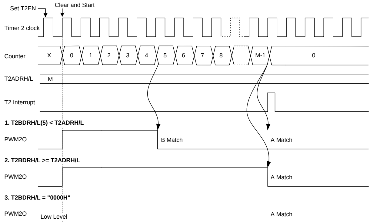
Figure 12.26 16-Bit PPG Mode Timing chart for Timer 2
