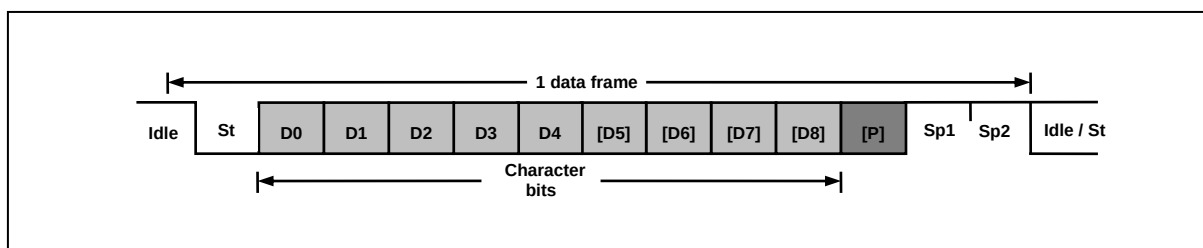
Figure 12.48 Frame Format
