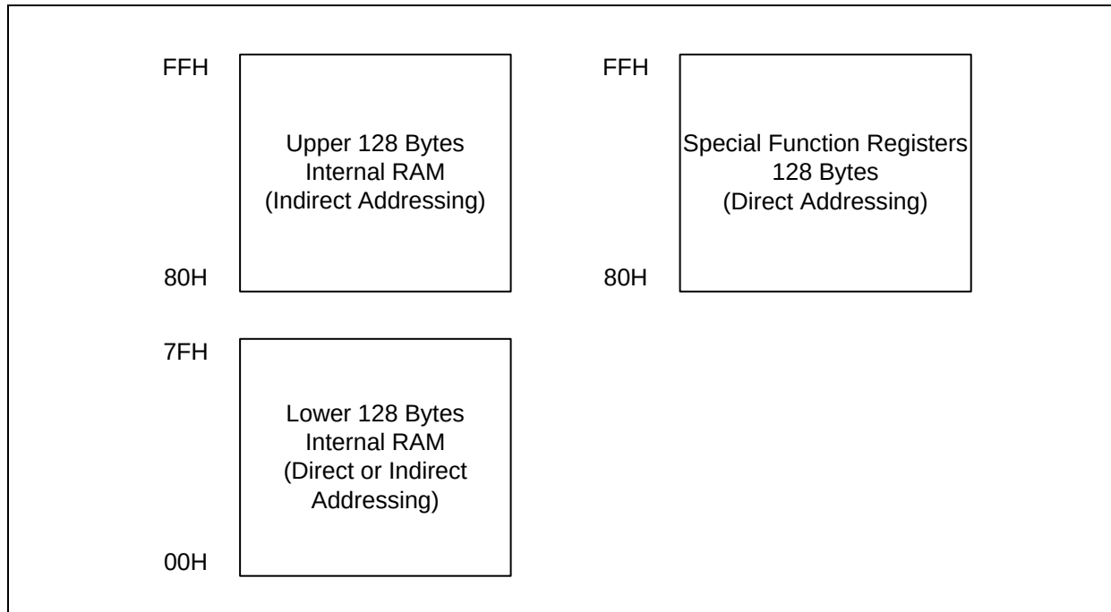
Figure 9.2 Data Memory Map
