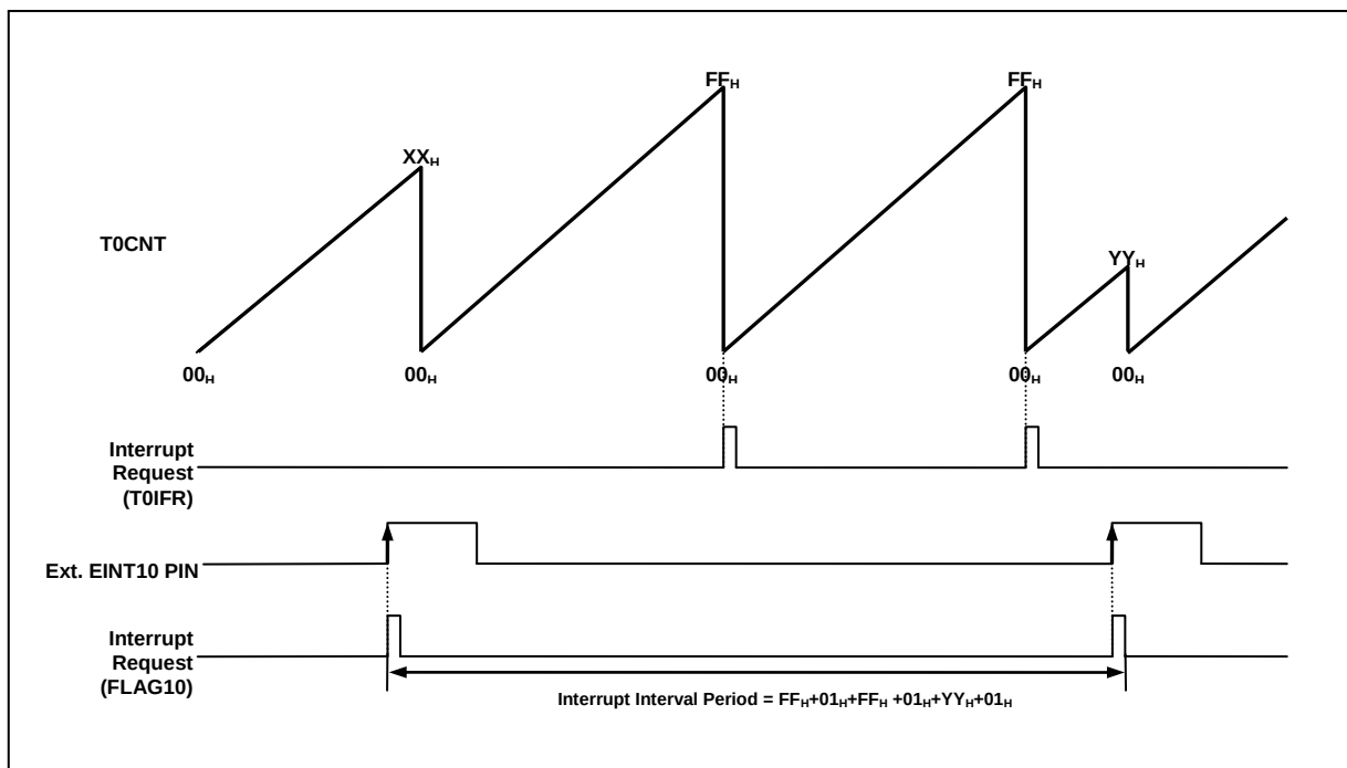
Figure 12.12 Express Timer Overflow in Capture Mode
