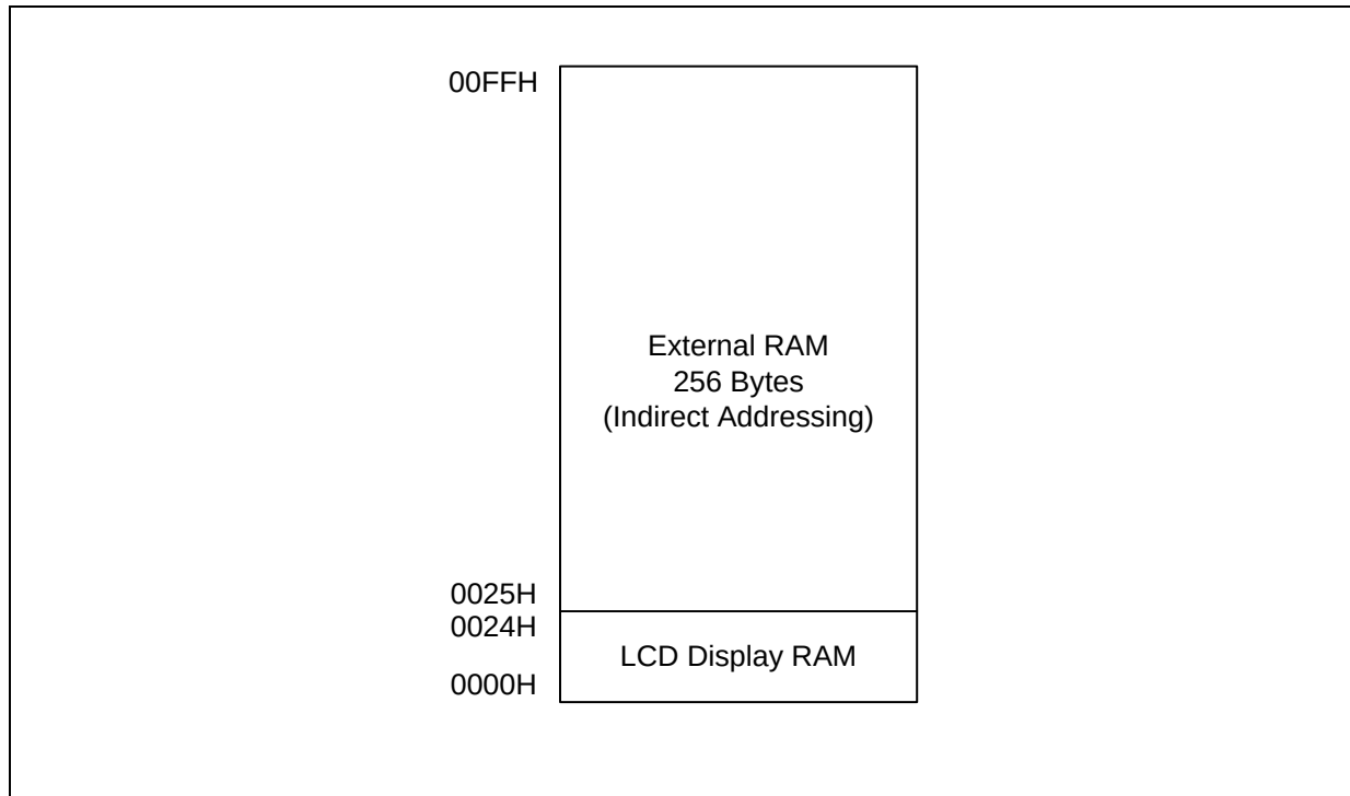
Figure 9.4 XDATA Memory Area
