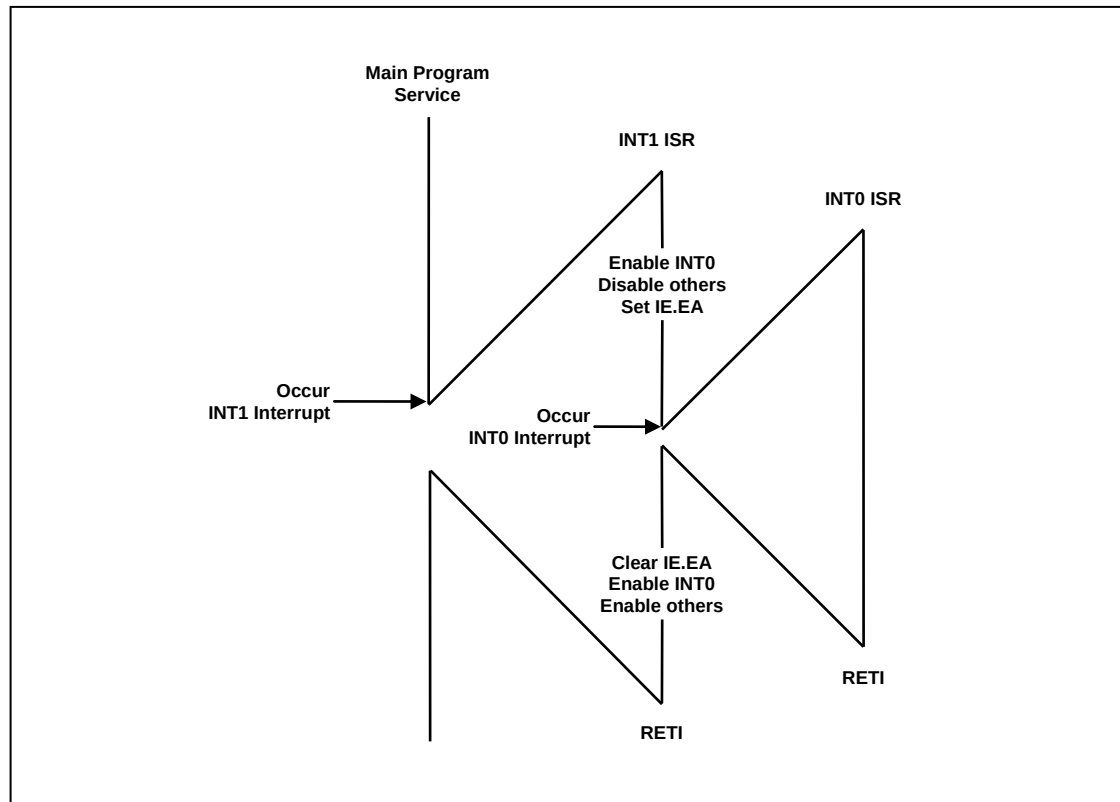
Figure 11.6 Effective Timing of Interrupt
