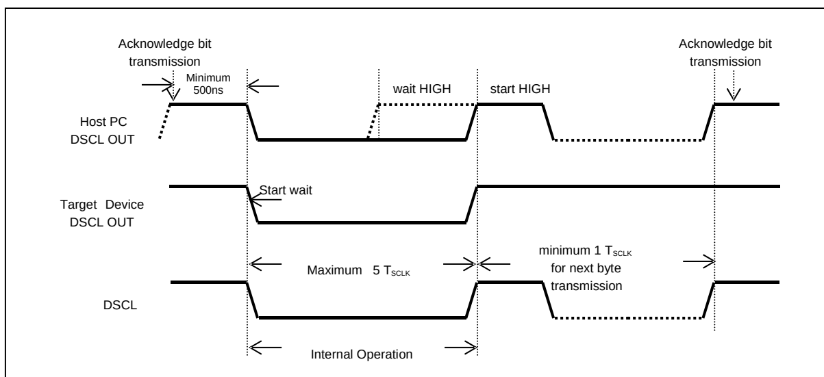
Figure 15.7 Clock Synchronization during Wait Procedure
