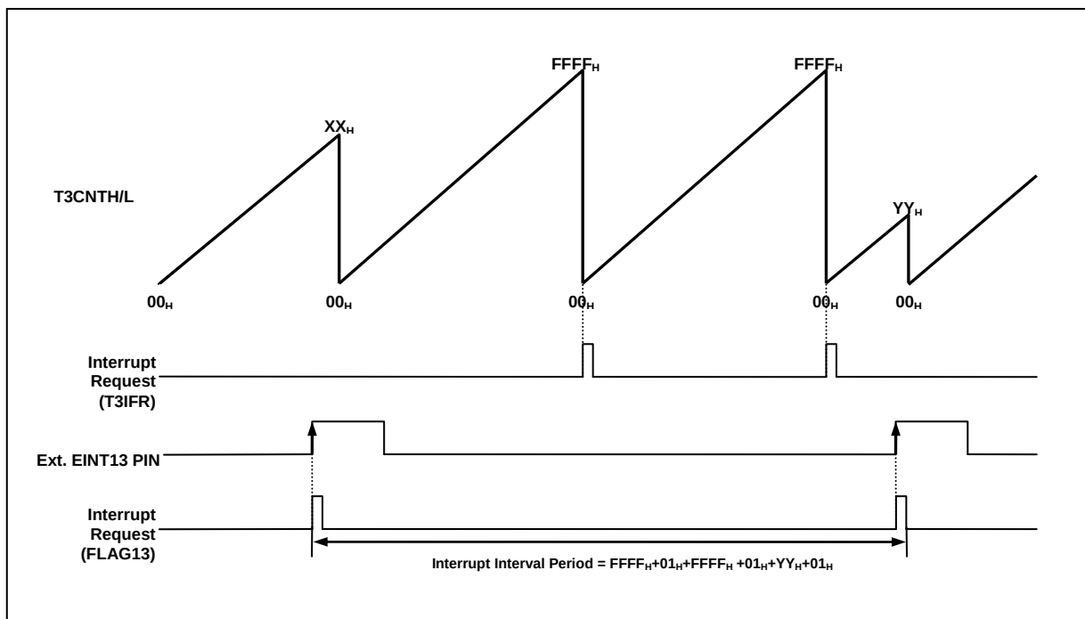
Figure 12.32 Express Timer Overflow in Capture Mode
