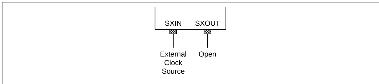
Figure 8.12 External Clock
