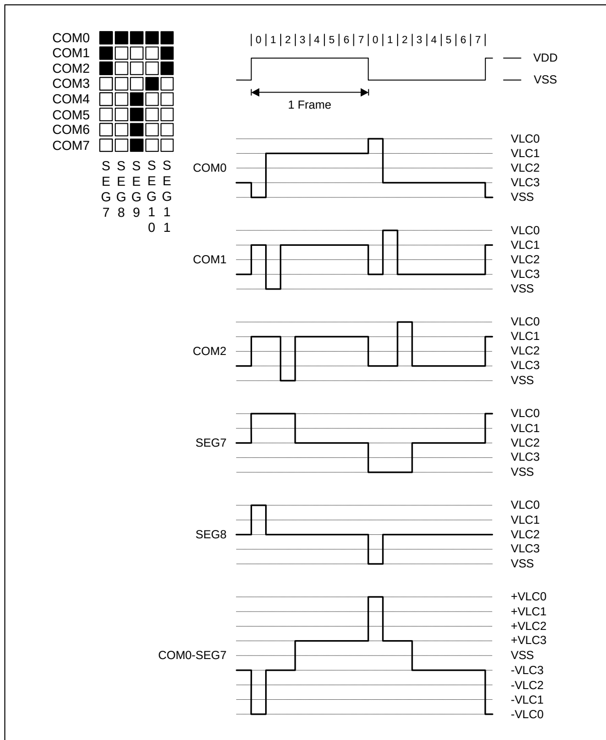
Figure 12.57 LCD Signal Waveforms (1/8Duty, 1/4Bias)
