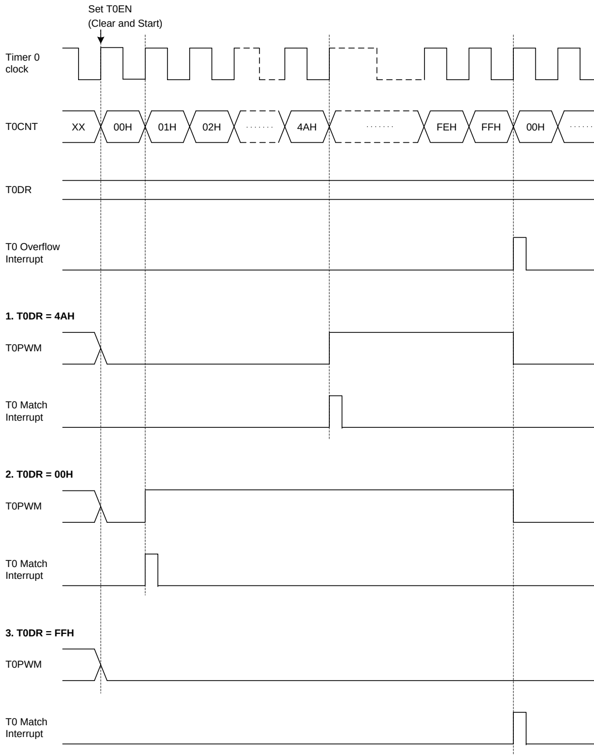
Figure 12.9 PWM Output Waveforms in PWM Mode for Timer 0
