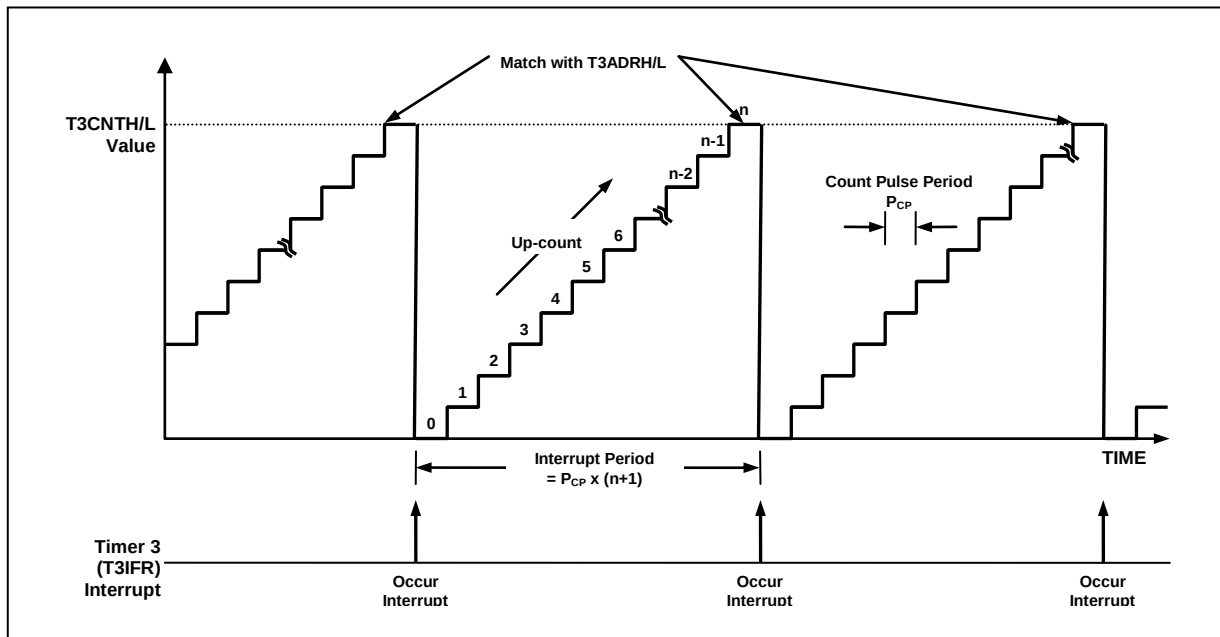
Figure 12.29 16-Bit Timer/Counter 3 Example
