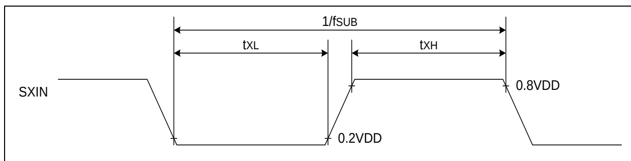
Figure 8.14 Clock Timing Measurement at SXIN
