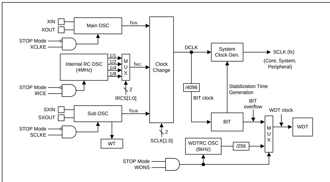
Figure 12.1 Clock Generator Block Diagram
