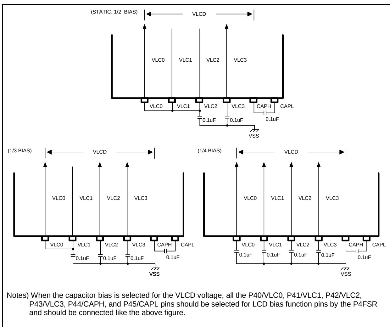
Figure 12.60 Capacitor Bias Connection
