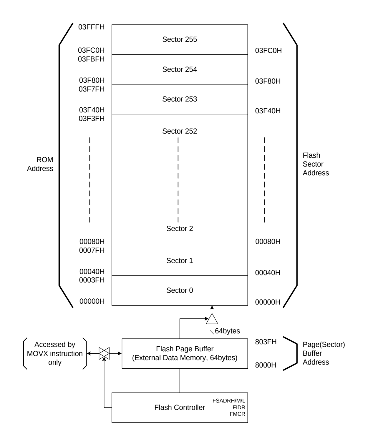
Figure 16.1 Flash Program ROM Structure
