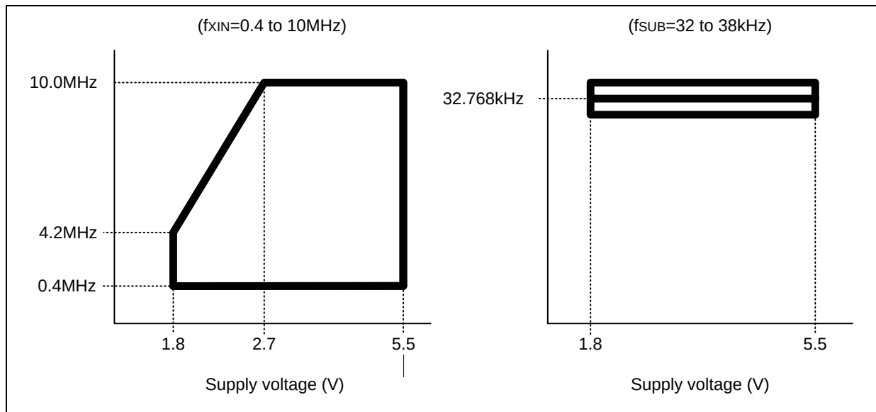
Figure 8.15 Operating Voltage Range
