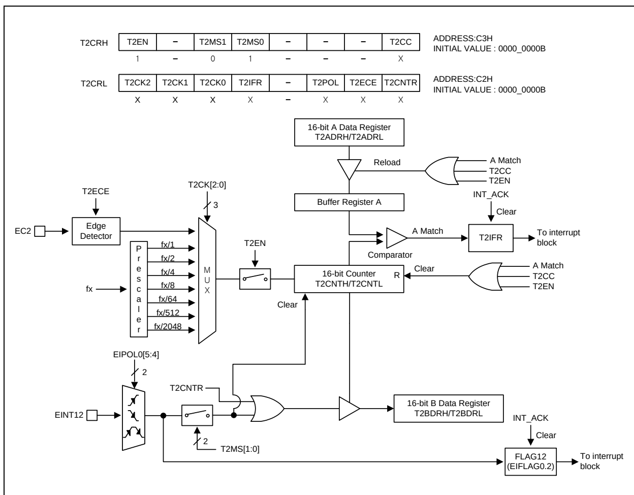
Figure 12.22 16-Bit Capture Mode for Timer 2
