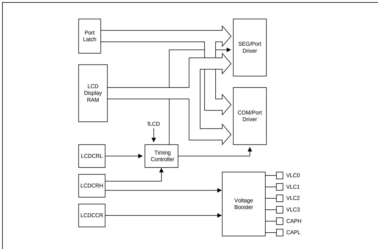
Figure 12.61 LCD Circuit Block Diagram
