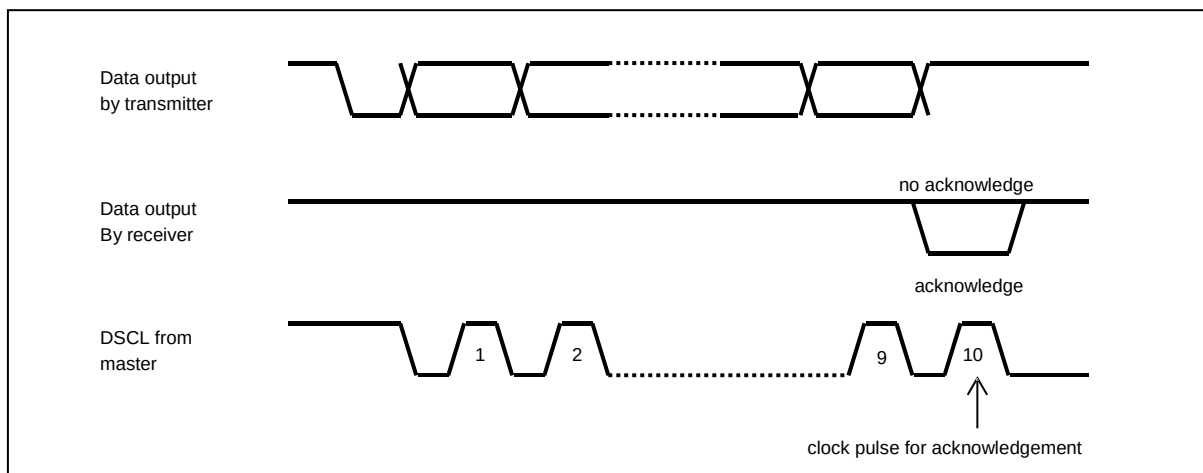
Figure 15.6 Acknowledge on the Serial Bus
