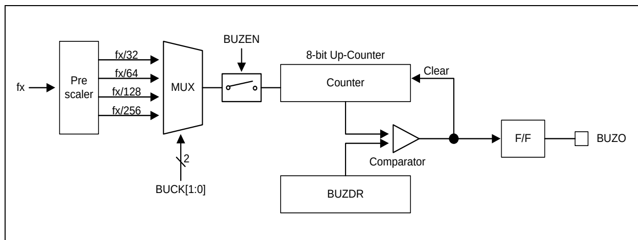
Figure 12.36 Buzzer Driver Block Diagram
