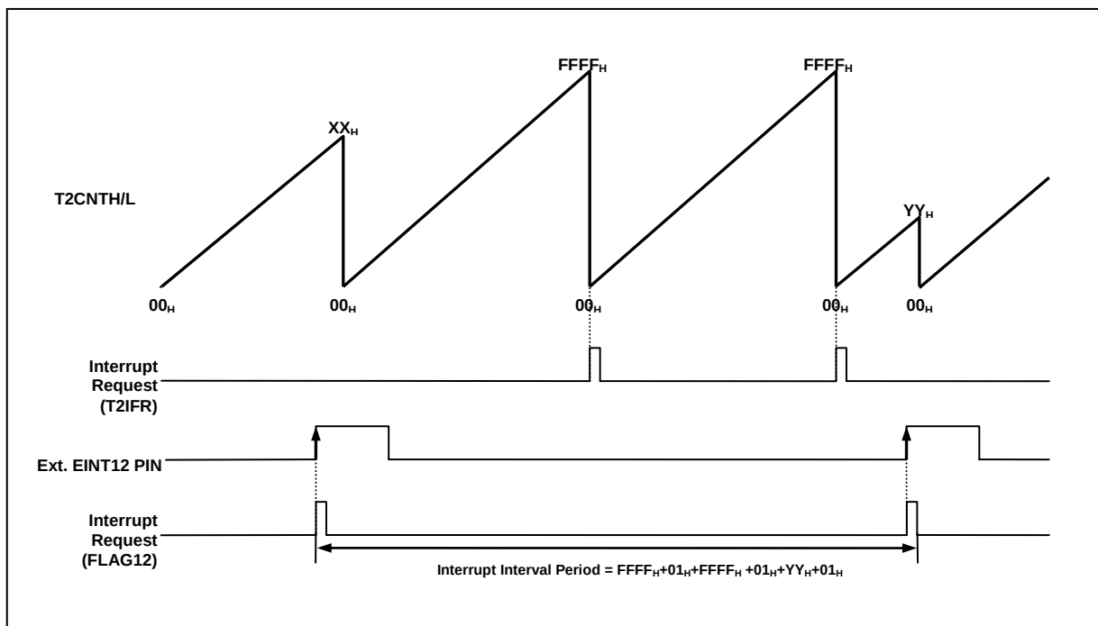
Figure 12.24 Express Timer Overflow in Capture Mode
