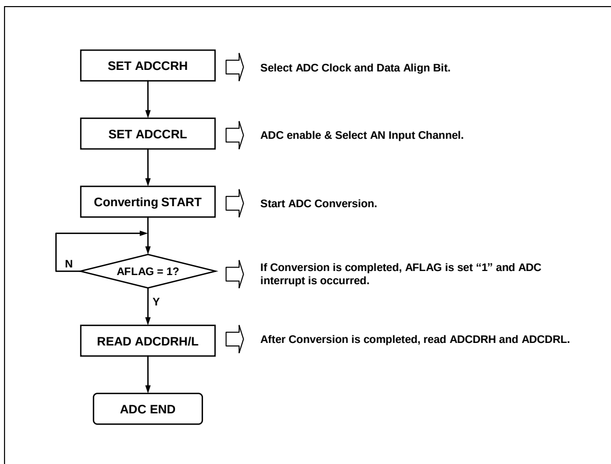
Figure 12.45 A/D Converter Operation Flow
