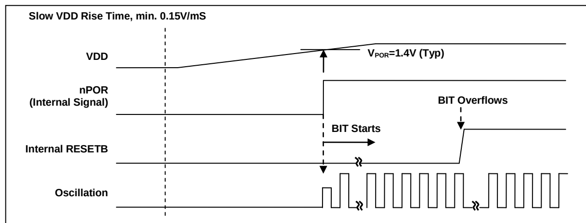
Figure 14.4 Internal RESET Release Timing On Power-Up
