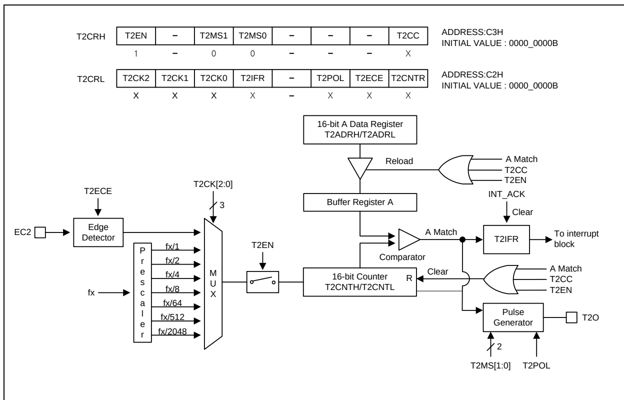
Figure 12.20 16-Bit Timer/Counter Mode for Timer 2
