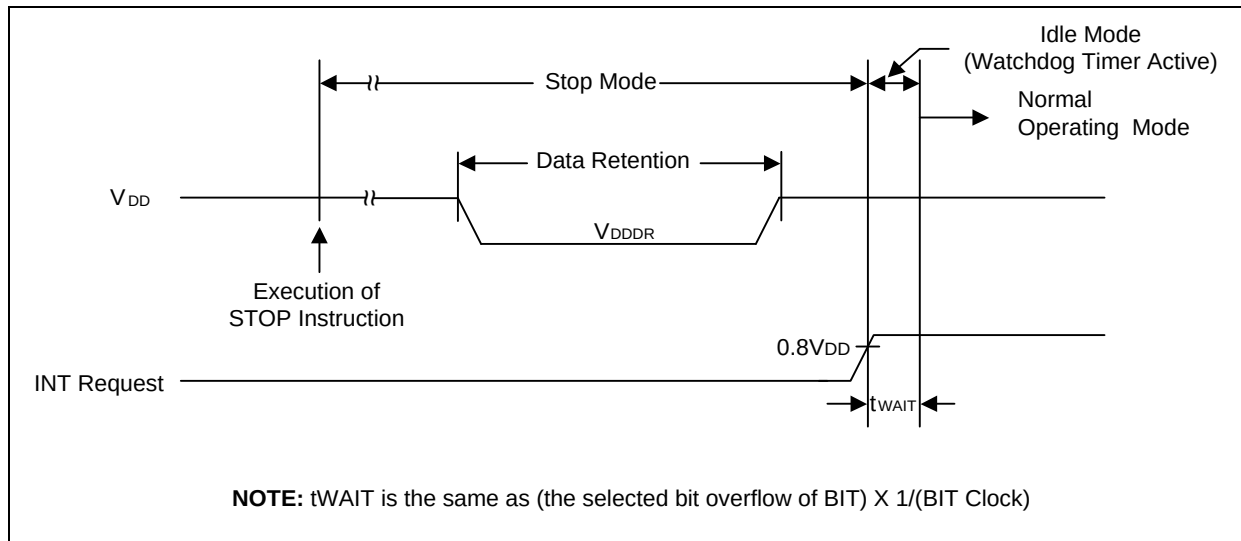
Figure 8.7 Stop Mode Release Timing when Initiated by an Interrupt
