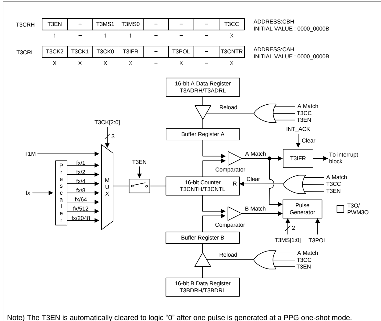
Figure 12.33 16-Bit PPG Mode for Timer 3
