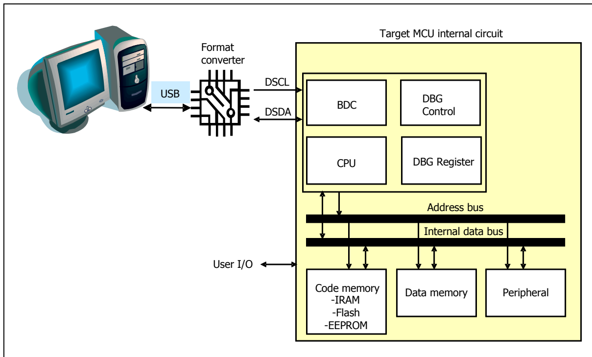
Figure 15.1 Block Diagram of On-Chip Debug System
