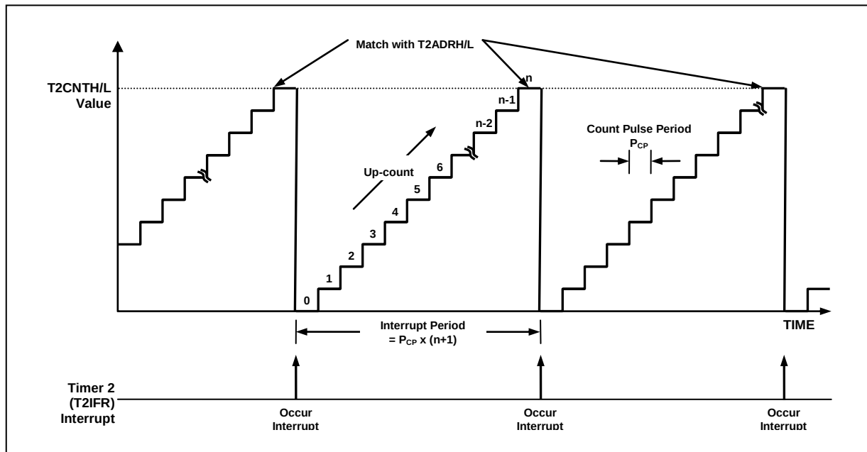
Figure 12.21 16-Bit Timer/Counter 2 Example
