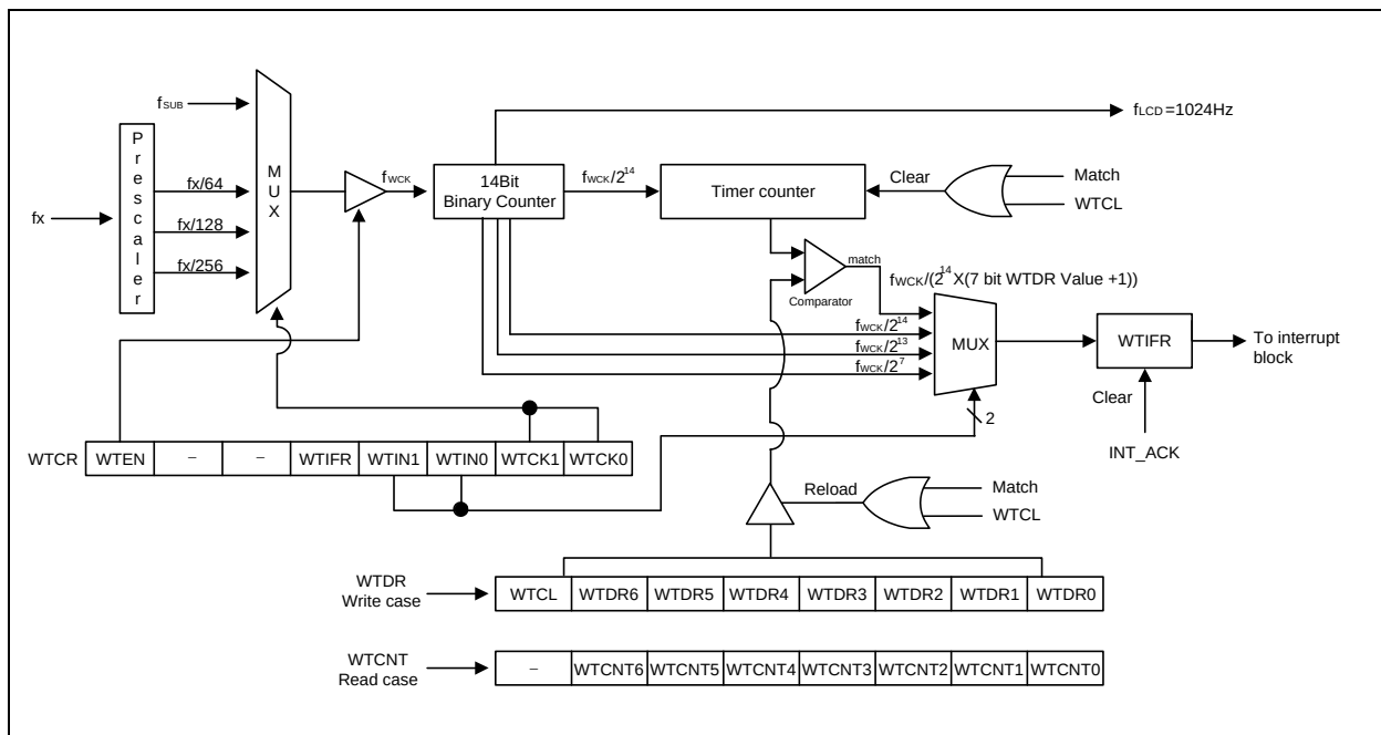
Figure 12.5 Watch Timer Block Diagram
