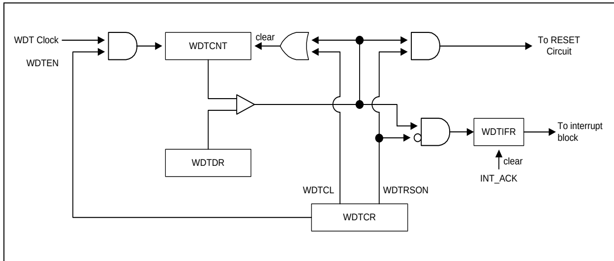
Figure 12.4 Watch Dog Timer Block Diagram
