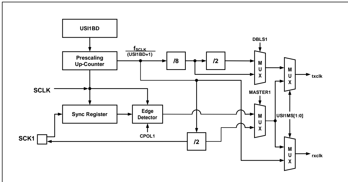
Figure 11.79 Clock Generation Block Diagram (US1)
