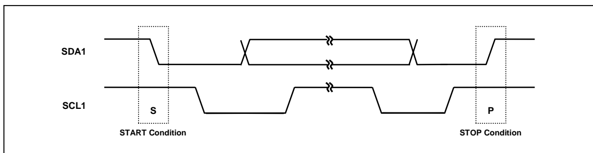
Figure 11.89 START and STOP Condition (US1)
