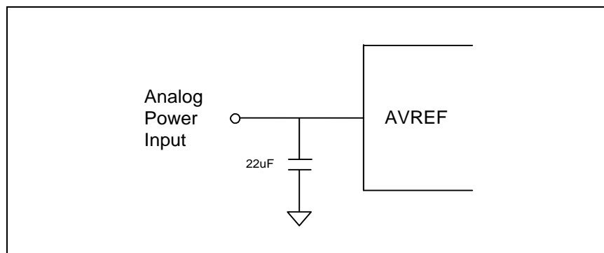
Figure 11.54 A/D Power (AVREF) Pin with Capacitor
