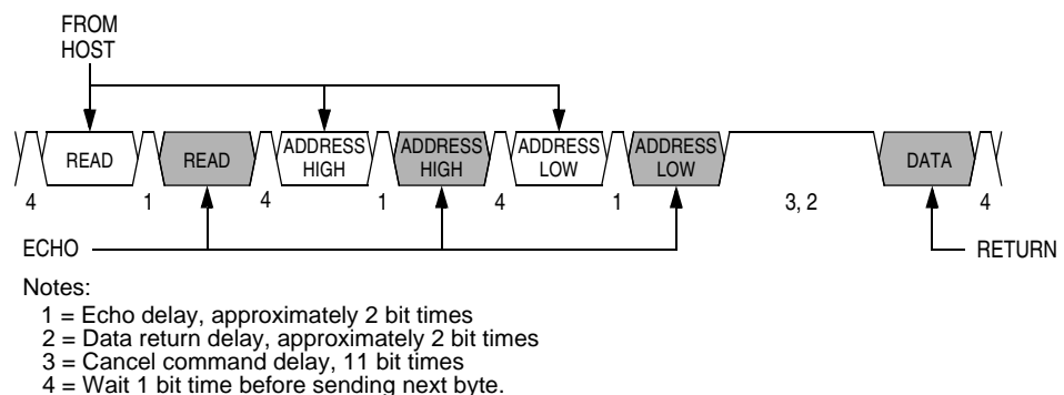
Figure 20-14. Read Transaction
