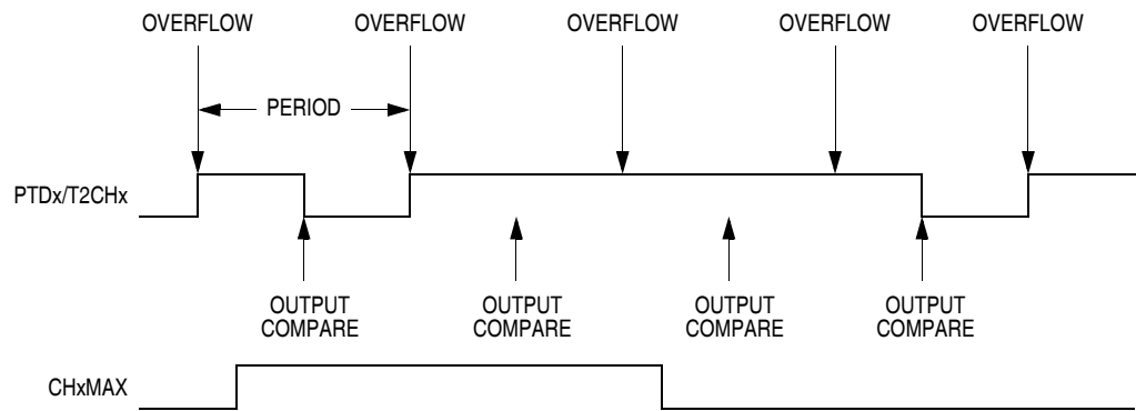
Figure 18-9. CHxMAX Latency
