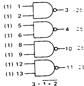
MC857/MC957 Quad 2-Input Buffers
