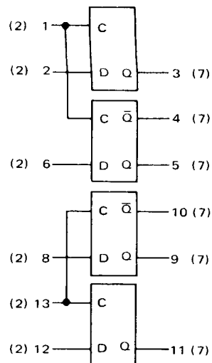
MC1814/MC1914 Quad Latch
