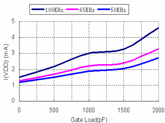
Operation Current VS Load
