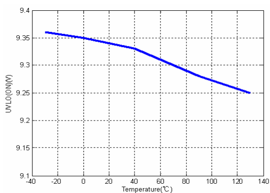
UVLO (On) Voltage VS Temp
