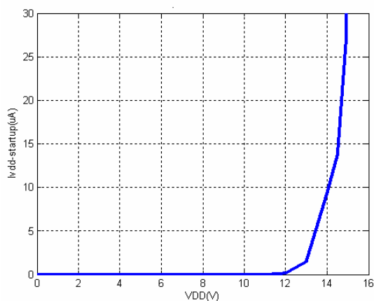
Start Current Vs VDD Voltage
