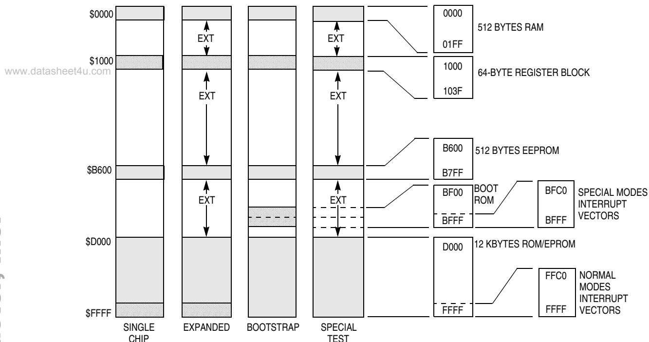
Figure 2-4. Memory Map for MC68HC(7)11E9
