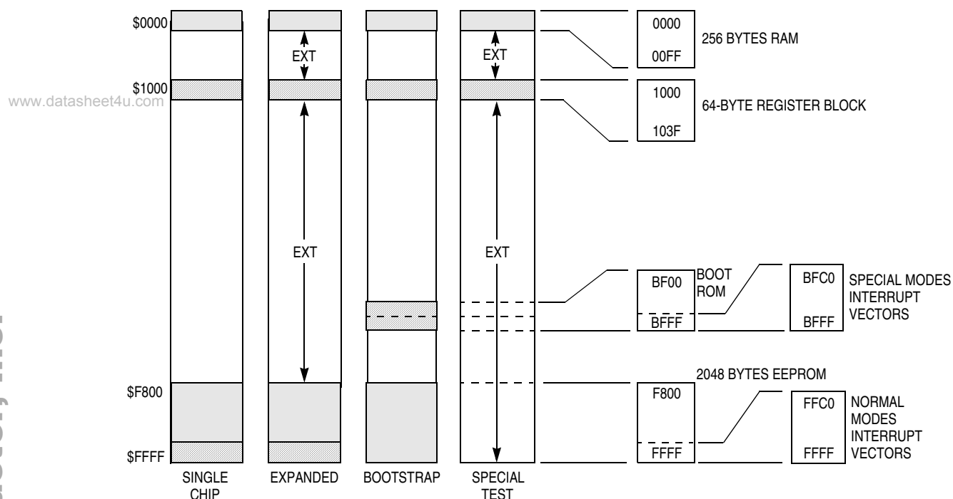
Figure 2-6. Memory Map for MC68HC811E2
