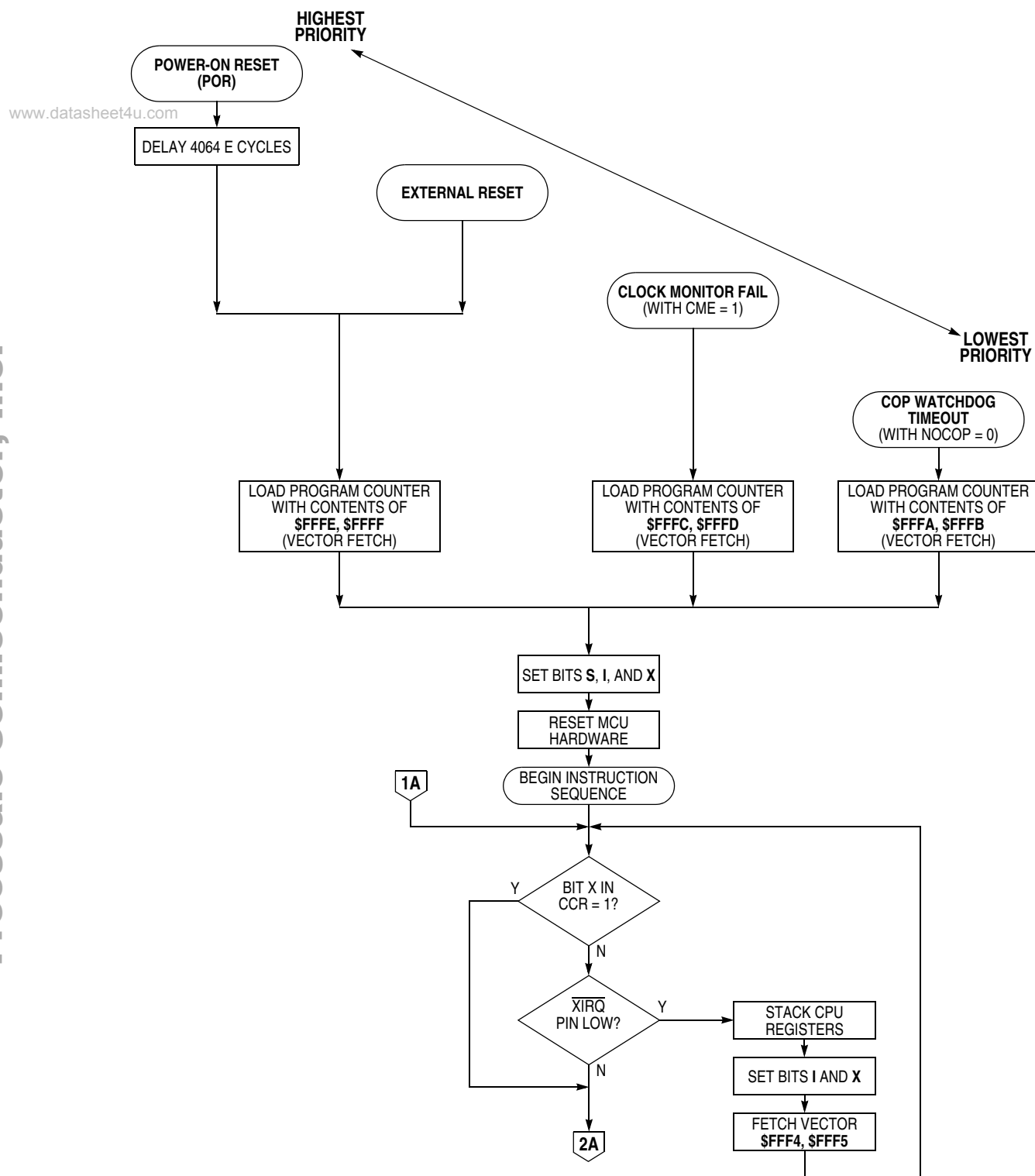
Figure 5-5. Processing Flow Out of Reset (Sheet 1 of 2)
