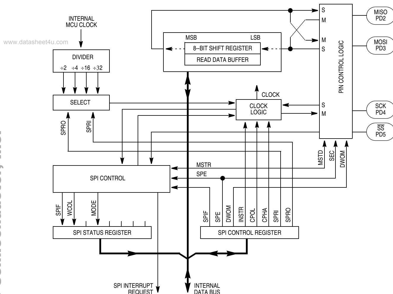
Figure 8-1. SPI Block Diagram
