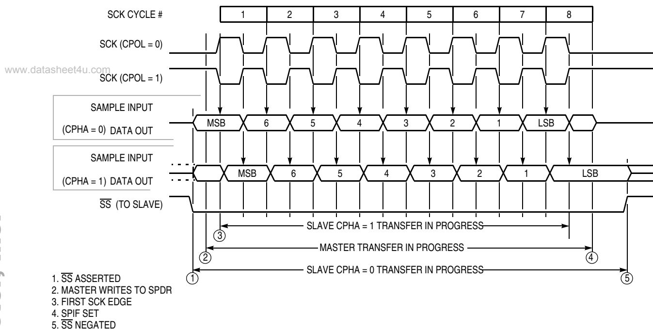
Figure 8-2. SPI Transfer Format
