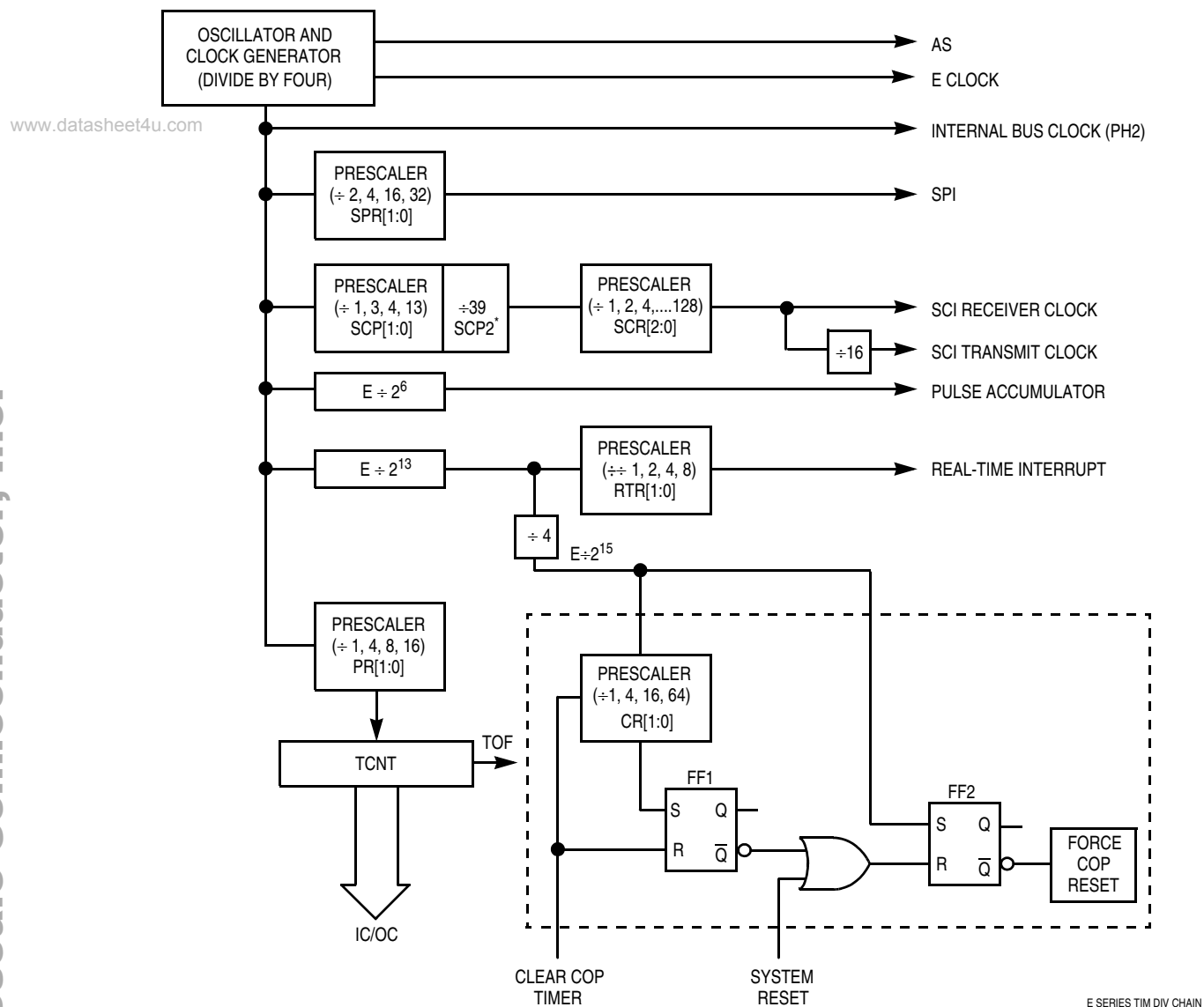
Figure 9-1. Timer Clock Divider Chains
