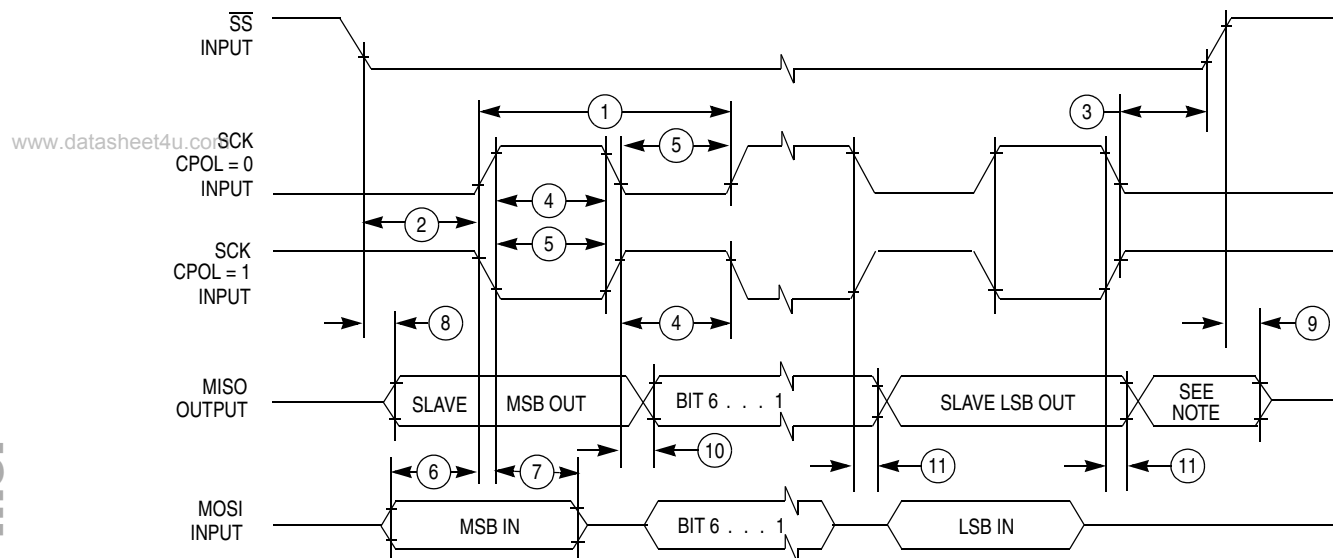
A) SPI Slave Timing (CPHA = 0)
