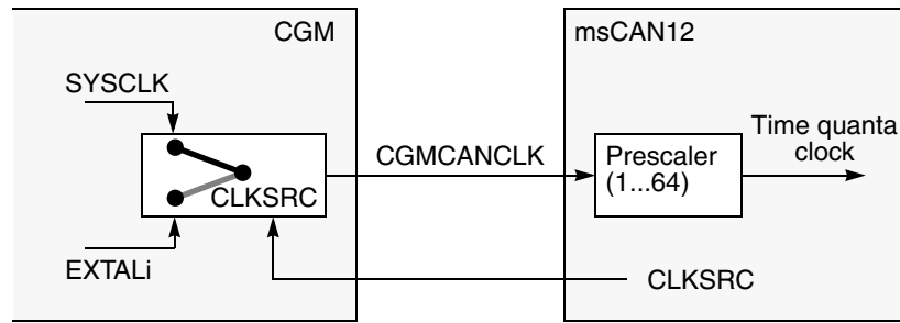
Figure 18-7. Clocking Scheme
