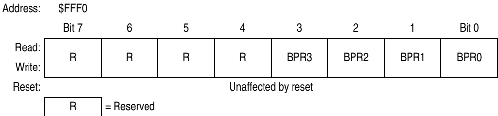
Figure 2-5. FLASH 2TS Block Protect Register (FLBPR)
