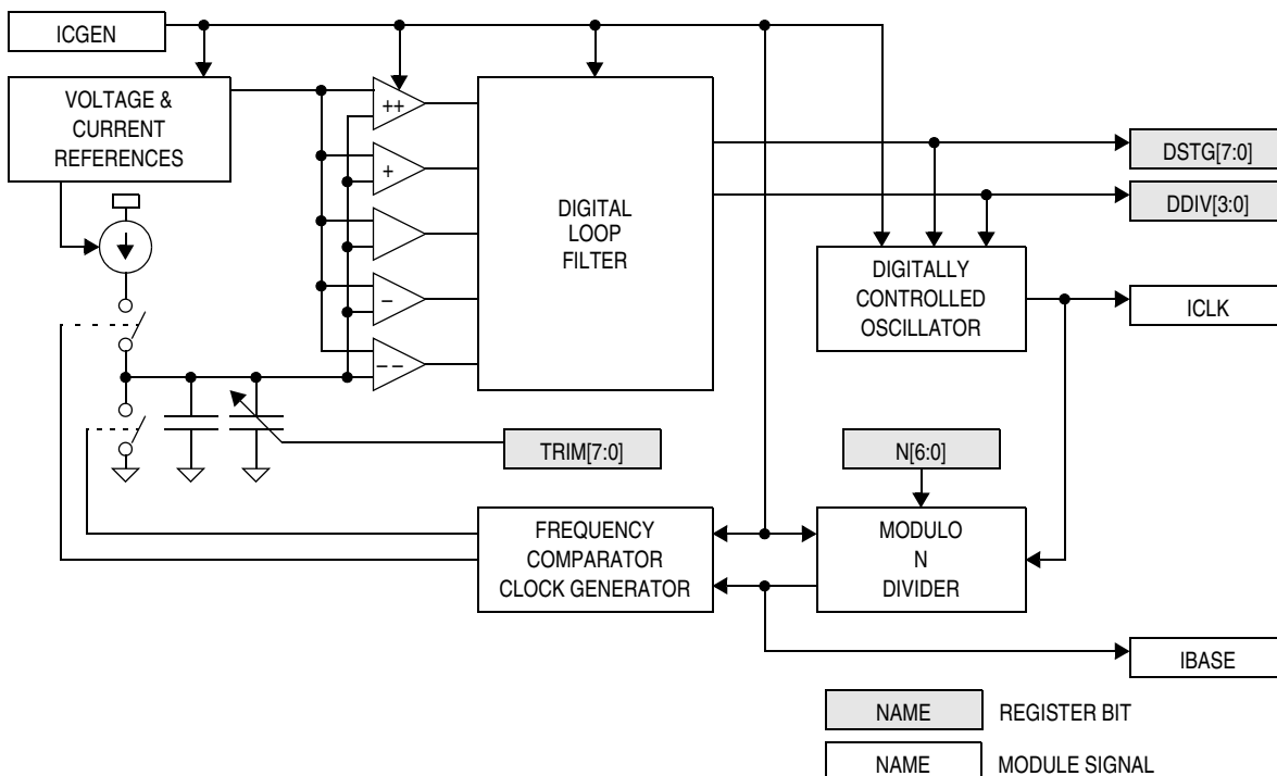
Figure 6-3. Internal Clock Generator Block Diagram
