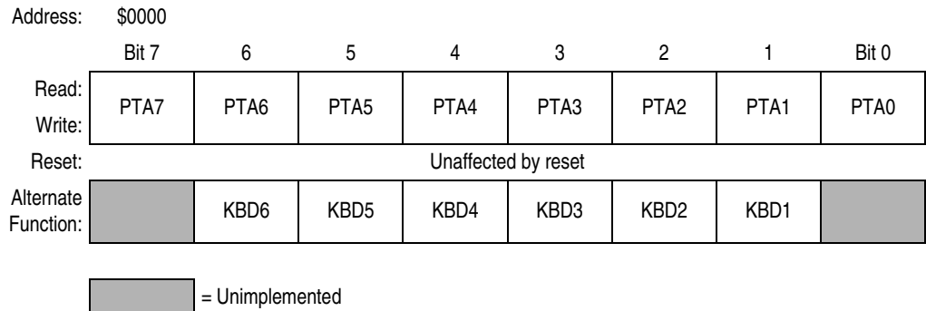
Figure 9-2. Port A Data Register (PTA)
