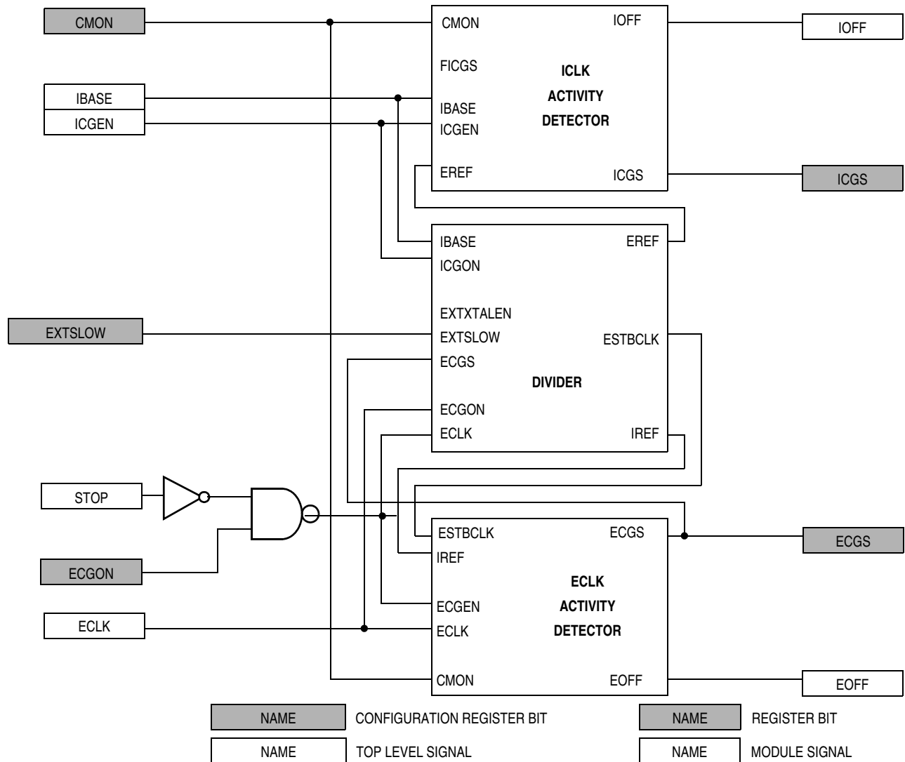
Figure 6-5. Clock Monitor Block Diagram
