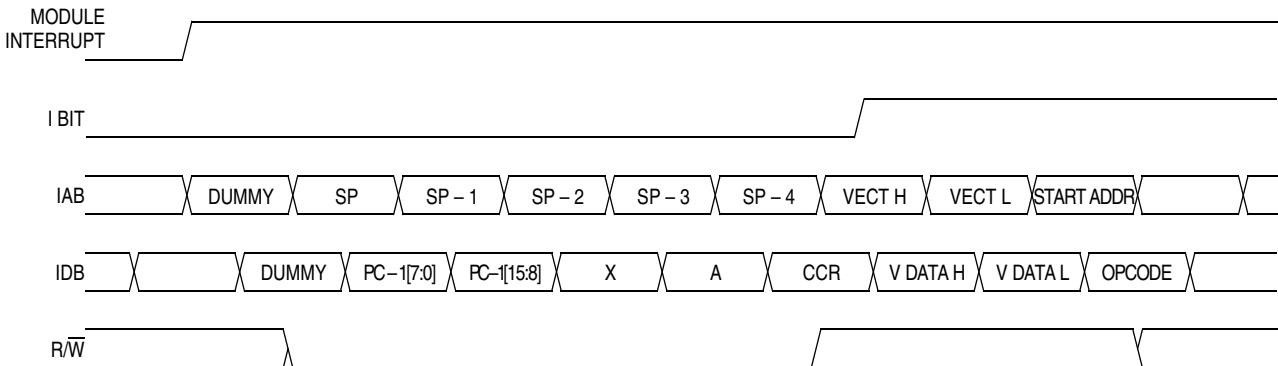
Figure 10-8. Interrupt Entry
