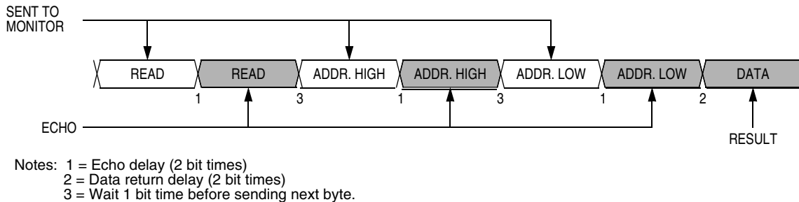
Figure 12-8. Read Transaction
