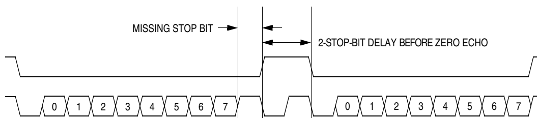
Figure 12-9. Break Transaction
