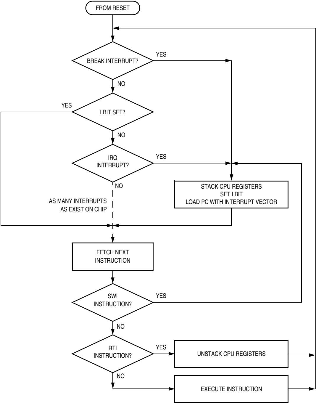
Figure 10-10. Interrupt Processing
