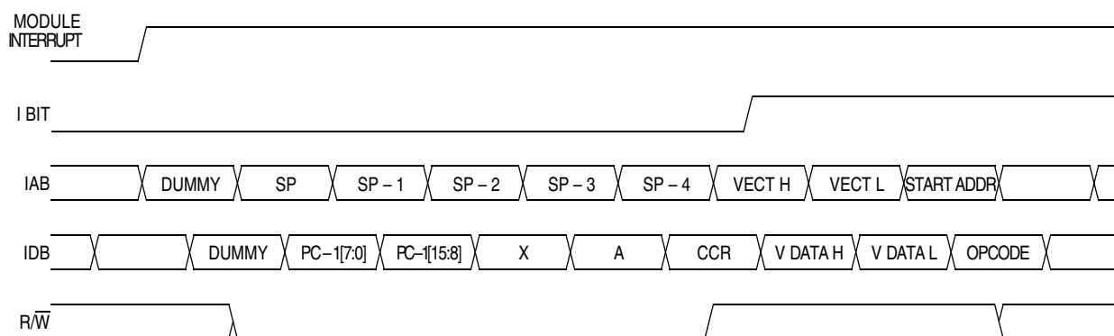
Figure 10-8. Interrupt Entry
