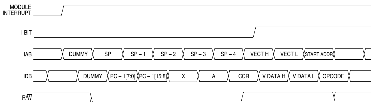
Figure 8-9. Interrupt Entry
