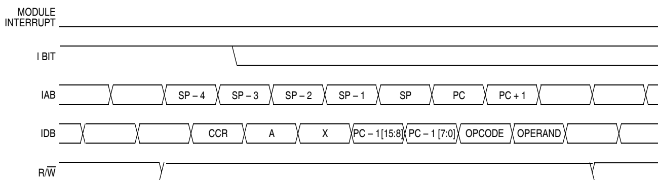
Figure 8-10. Interrupt Recovery
