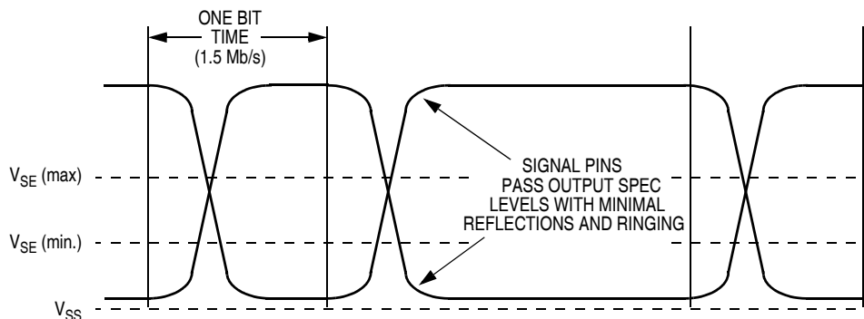
Figure 11-11. Receiver Characteristics
