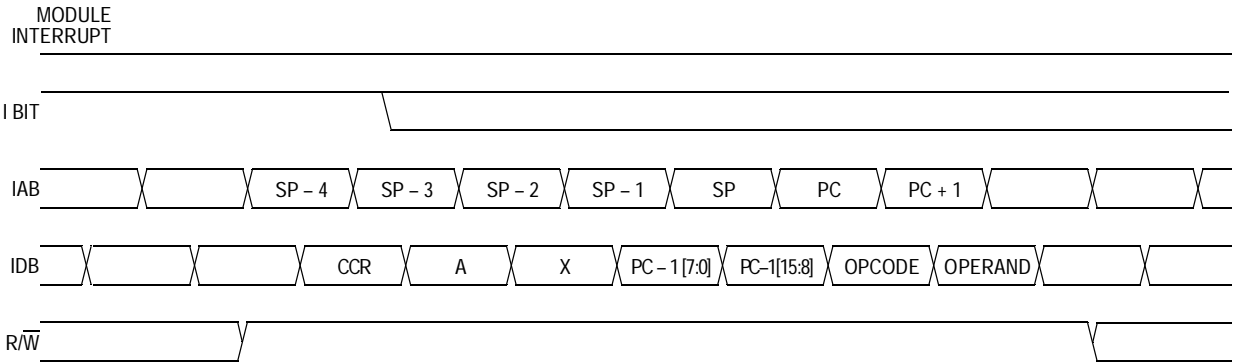
Figure 9-9. Interrupt Recovery
