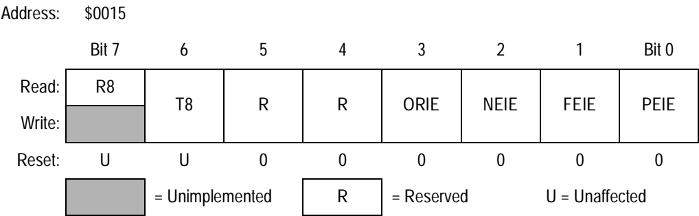
Figure 17-11. SCI Control Register 3 (SCC3)
