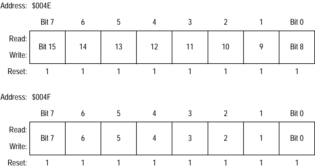
Figure 19-5. TIM Counter Modulo Registers (TMODH–TMODL)
