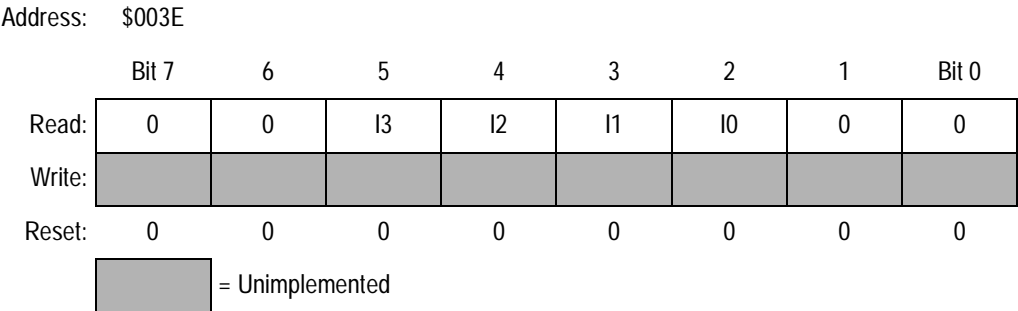
Figure 21-20. BDLC State Vector Register (BSVR)
