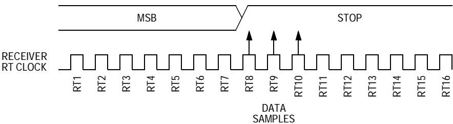
Figure 17-7. Slow Data
