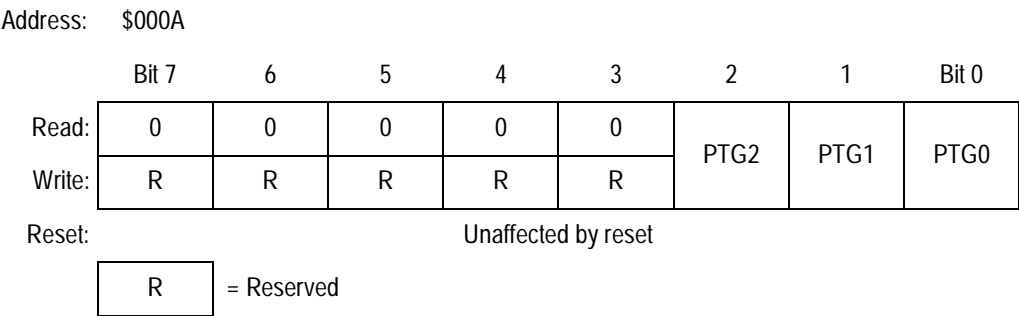
Figure 20-20. Port G Data Register (PTG)
