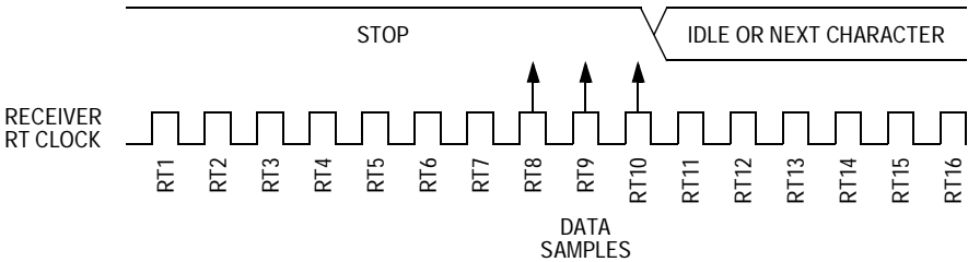
Figure 17-8. Fast Data
