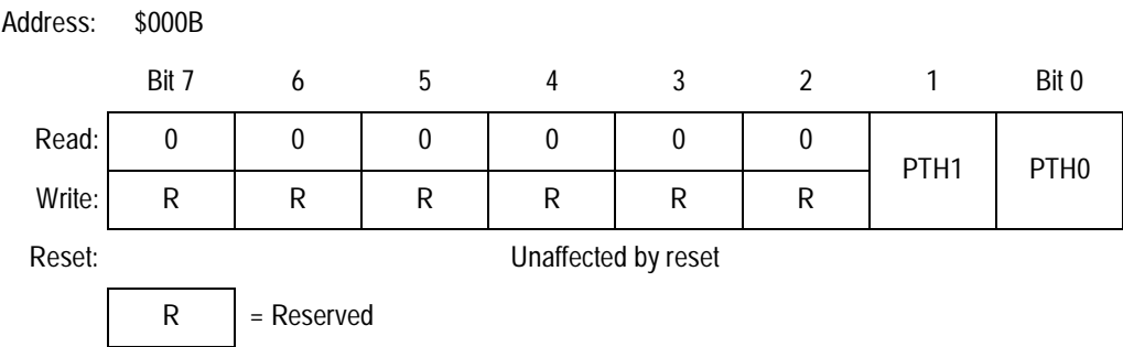
Figure 20-23. Port H Data Register (PTH)
