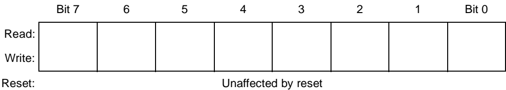
Figure 8-2. Accumulator (A)
