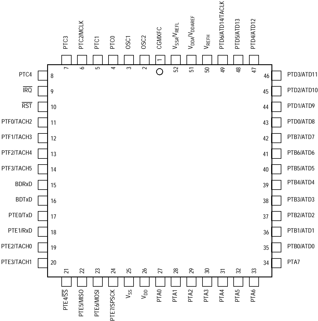
Figure 1-2. MC68HC908AS60 (52-Pin PLCC)
