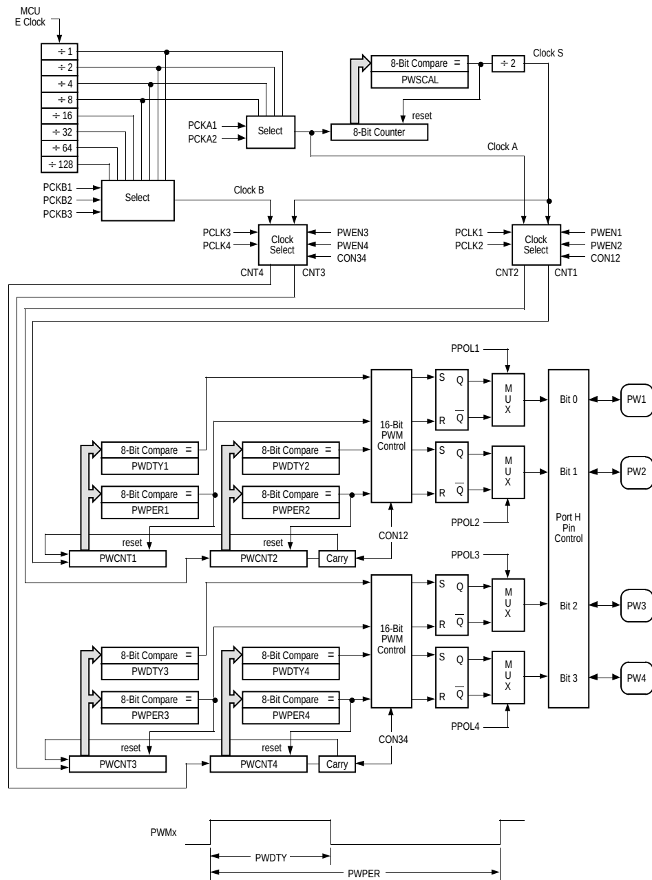
Figure 10-1. PWM Timer Module Block Diagram
