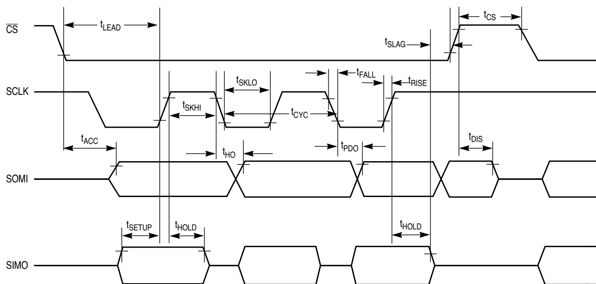
Figure A-3 SPI Timing — Active Low SCLK
