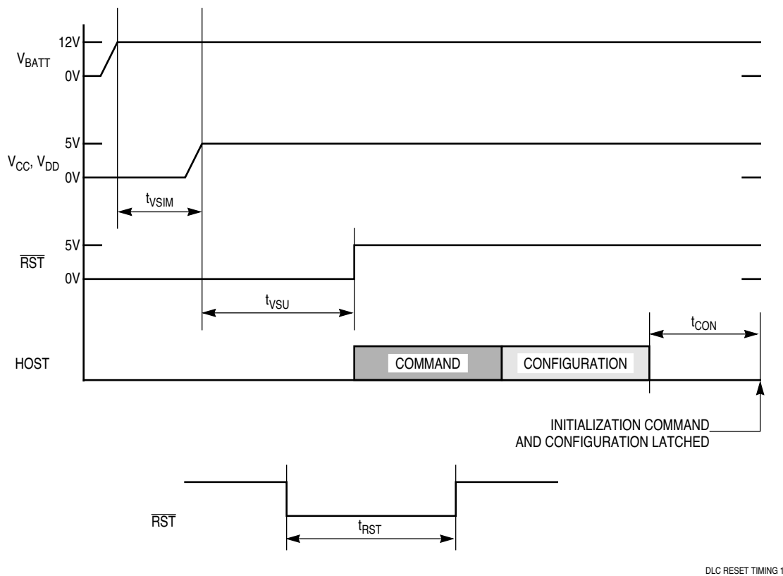
Figure A-5 Reset Timing
