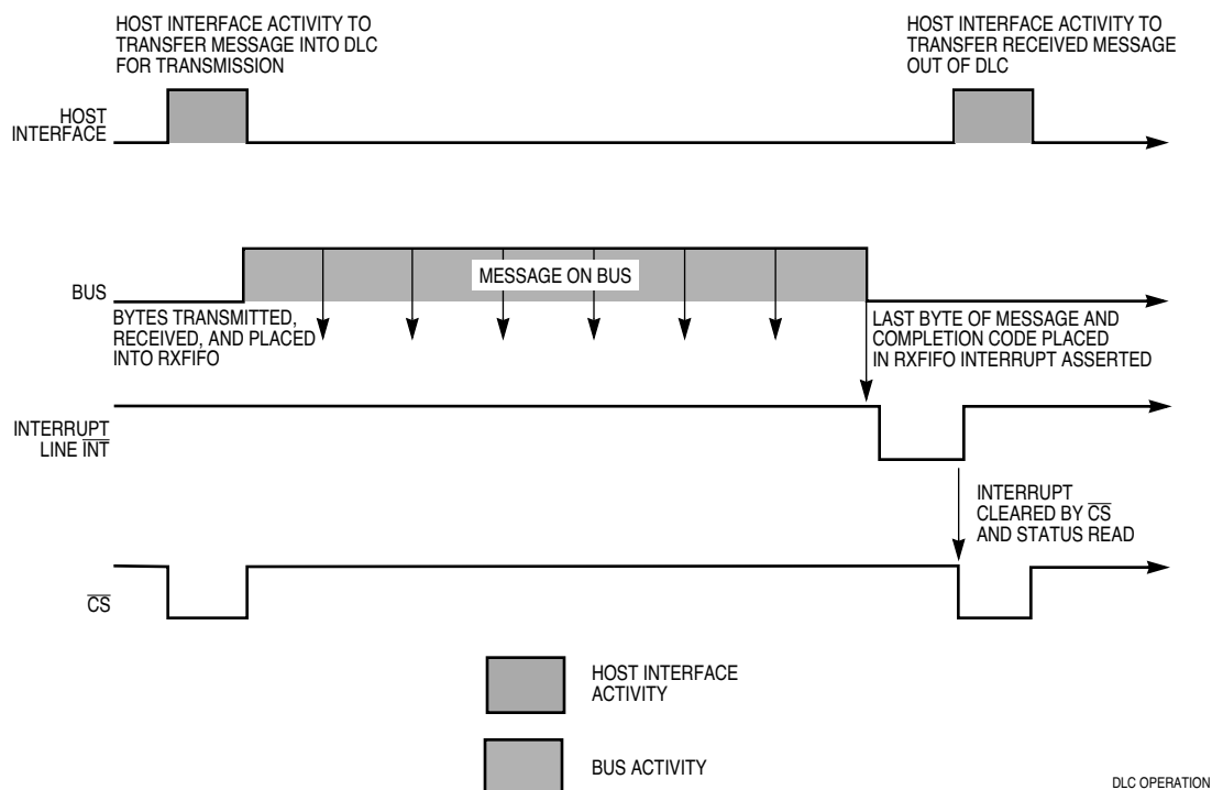
Figure 4-3 DLC Operation
