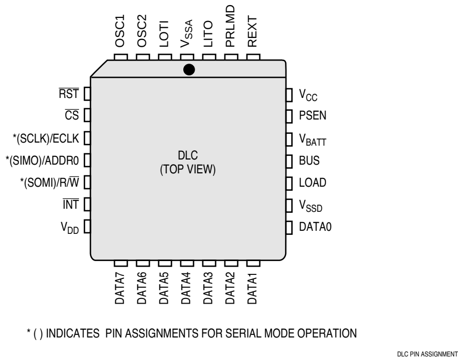
Figure B-1 MC68HC58 28-Pin PLCC
