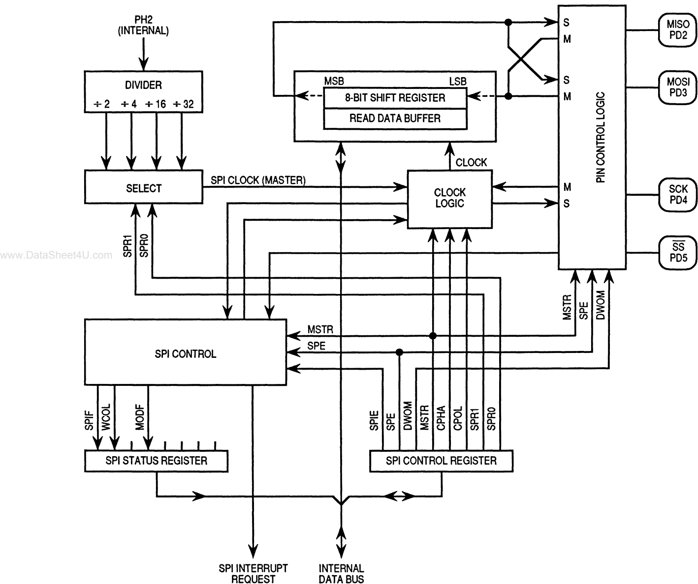
Figure 8-1. SPI Block Diagram
