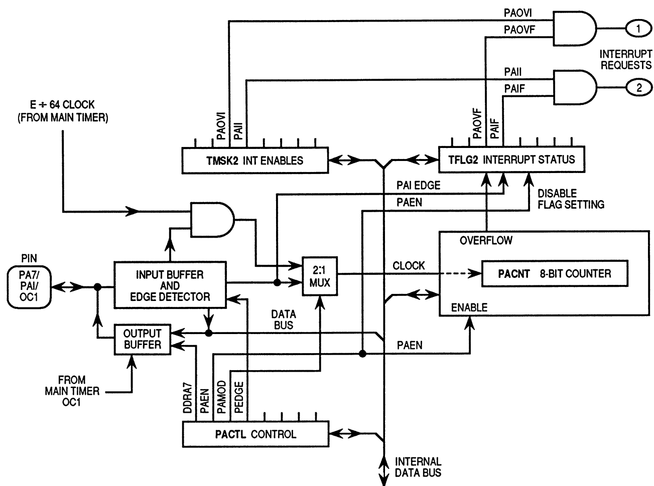
Figure 9–3. Pulse Accumulator
