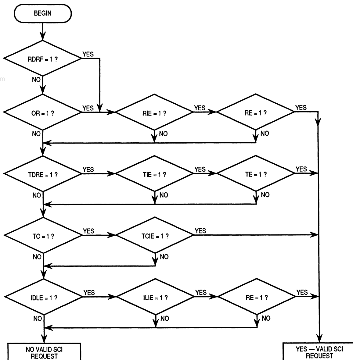
Figure 7-4. Interrupt Source Resolution Within SCI
