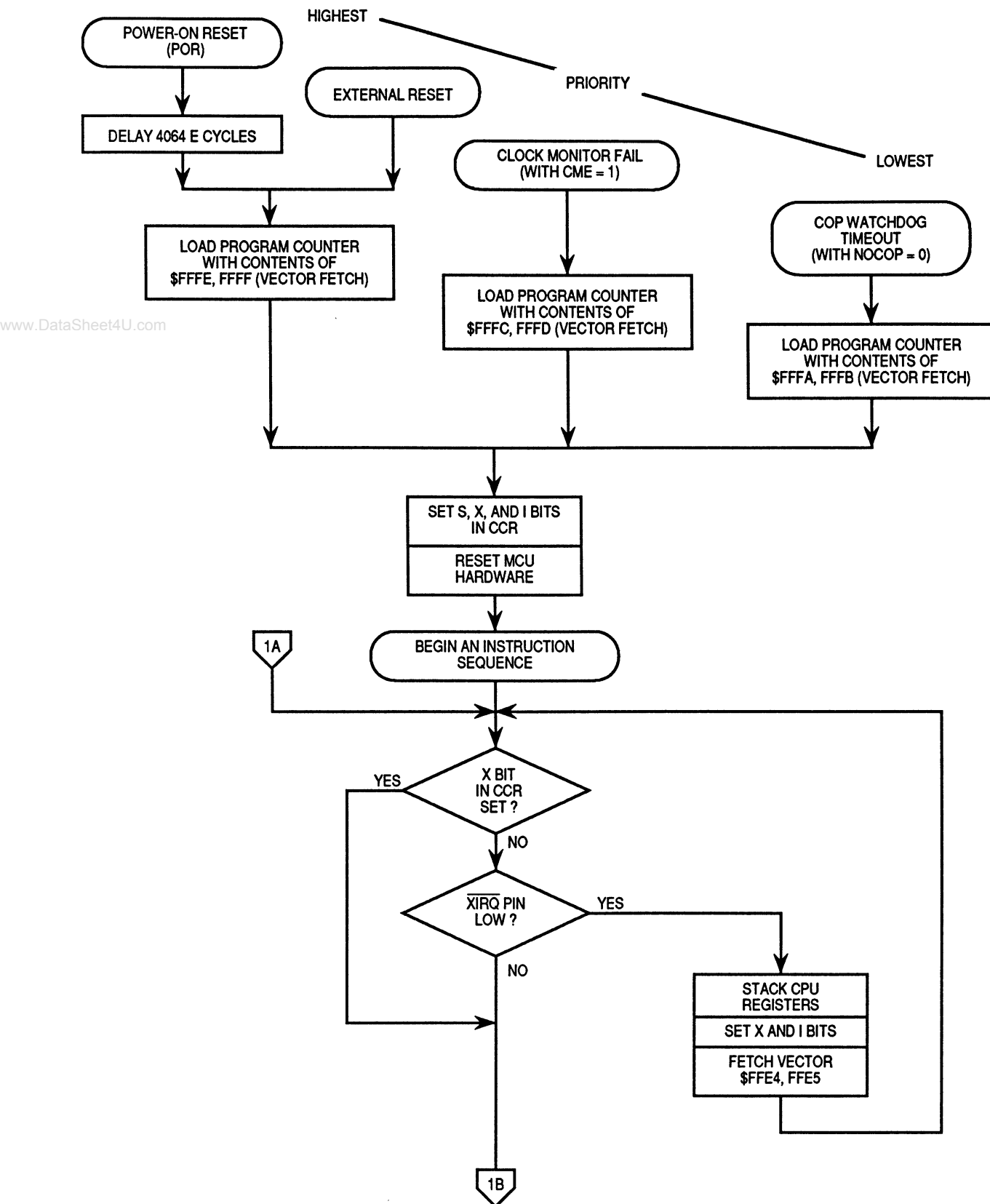
Figure 5–1. Processing Flow out of Reset (1 of 2)
