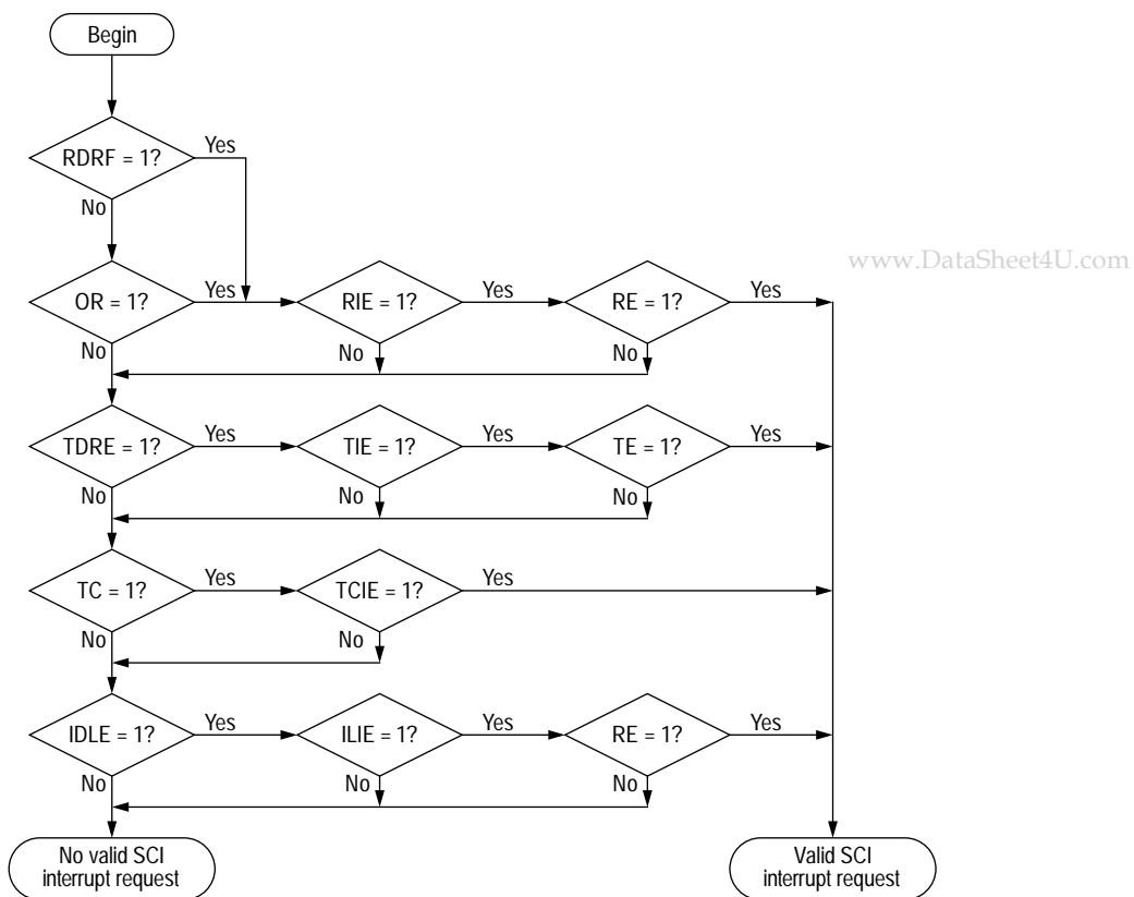
Figure 5-6 Interrupt source resolution within the SCI subsystem
