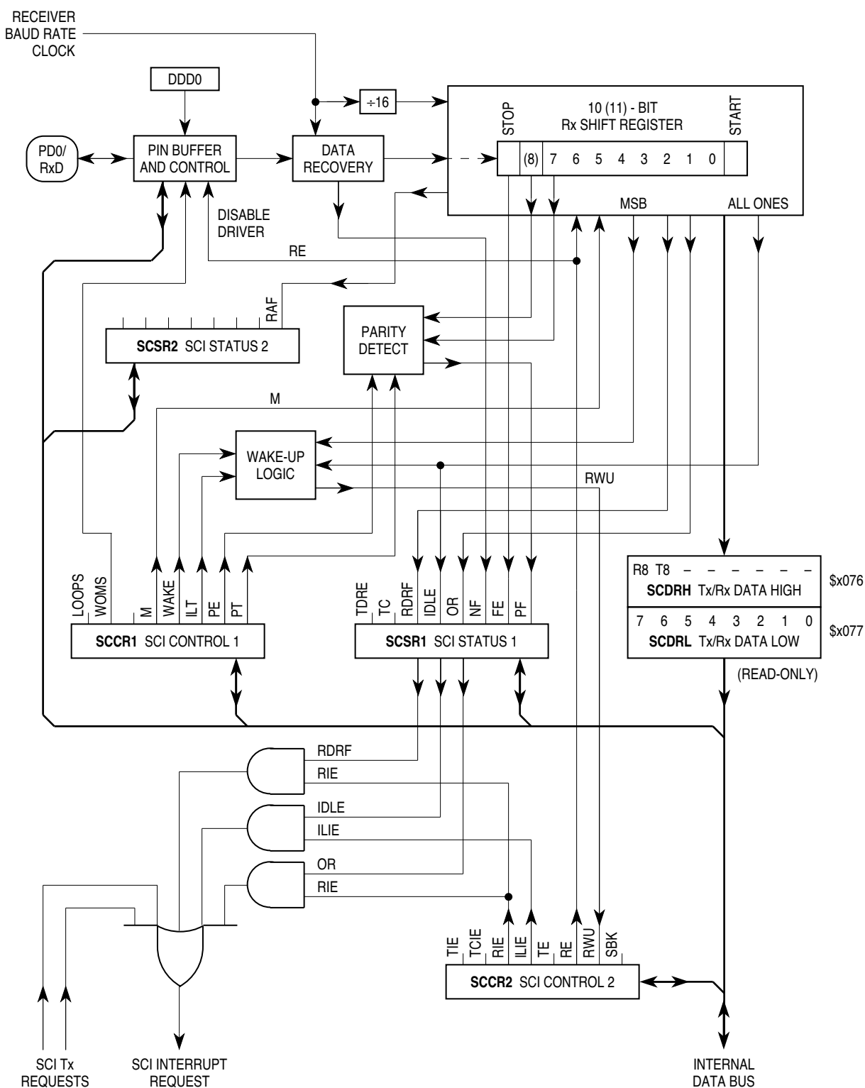
Figure 11 SCI Receiver Block Diagram
