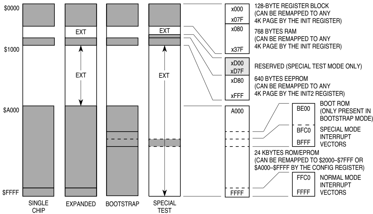
Figure 4 Memory Map
