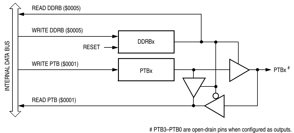
Figure 18-8. Port B I/O Circuit
