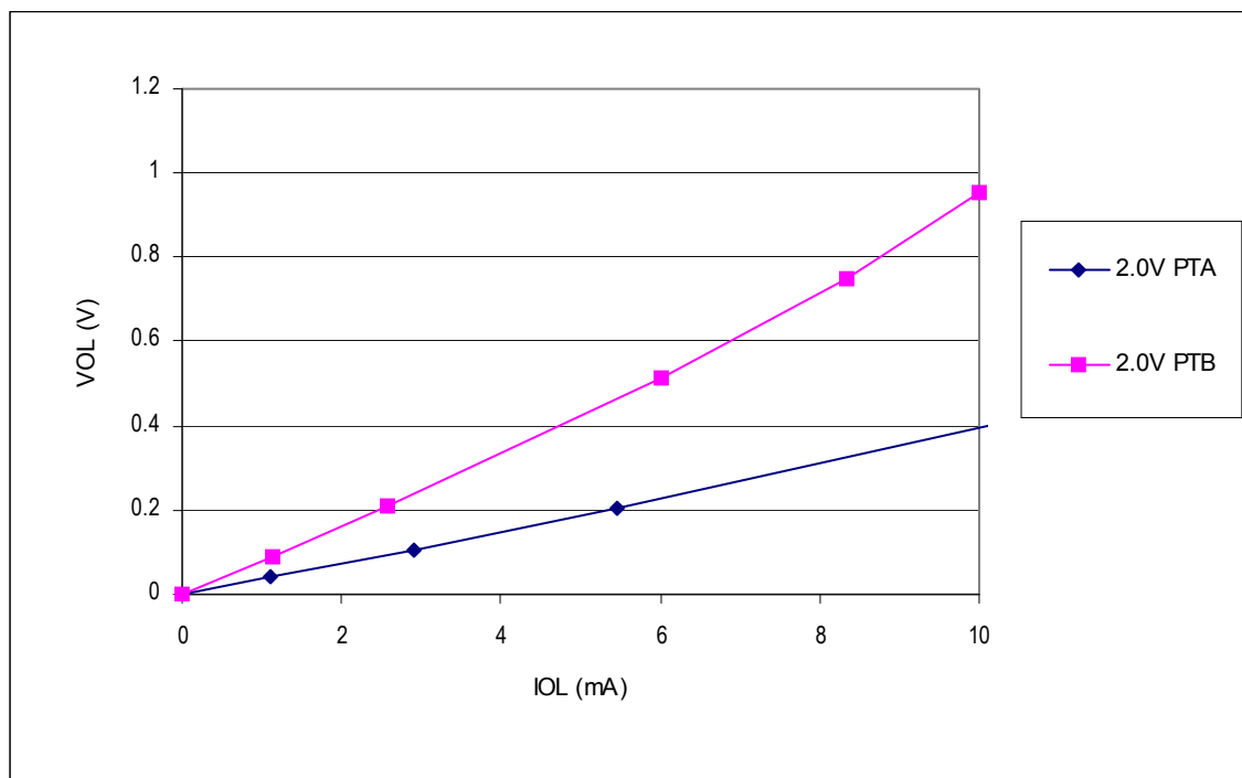
Figure 16-8. Typical 2-Volt Output Low Voltage versus Output Low Current (25°C)
