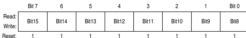
Figure 14-7. TIM Counter Modulo High Register (TMDH)
