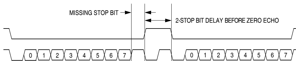
Figure 15-12. Break Transaction
