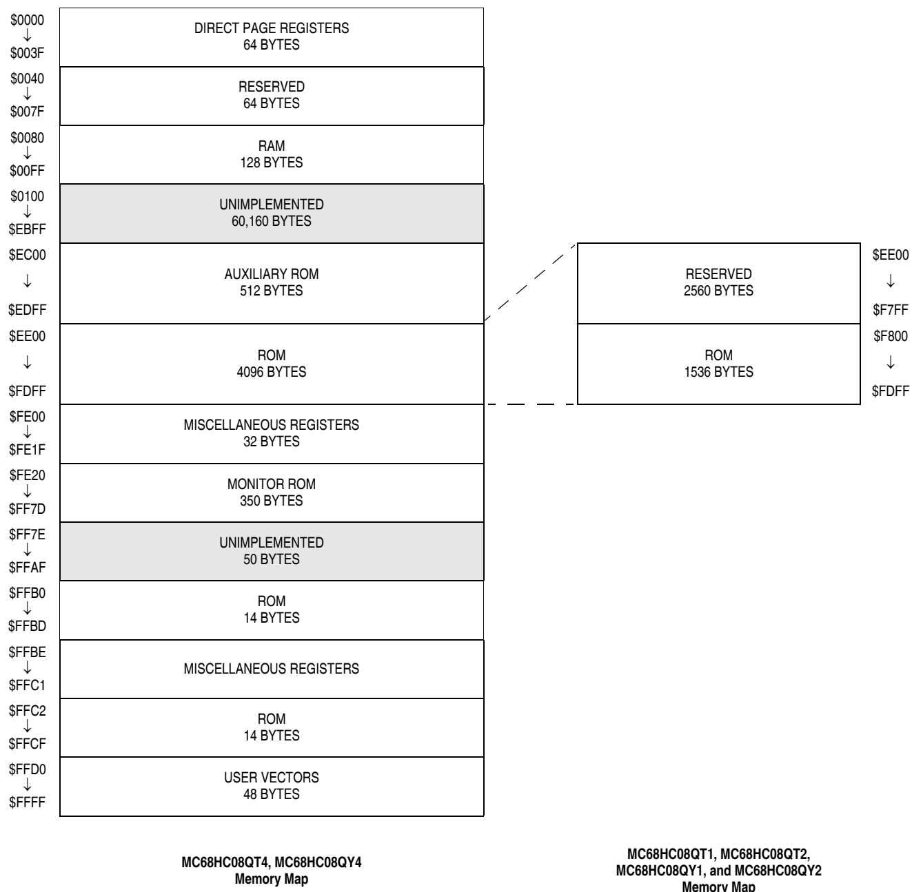
Figure 2-1. Memory Map
