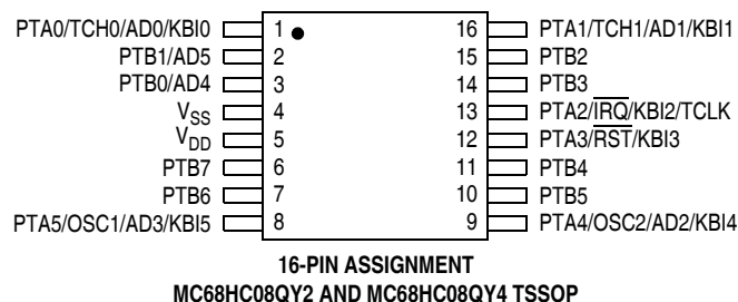
Figure 1-2. MCU Pin Assignments
