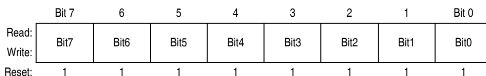
Figure 14-8. TIM Counter Modulo Low Register (TMDL)
