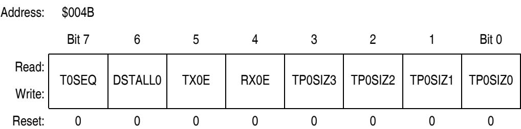
Figure 9-15. USB Embedded Device Control Register 0 (DCR0)
