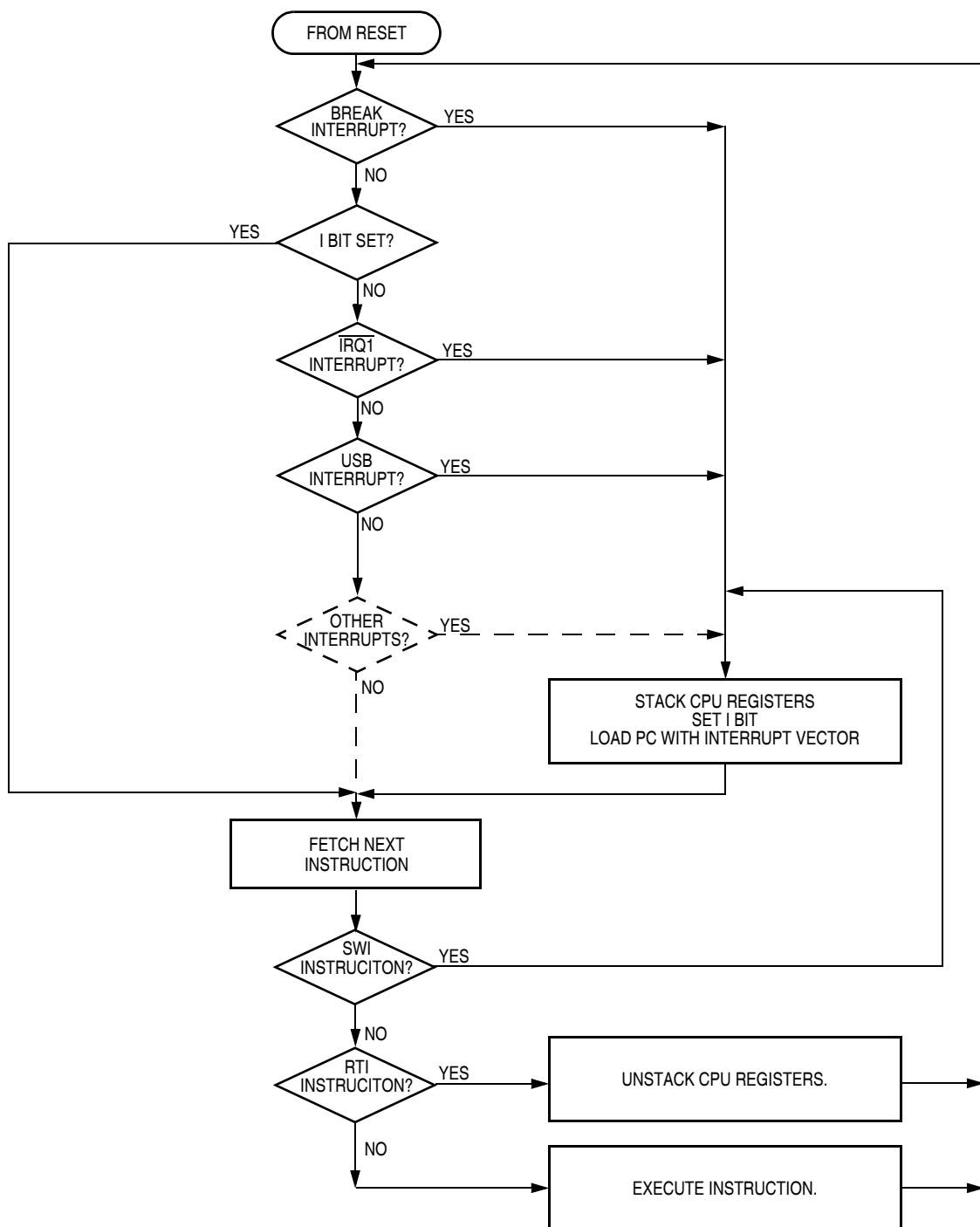
Figure 7-8. Interrupt Processing
