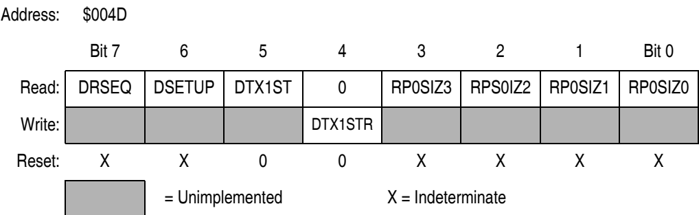
Figure 9-17. USB Embedded Device Status Register (DSR)
