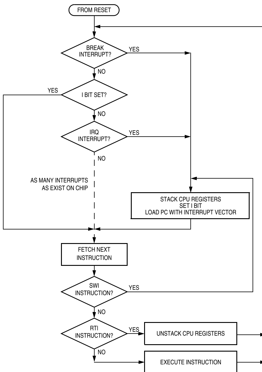
Figure 14-11. Interrupt Processing
