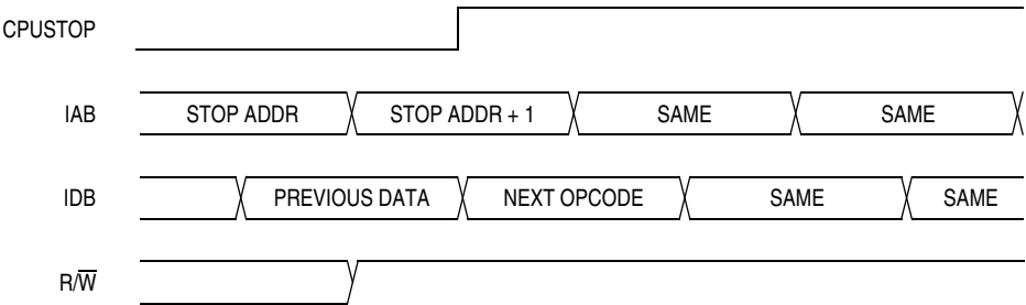
Figure 14-20. Stop Mode Entry Timing
