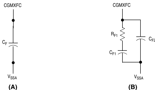
Figure 4-11. PLL Filter
