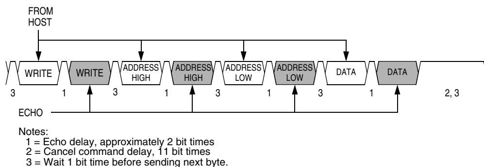
Figure 19-13. Write Transaction
