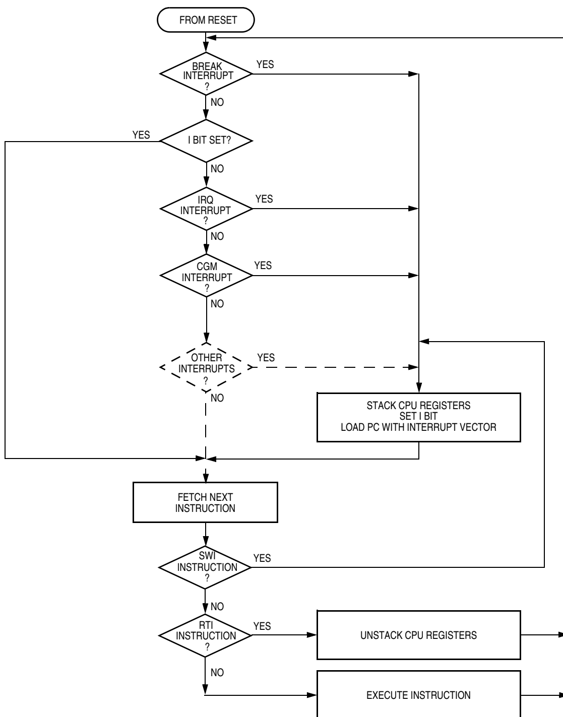
Figure 13-6. Interrupt Processing
