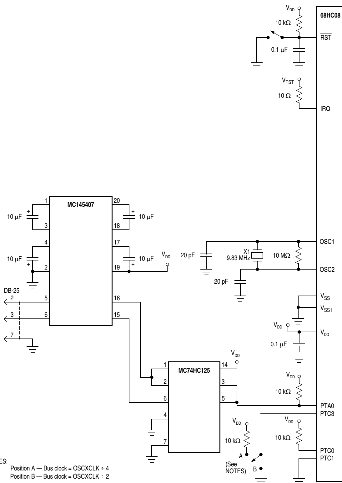
Figure 9-1. Monitor Mode Circuit
