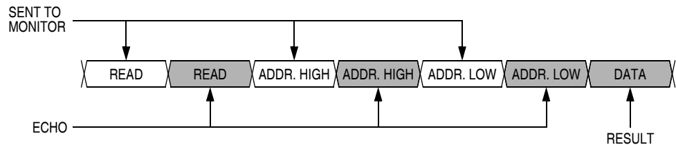
Figure 9-4. Read Transaction
