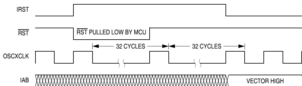
Figure 7-4. Internal Reset Timing
