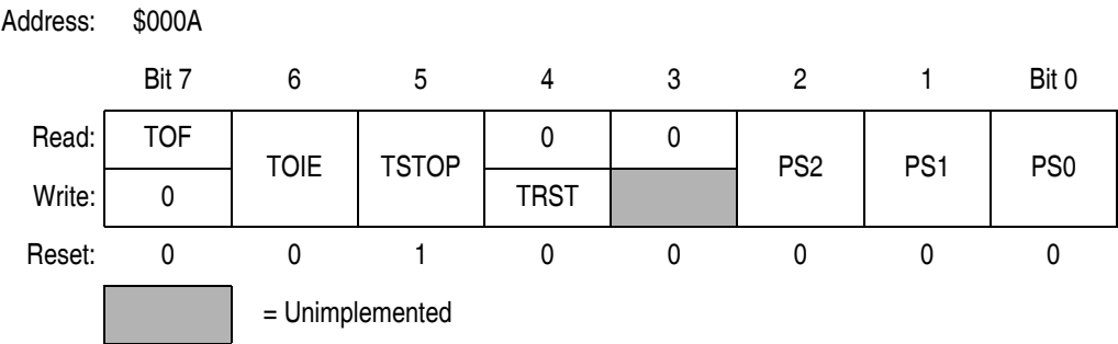
Figure 10-3. TIM Status and Control Register (TSC)
