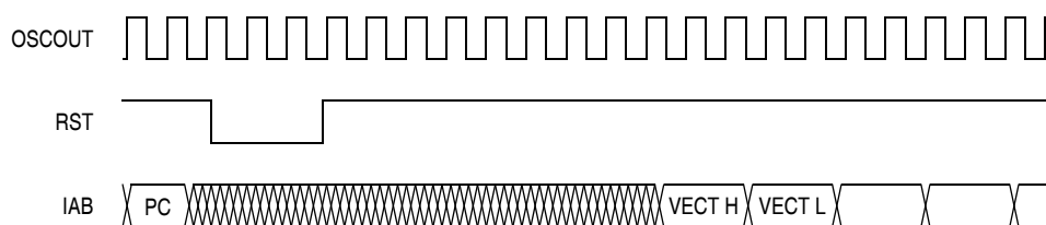
Figure 7-3. External Reset Timing
