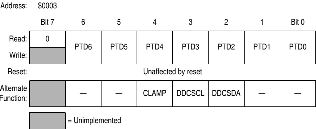
Figure 15-12. Port D Data Register (PTD)
