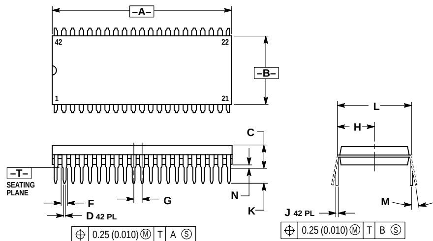
Figure 20-2. 42-Pin SDIP (Case 858)
