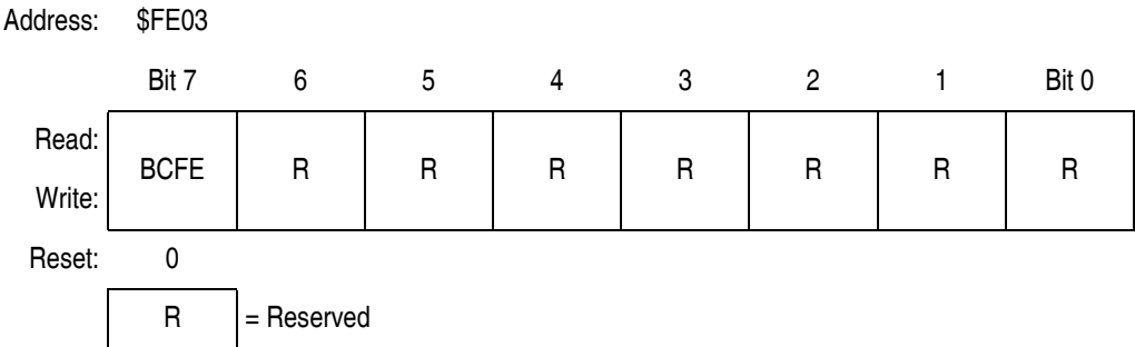
Figure 18-6. SIM Break Flag Control Register (SBFCR)
