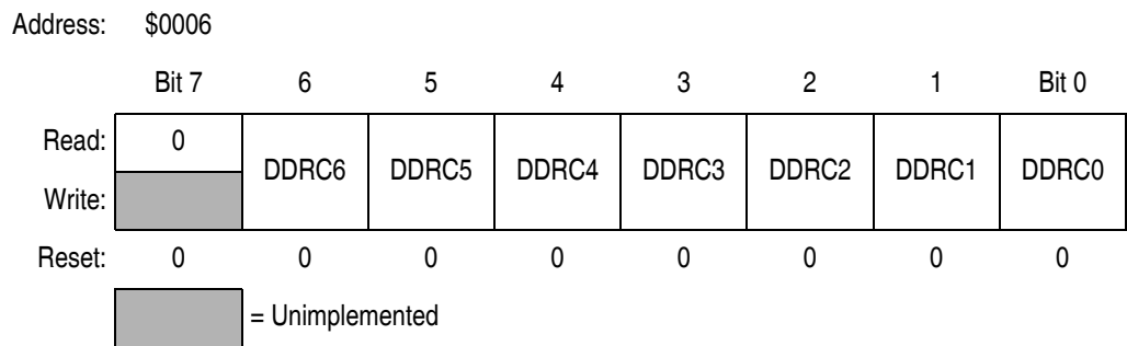
Figure 15-10. Data Direction Register C (DDRC)
