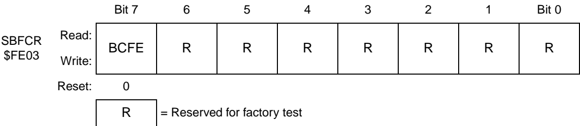
Figure 8-17. SIM Break Flag Control Register (SBFCR)
