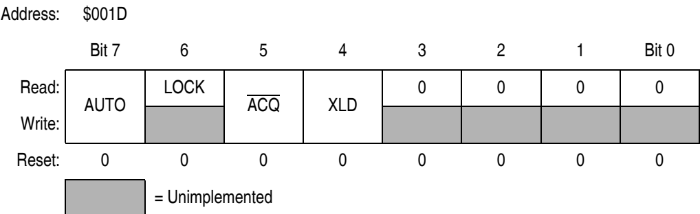
Figure 9-5. PLL Bandwidth Control Register (PBWC)
