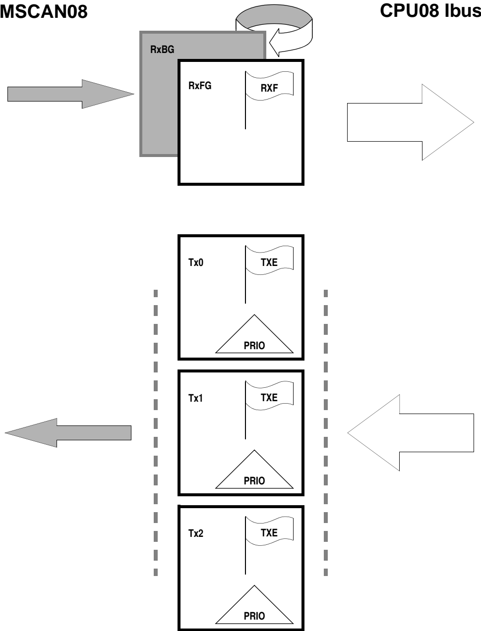
Figure 21-2. User Model for Message Buffer Organization
