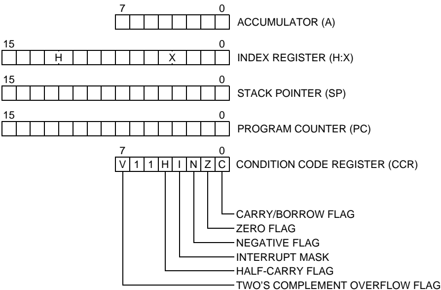
Figure 7-1. CPU Registers
