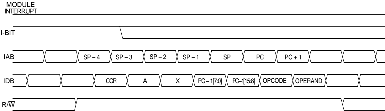
Figure 8-8. Interrupt Recovery
