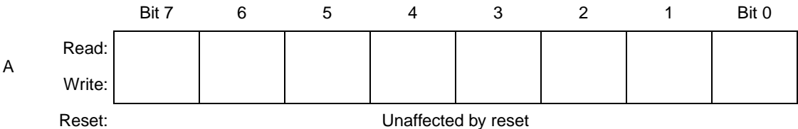
Figure 7-2. Accumulator (A)
