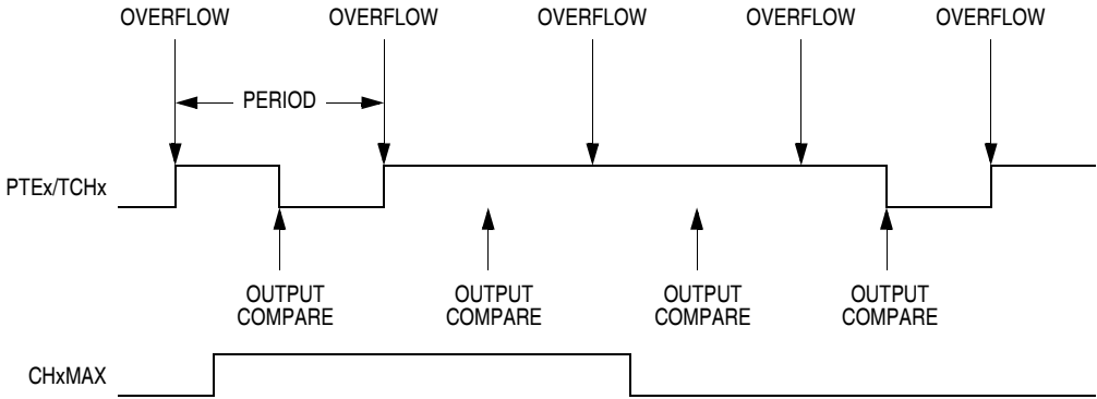
Figure 23-8. CHxMAX Latency
