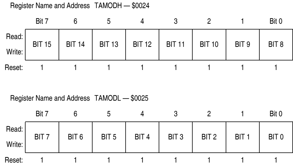
Figure 23-6. TIMA Counter Modulo Registers (TAMODH and TAMODL)
