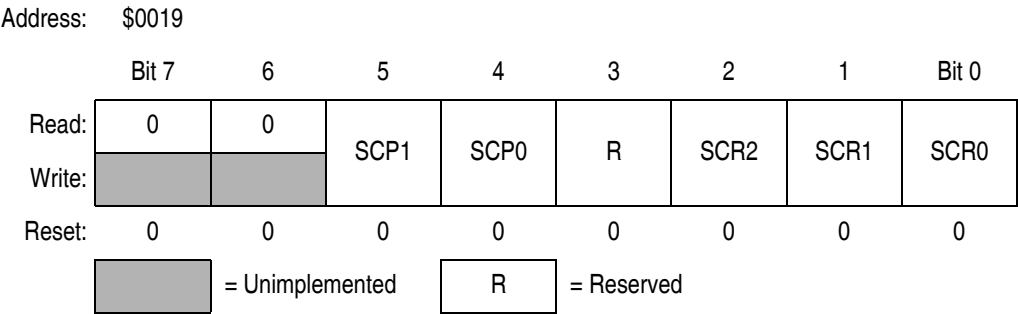
Figure 16-18. SCI Baud Rate Register (SCBR)
