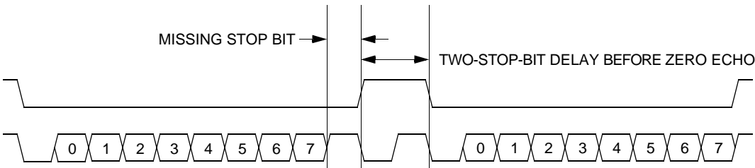
Figure 12-5. Break Transaction
