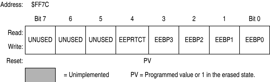
Figure 6-4. EEPROM-2 Nonvolatile Register (EE2NVR)
