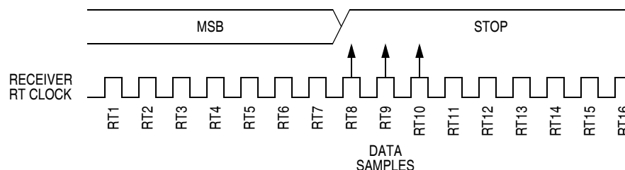
Figure 16-9. Slow Data
