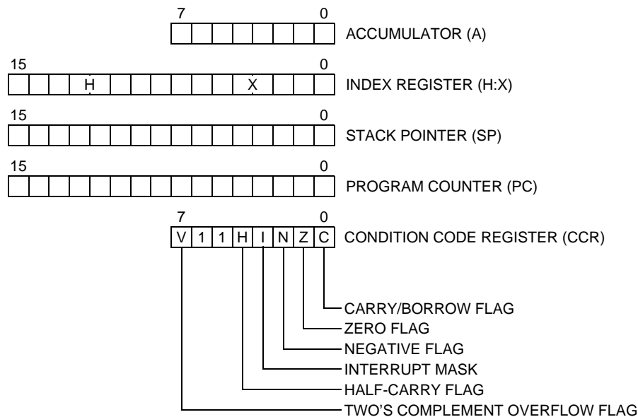
Figure 8-1. CPU registers
