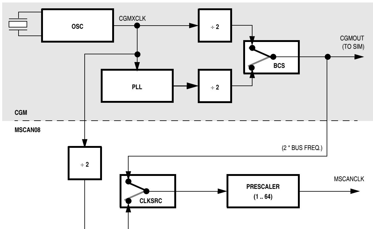
Figure 22-7. Clocking Scheme
