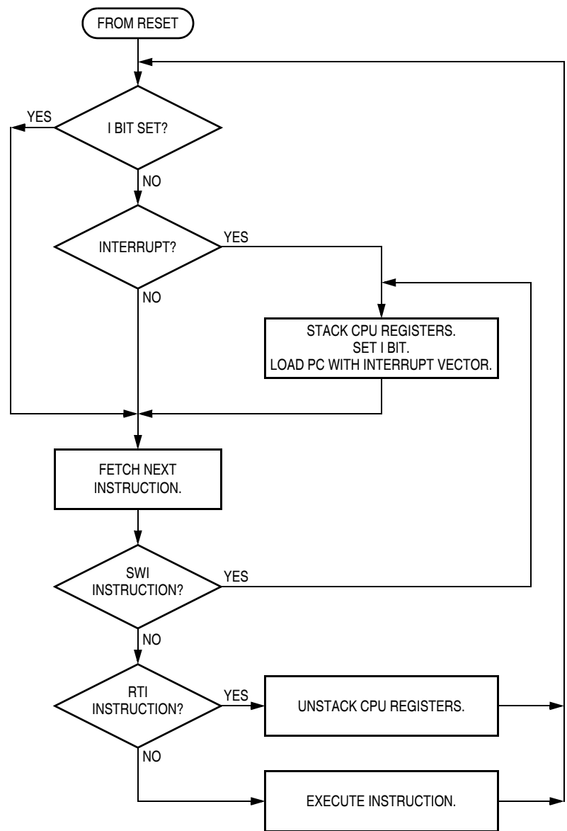
Figure 16-2. IRQ Interrupt Flowchart
