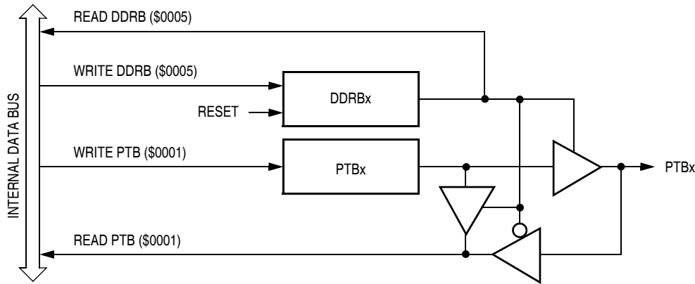
Figure 21-6. Port B I/O Circuit
