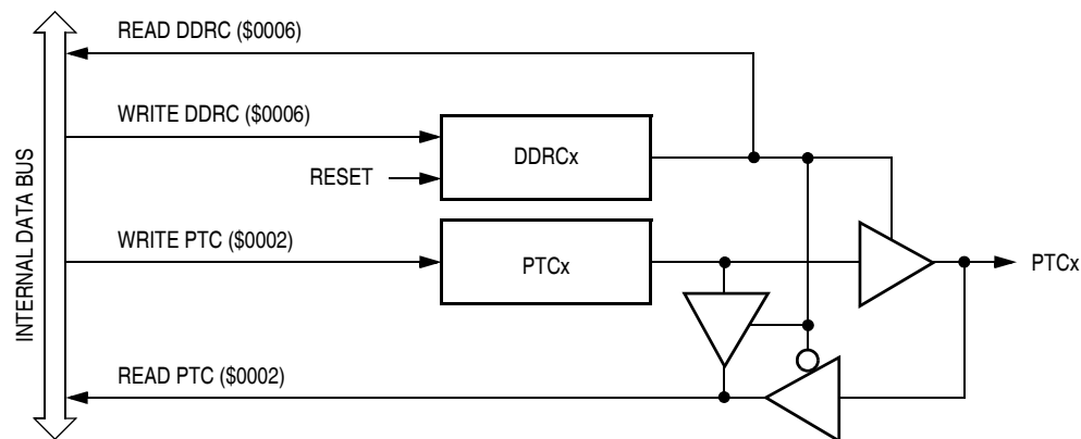
Figure 21-9. Port C I/O Circuit
