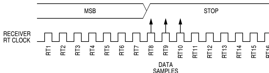
Figure 17-9. Slow Data
