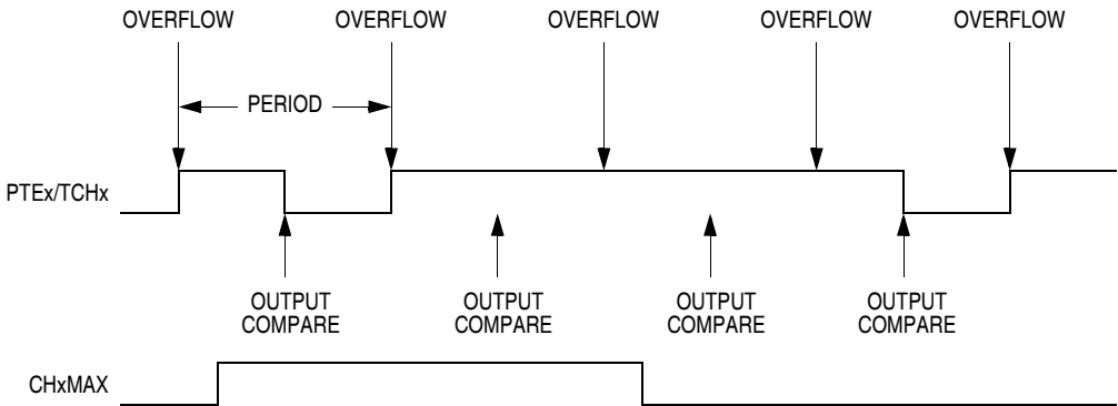
Figure 24-8. CHxMAX Latency
