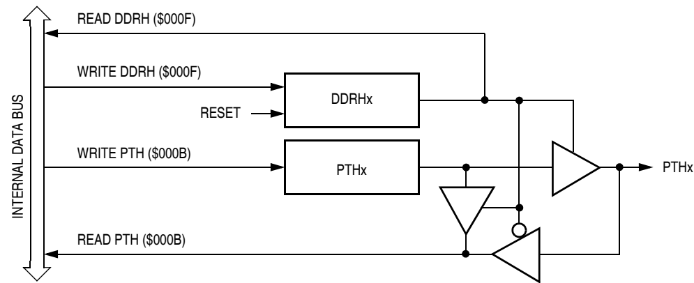
Figure 21-24. Port H I/O Circuit
