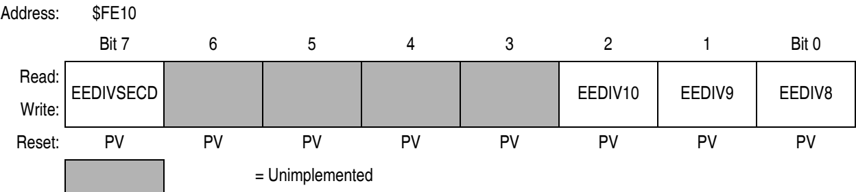
Figure 27-3. EEPROM-2 Divider High Non-volatile Register (EEDIVHNVR)
