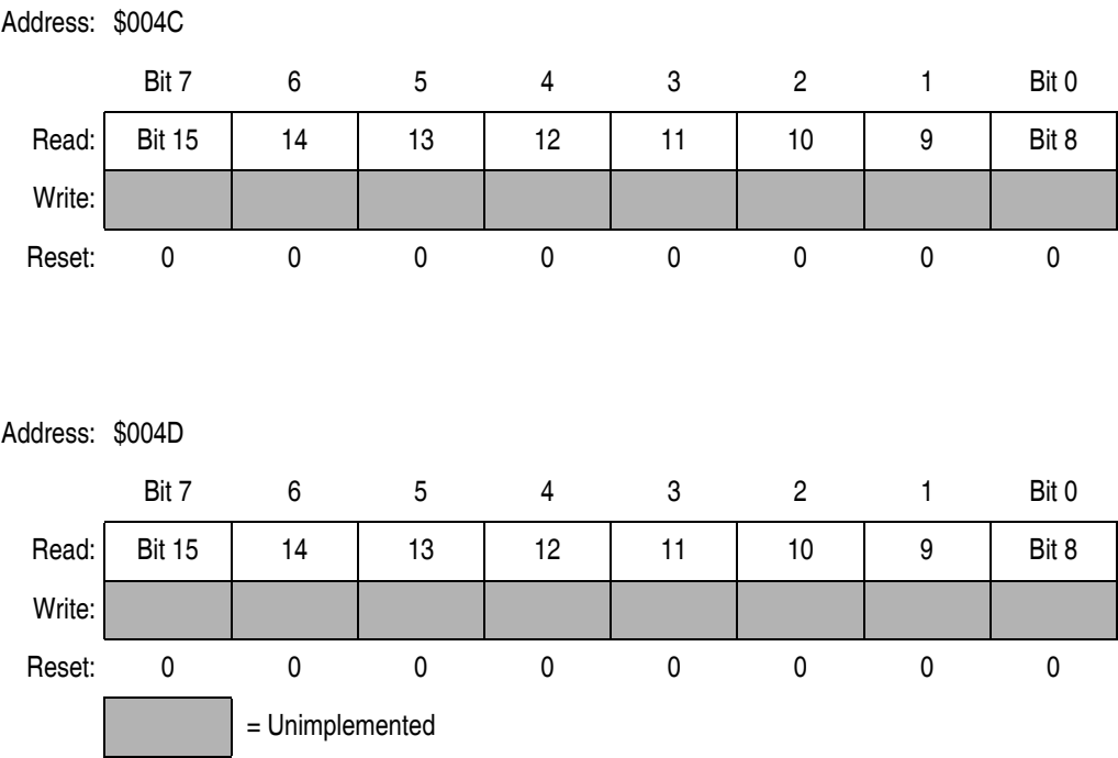
Figure 20-4. PIT Counter Registers (PCNTH–PCNTL)
