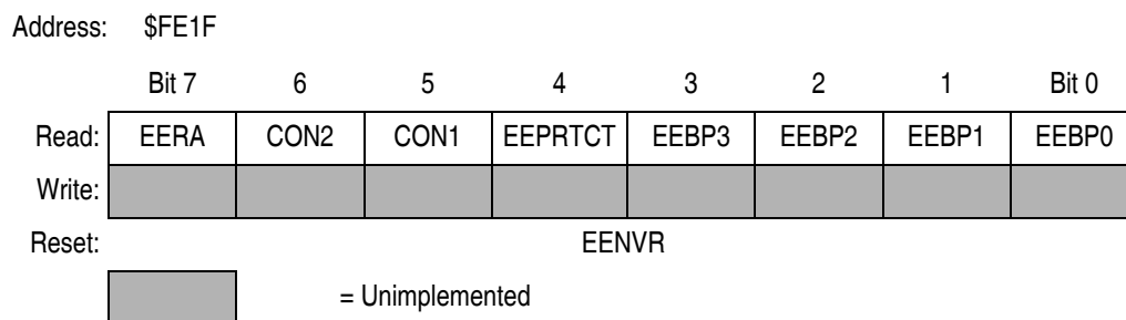
Figure 6-3. EEPROM-1 Array Control Register (EEACR1)
