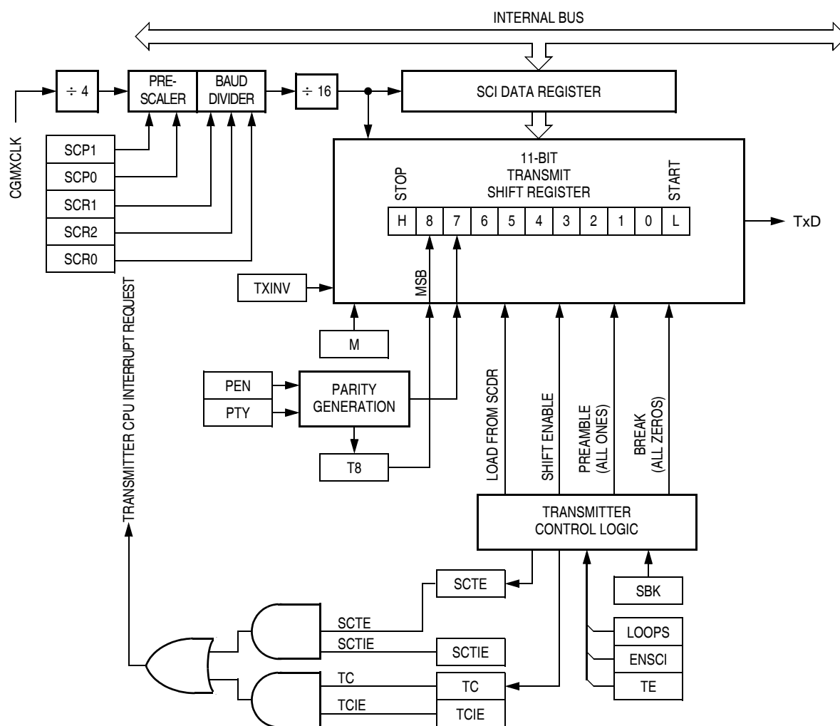
Figure 17-4. SCI Transmitter
