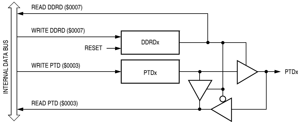
Figure 21-12. Port D I/O Circuit
