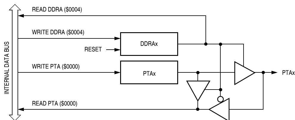
Figure 21-3. Port A I/O Circuit
