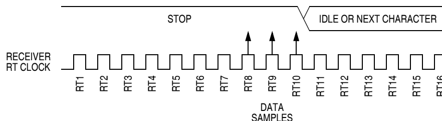
Figure 17-10. Fast Data
