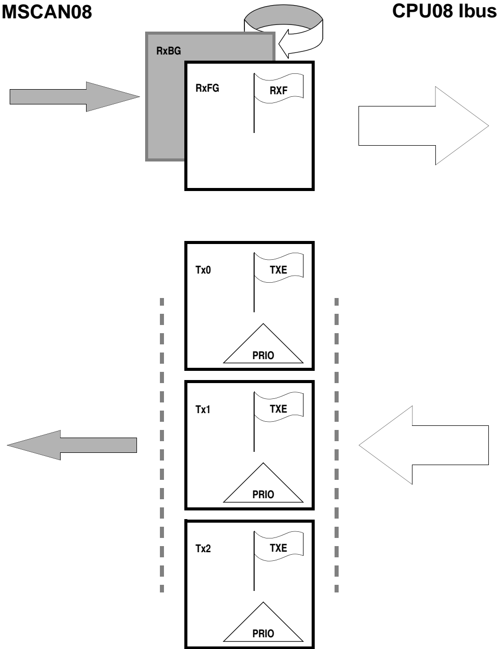
Figure 22-2. User Model for Message Buffer Organization
