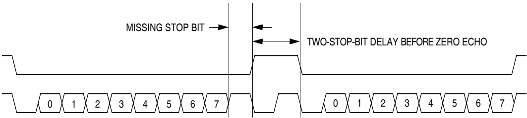
Figure 13-5. Break Transaction
