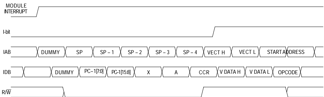
Figure 7. Interrupt entry
