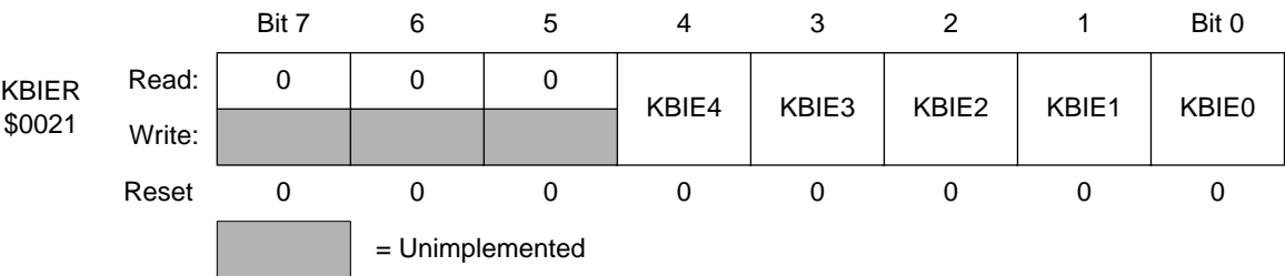
Figure 7. Keyboard interrupt enable register (KBIER)
