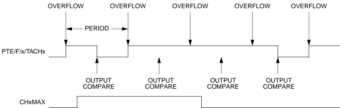
Figure 7. CHxMAX Latency
