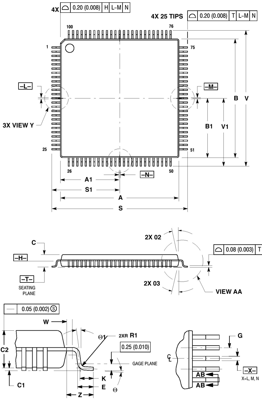
Figure 7. 100-pin QFP
