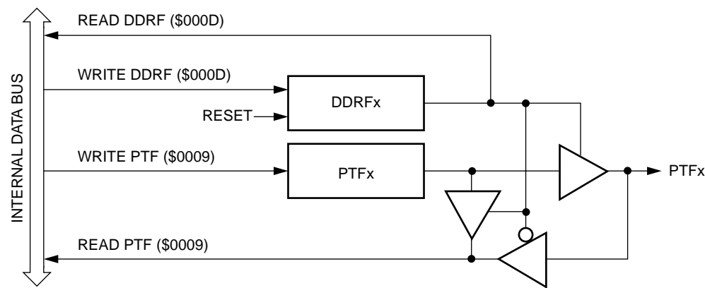
Figure 18. Port F I/O circuit
