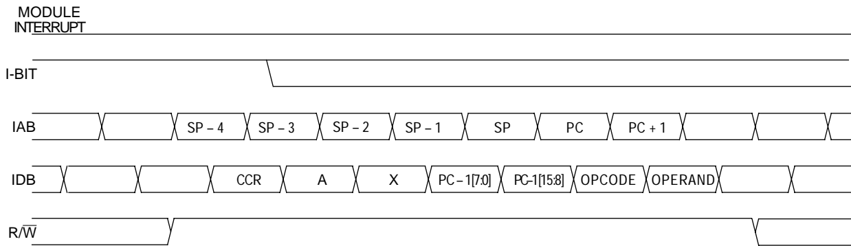
Figure 9. Interrupt recovery
