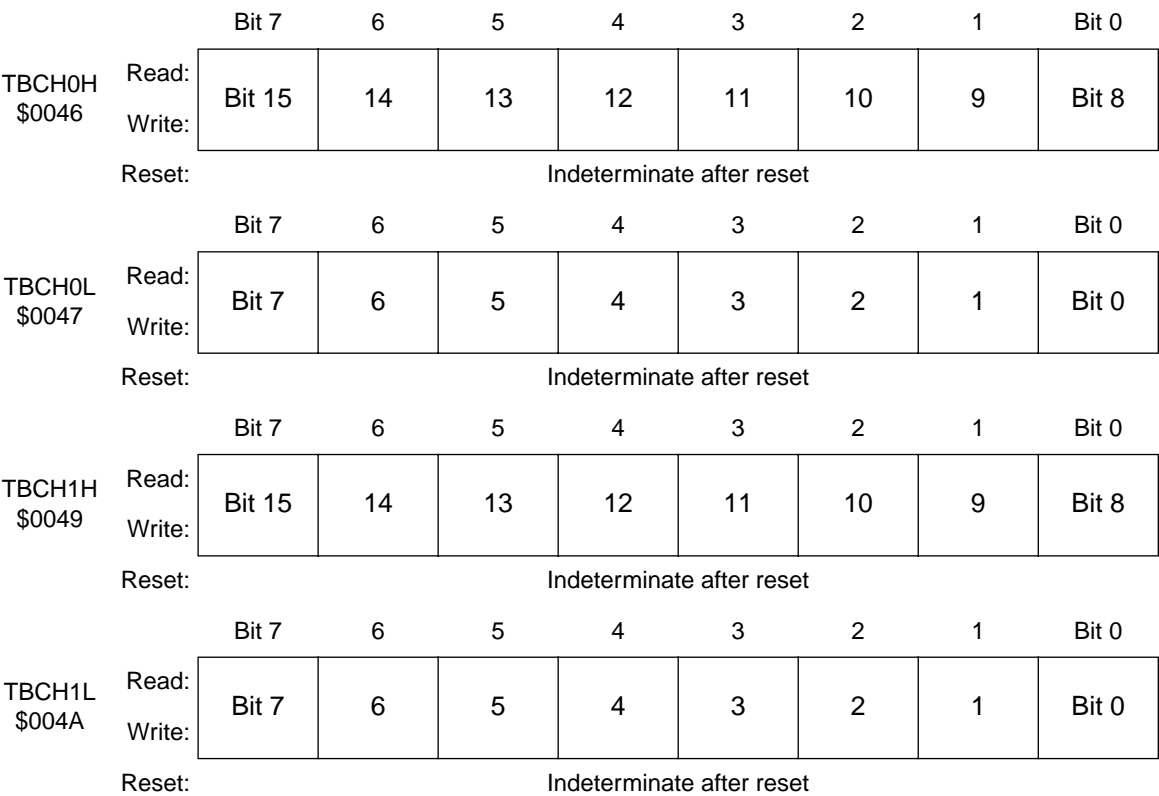
Figure 16. TIMB channel registers (TBCH0H/L–TBCH1H/L)
