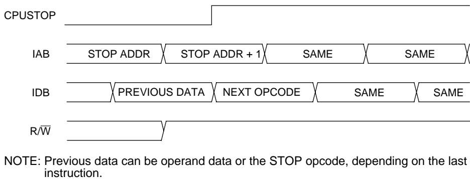
Figure 14. STOP mode entry timing
