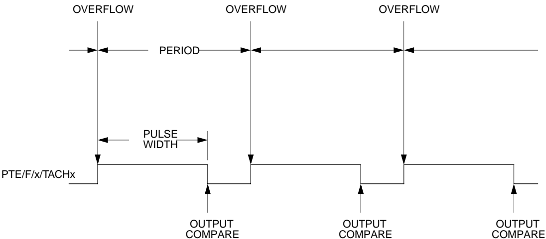
Figure 2. PWM period and pulse width
