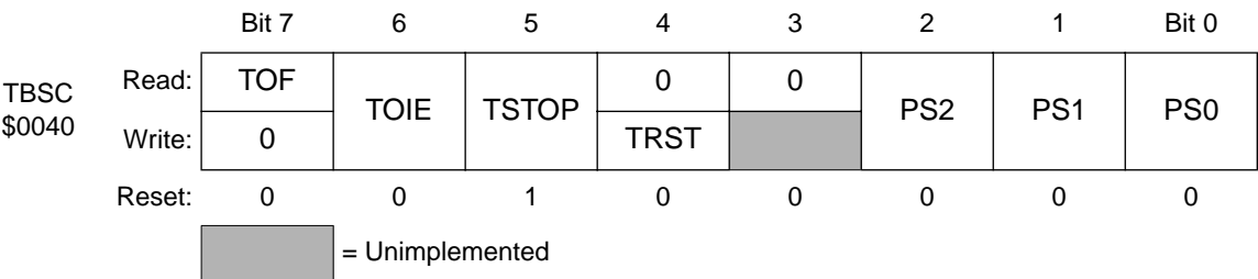
Figure 11. TIMB status and control register (TBSC)
