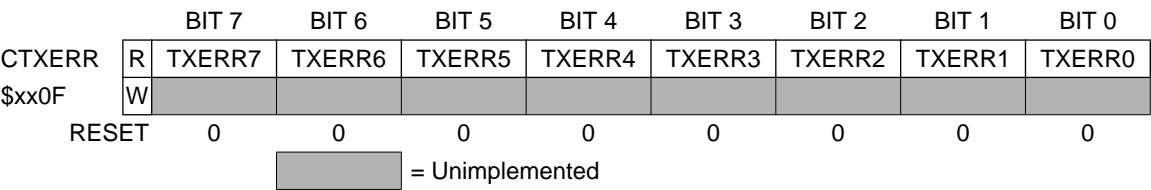
Figure 24. Transmit Error Counter
