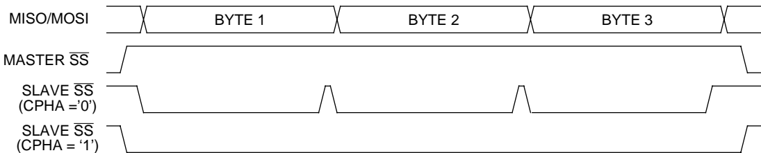
Figure 12. CPHA/ \overline{SS} timing
