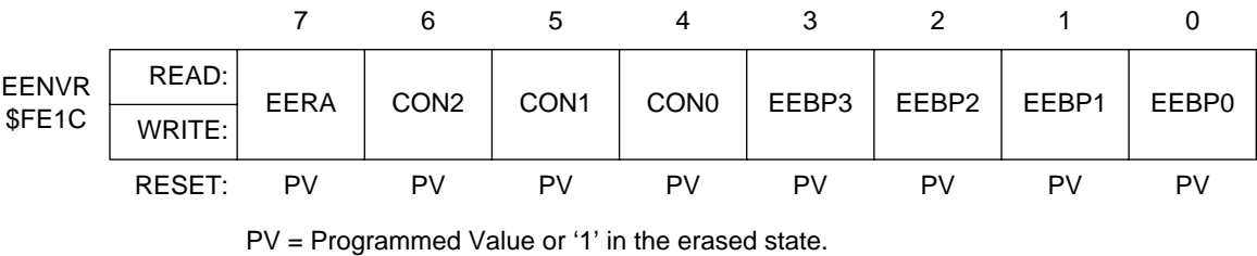
Figure 2. EEPROM non-volatile register (EENVR)
