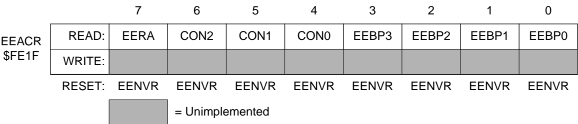
Figure 3. EEPROM array control register (EEACR)
