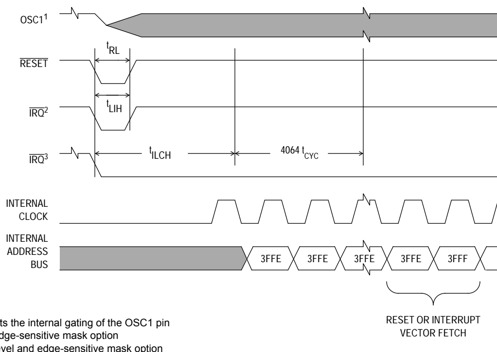
Figure 6-1. Stop Recovery Timing Diagram
