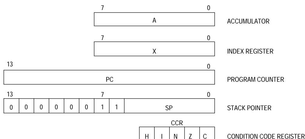
Figure 3-1. Programming Model
