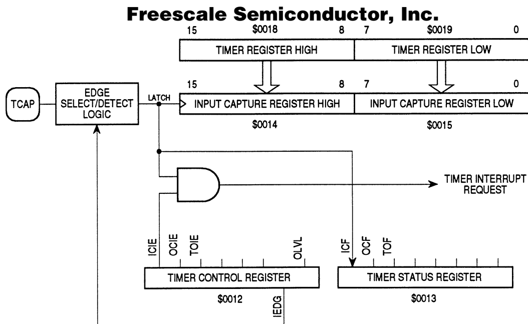
Figure 8-2. Input Capture Operation
