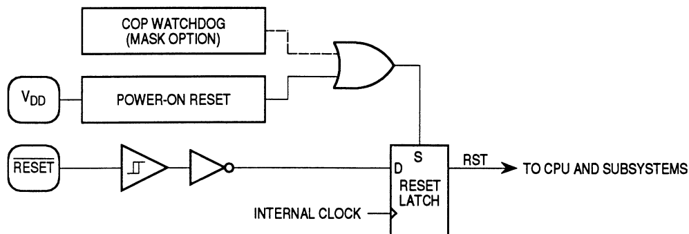
Figure 5-1. Reset Sources
