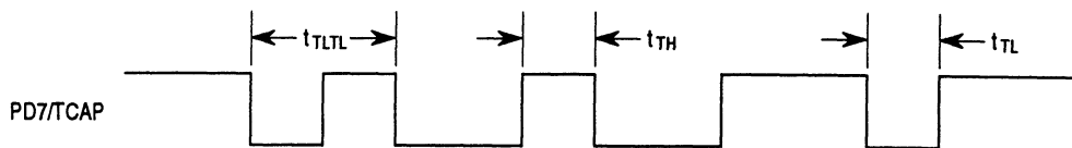
Figure 13-4. TCAP Timing
