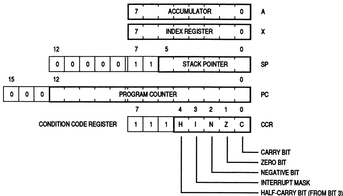
Figure 3-2. Programming Model
