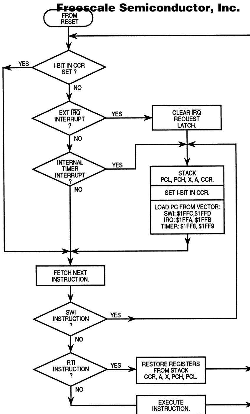
Figure 4-3. Reset and Interrupt Flowchart
