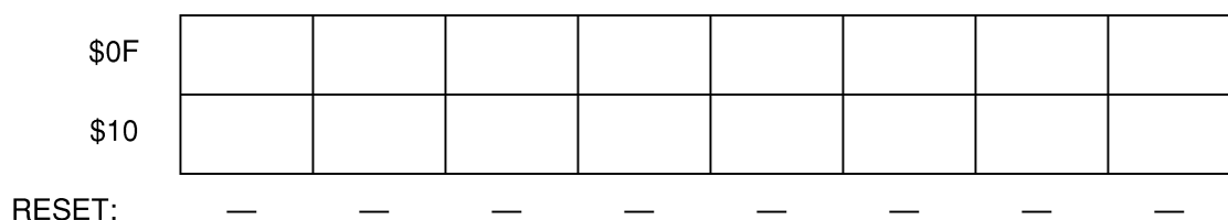
Figure 9-6 PWM Data Registers
