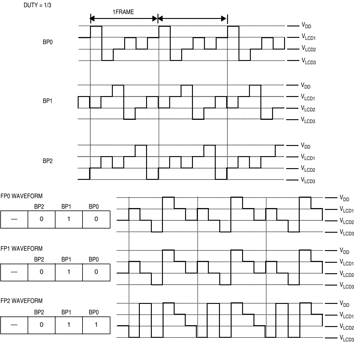
Figure 11-10. BP0–BP2 and FP0–FP2 Output Waveforms
