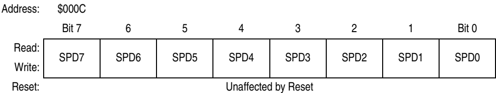
Figure 10-4. SPI Data Register (SPDR)
