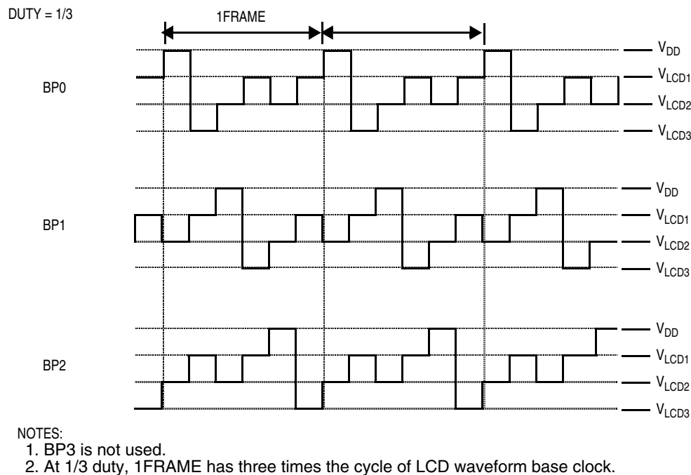
Figure 11-5. 1/3 Duty LCD Backplane Driver Waveforms
