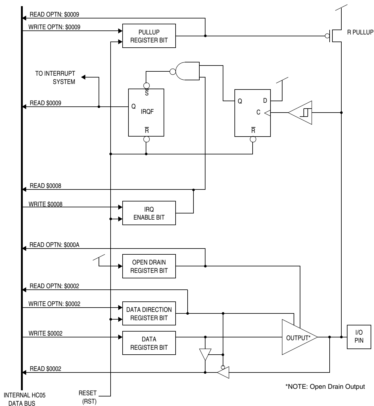
Figure 7-16. PC3/IRQ Circuitry
