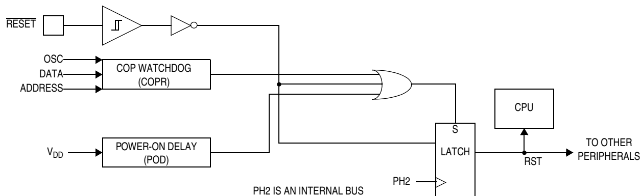
Figure 5-1. Reset Block Diagram
