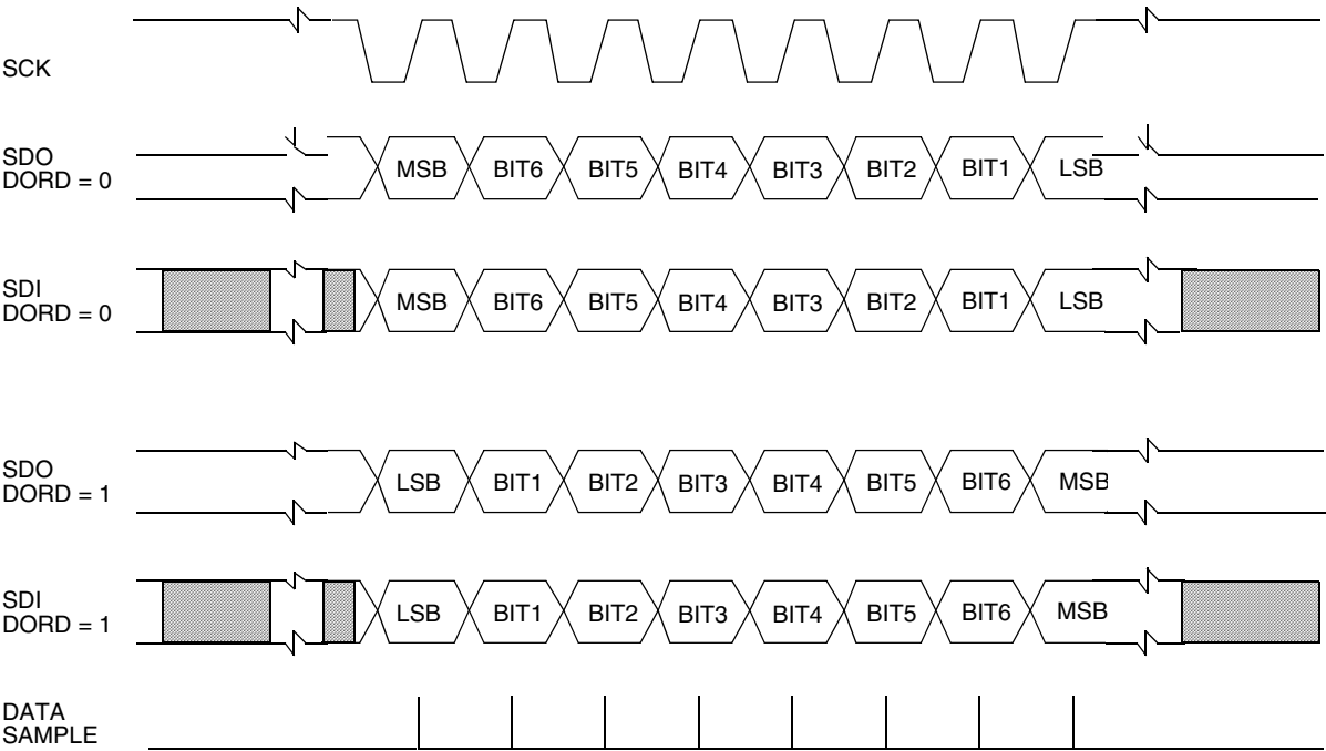
Figure 10-5. Clock/Data Timing
