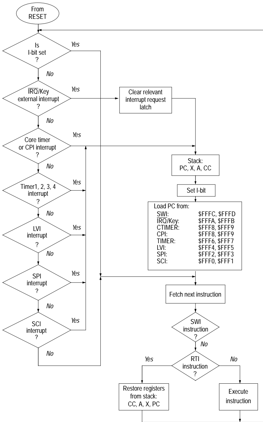
Figure 14-1 Interrupt flowchart
