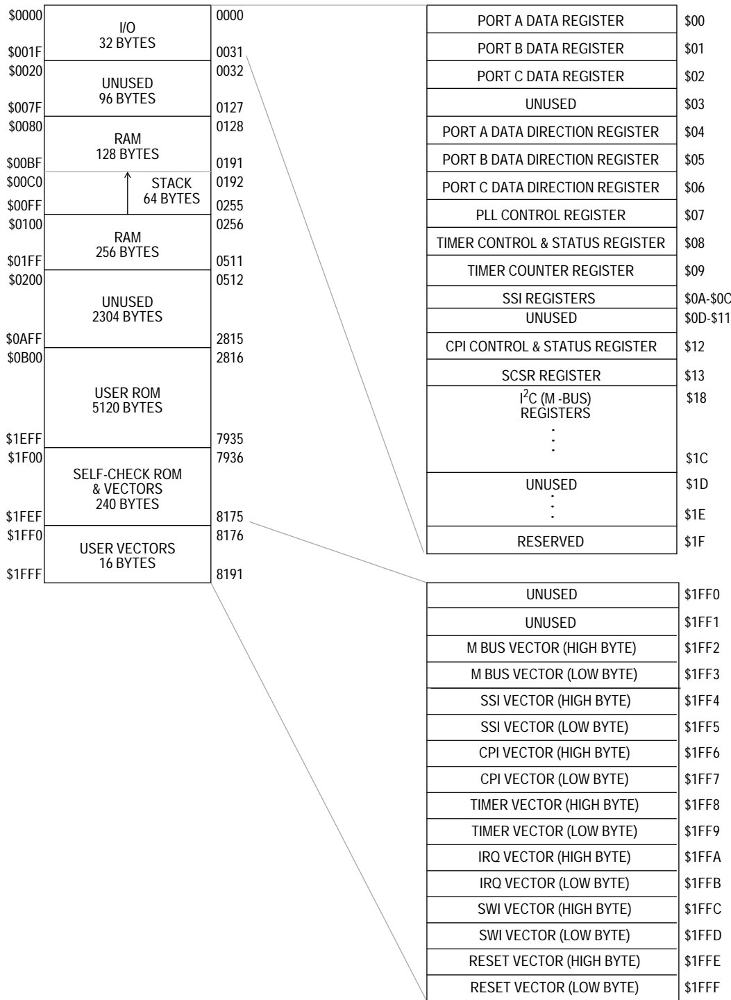
Figure 2-1. Memory Map
