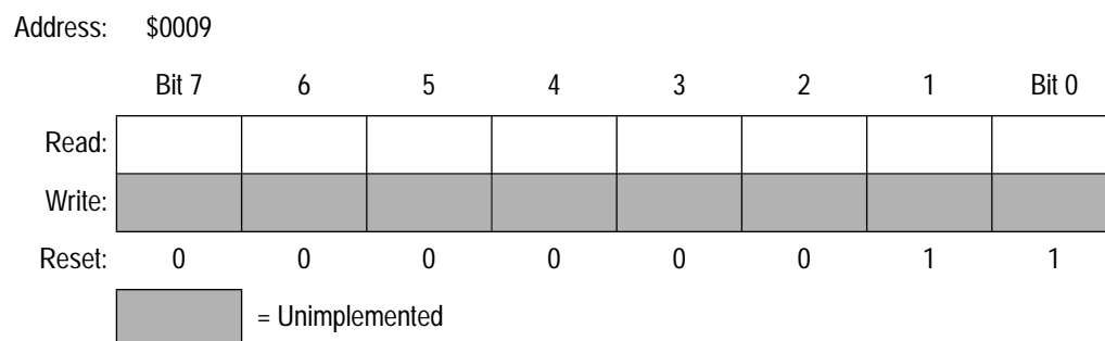
Figure 8-3. Timer Counter Register (TCR)
