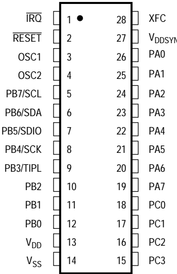
Figure 1-2. Single-Chip Mode Pinout
