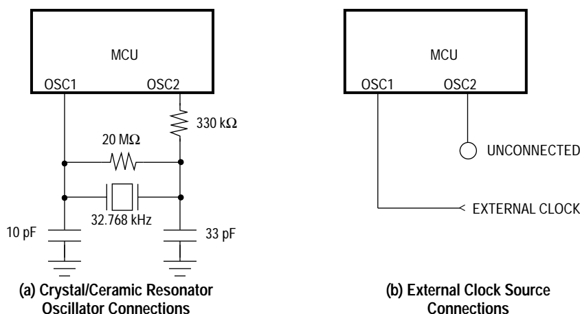
Figure 1-3. Oscillator Connections
