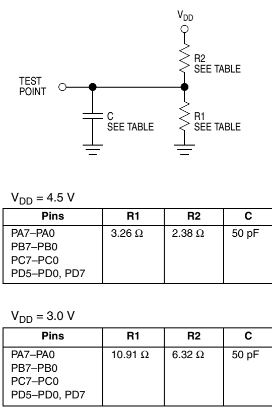
Figure 12-1. Test Load
