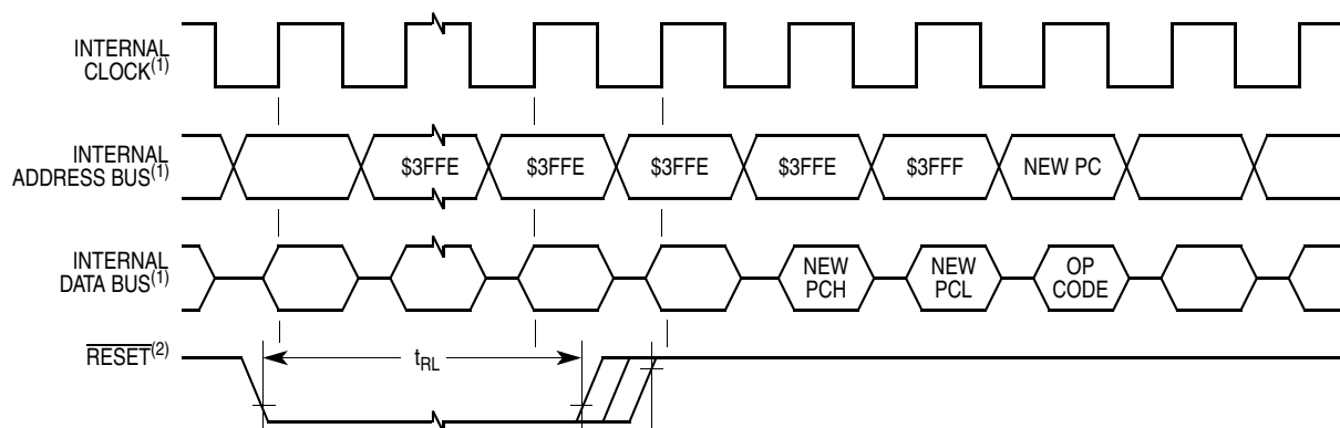
Figure 12-7. Power-On Reset Timing Diagram
