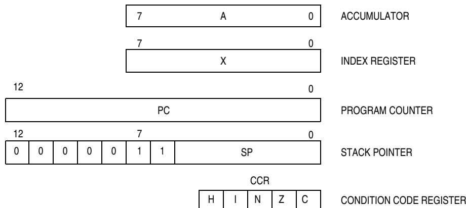
Figure 3-1. Programming Model
