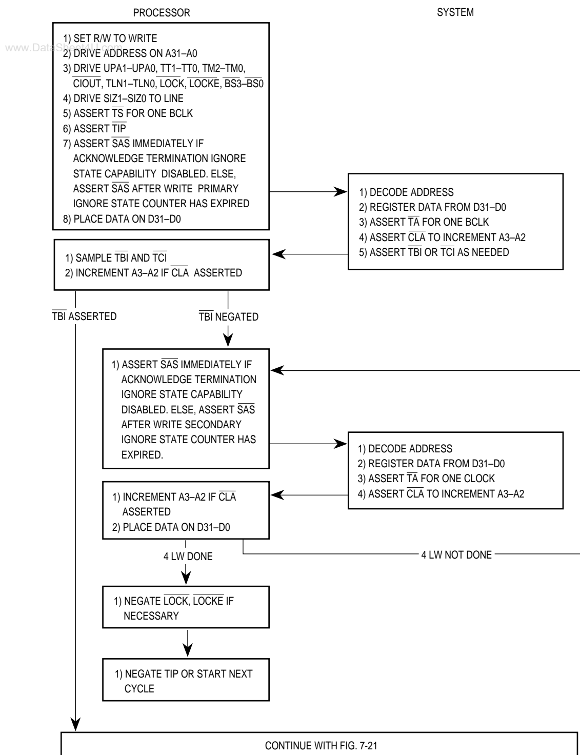
Figure 7-20. Line Write Cycle Flowchart
