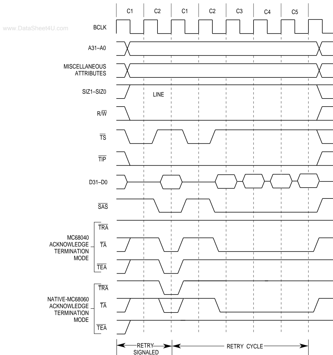
Figure 7-40. Line Write Retry Bus Cycle Timing
