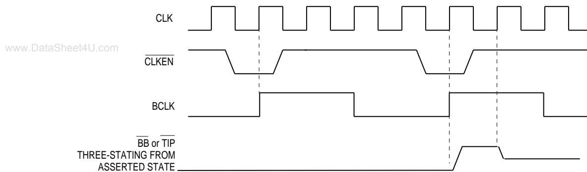
Figure 7-4. Quarter-Speed Clock
