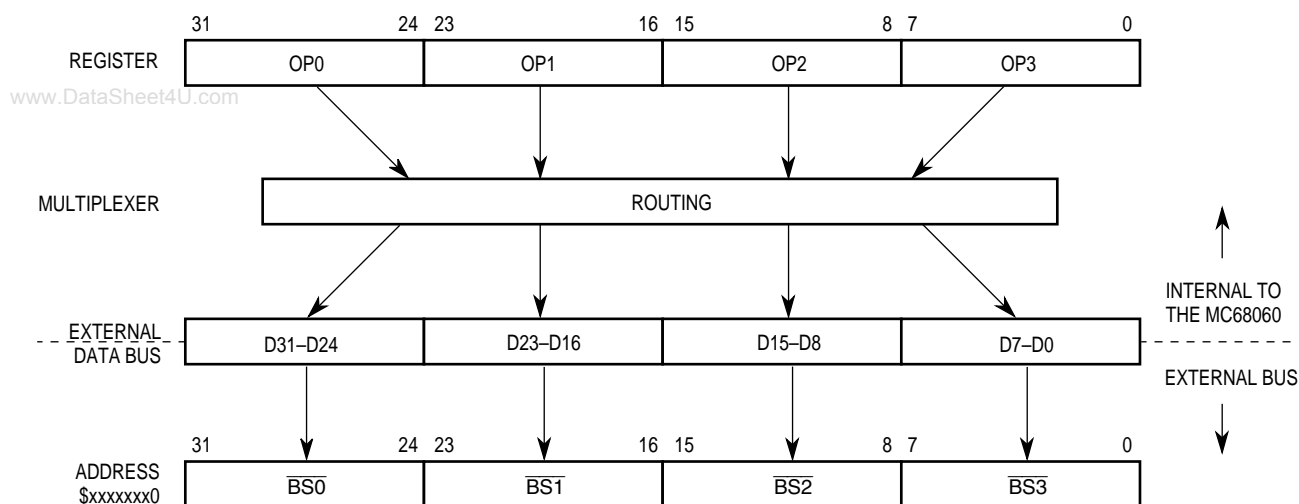
Figure 7-7. Data Multiplexing
