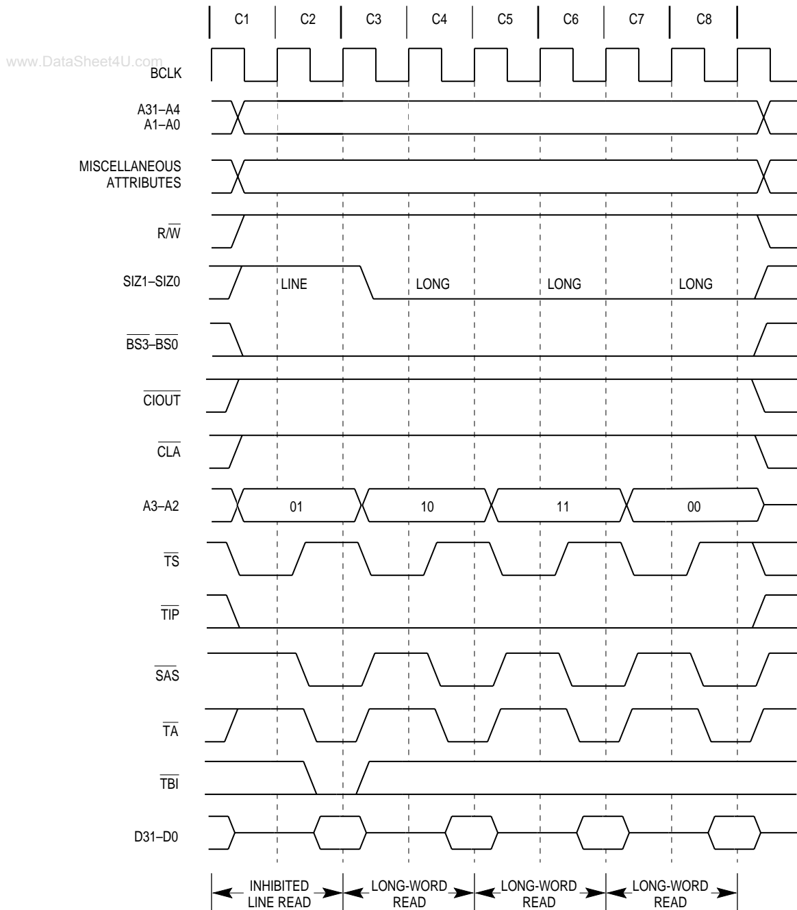
Figure 7-17. Burst-Inhibited Line Read Bus Cycle Timing
