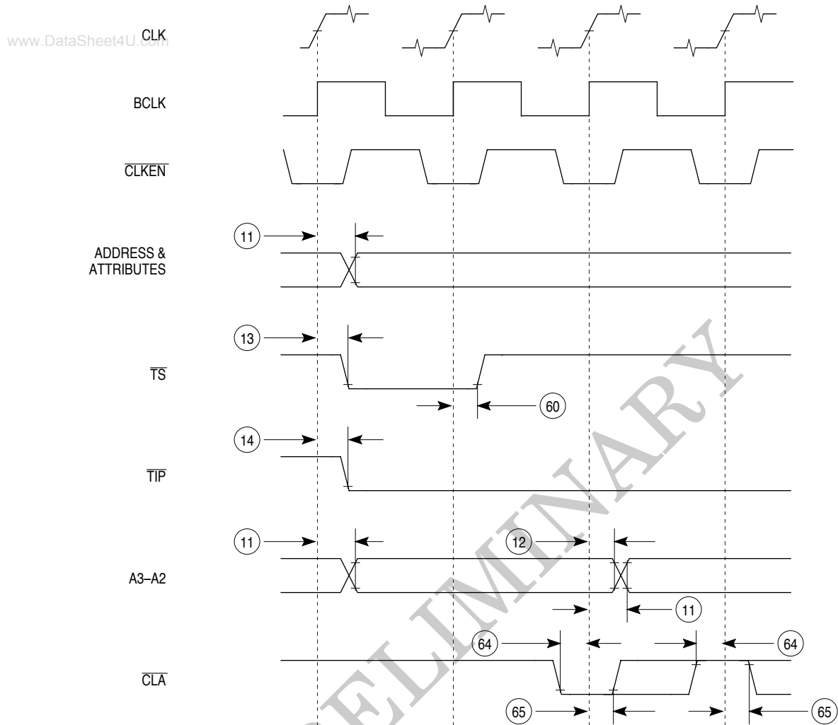
Figure 12-6. CLA Timing
