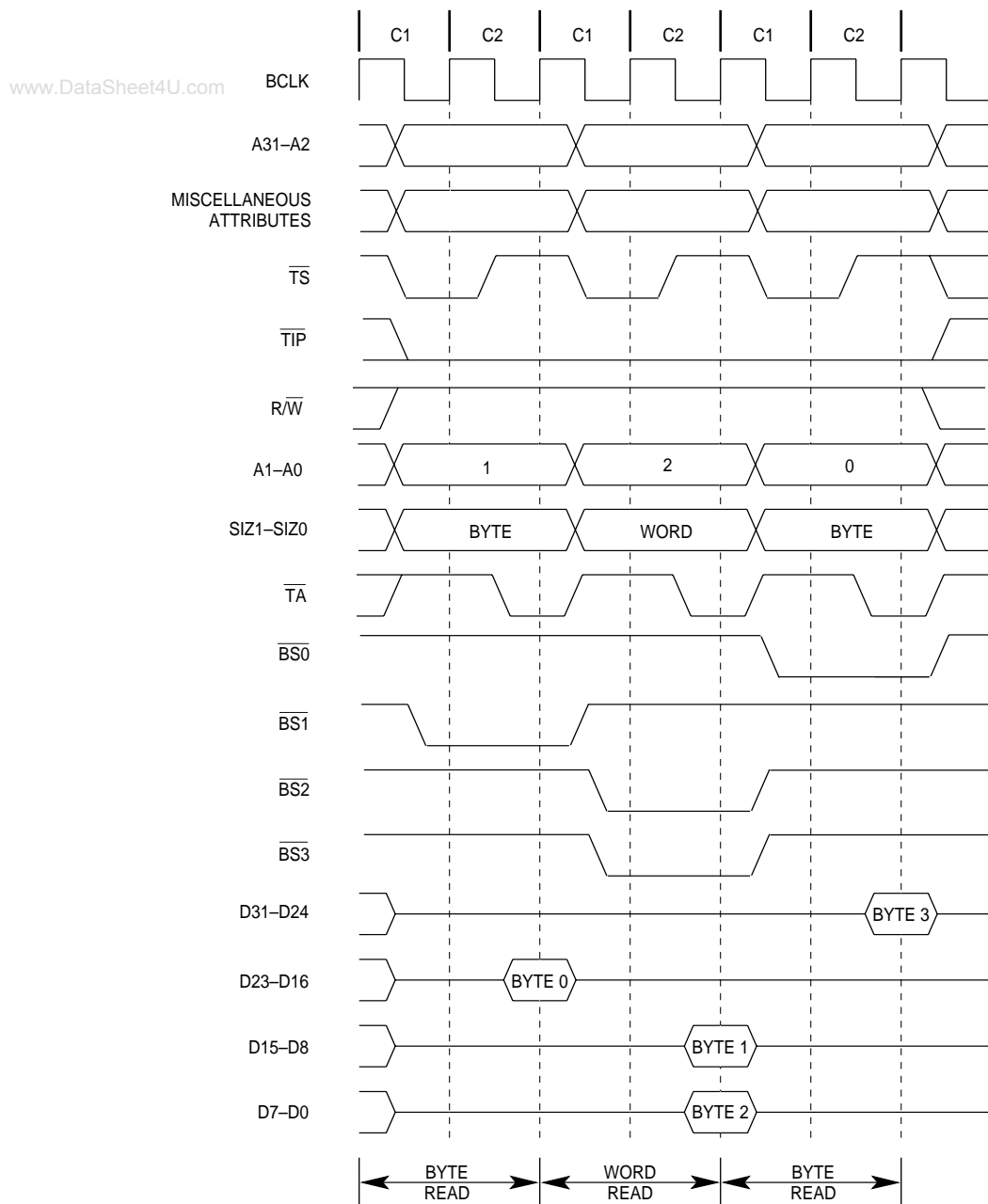
Figure 7-11. Misaligned Long-Word Read Bus Cycle Timing
