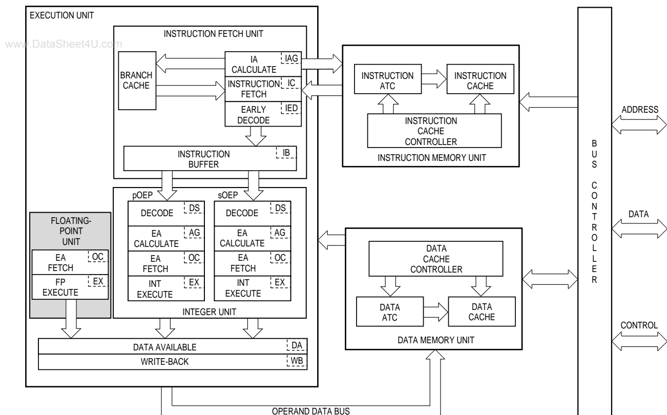
Figure 6-1. Floating-Point Unit Block Diagram
