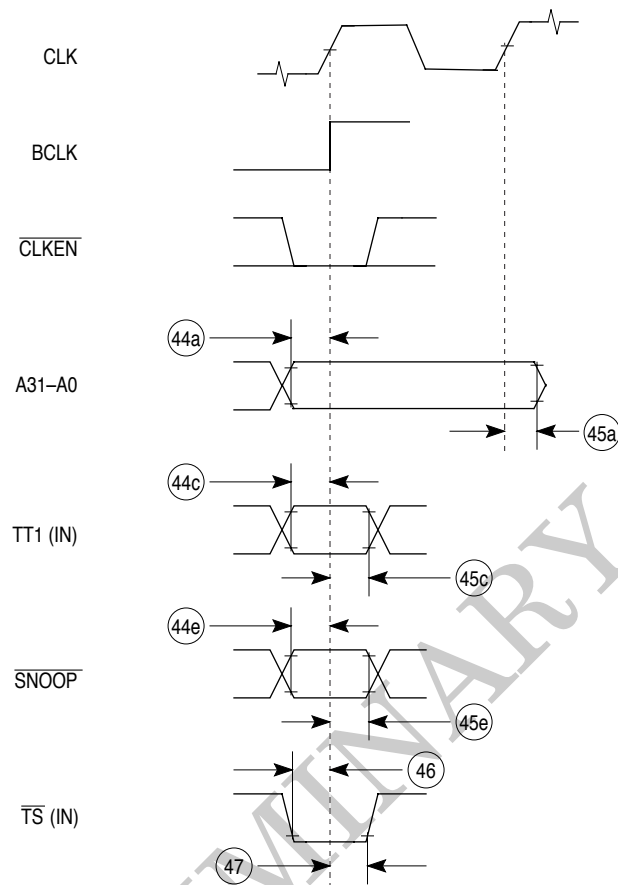
Figure 12-7. Snoop Timing
