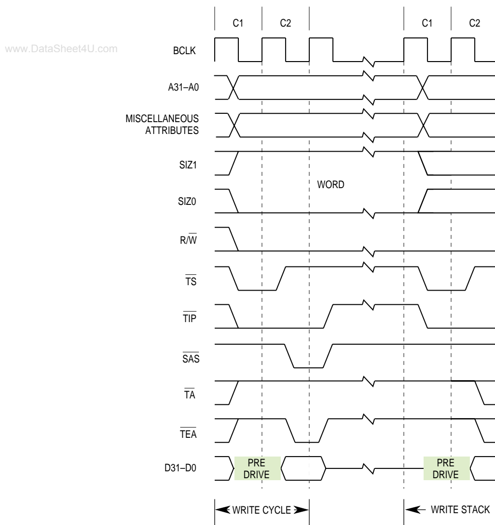
Figure 7-37. Word Write Access Bus Cycle Terminated with \overline{TEA} Timing
