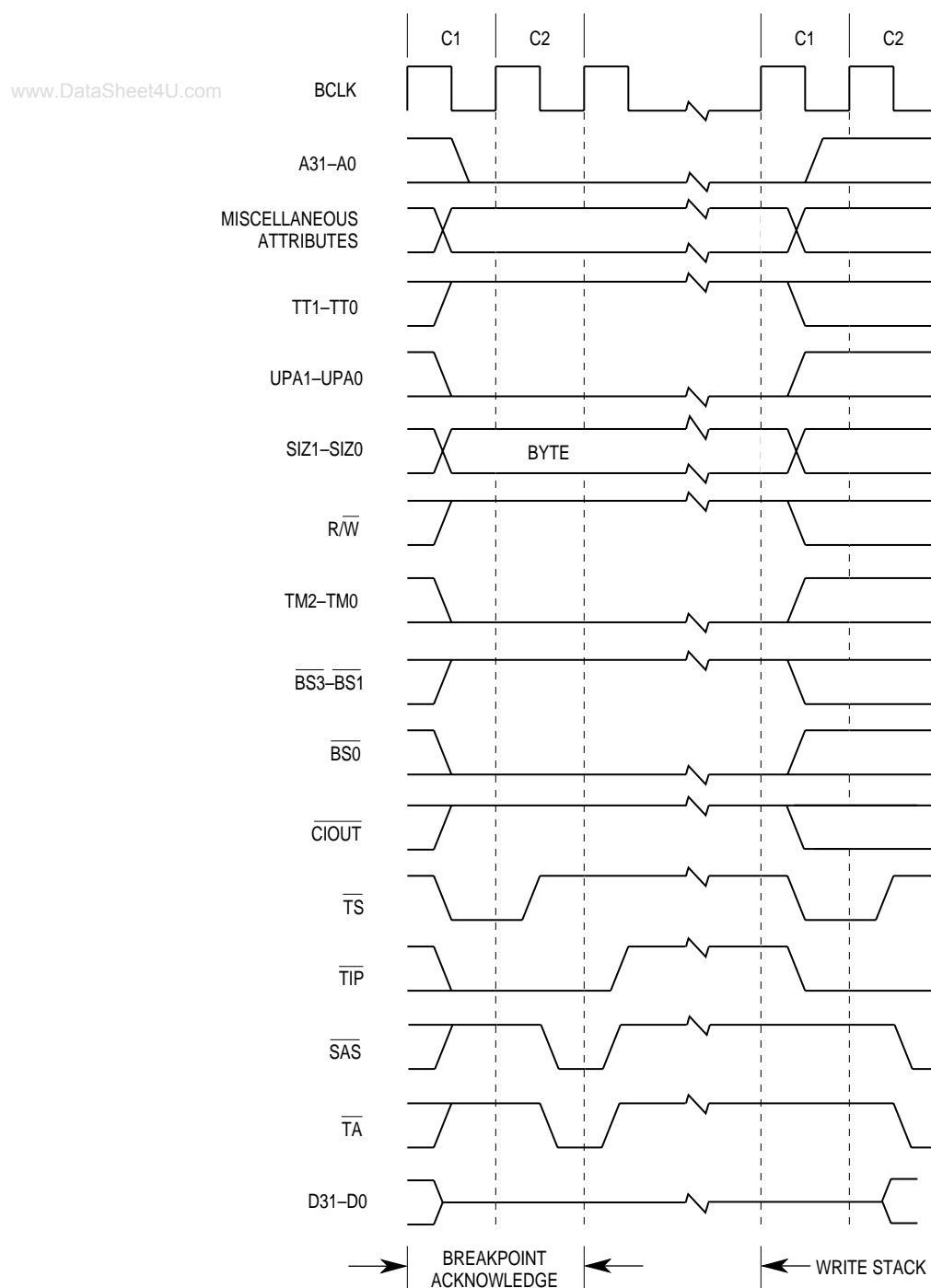
Figure 7-31. Breakpoint Interrupt Acknowledge Bus Cycle Timing
