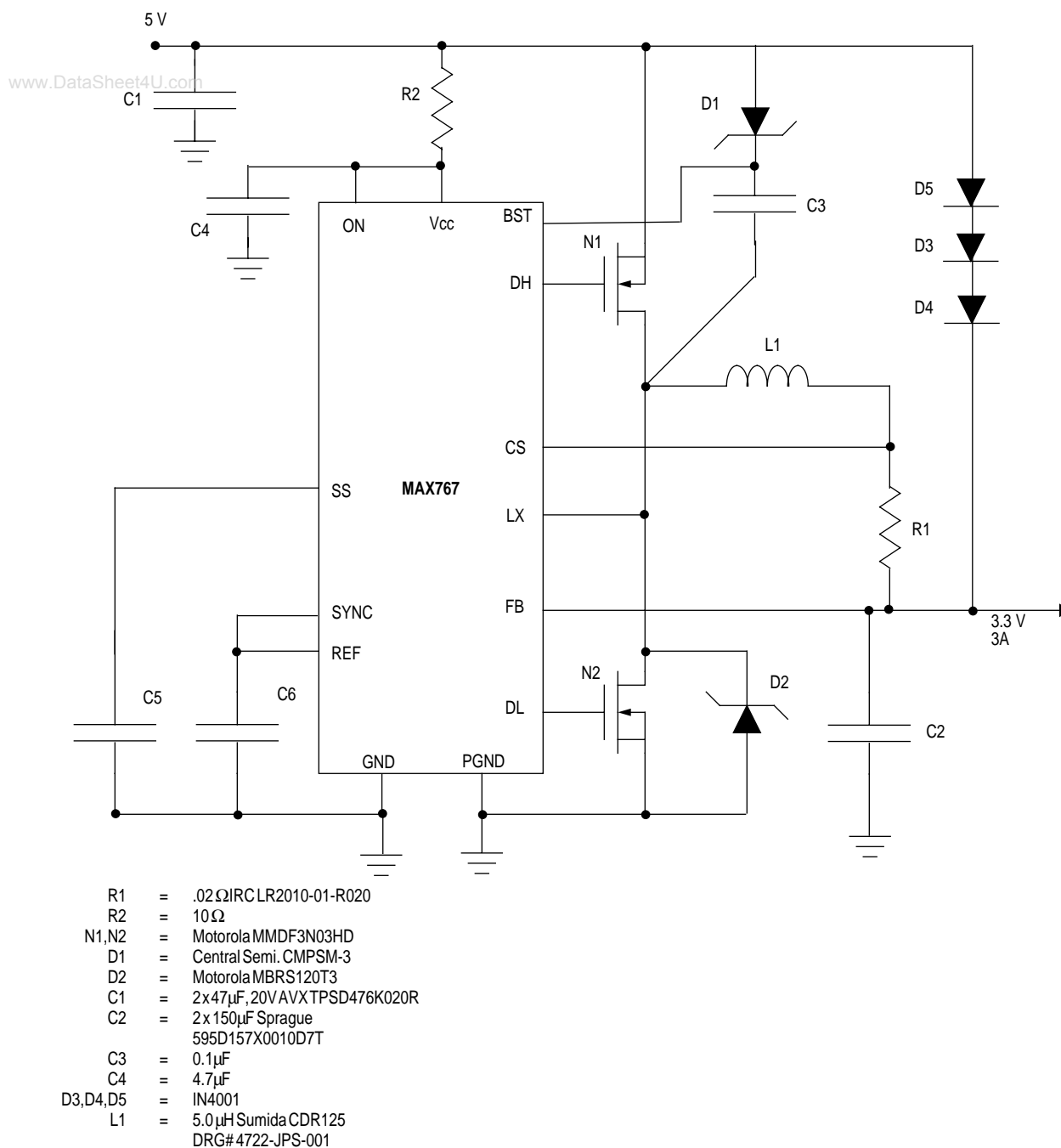
Figure 11-4. MAX767 Voltage Regulator Solution
