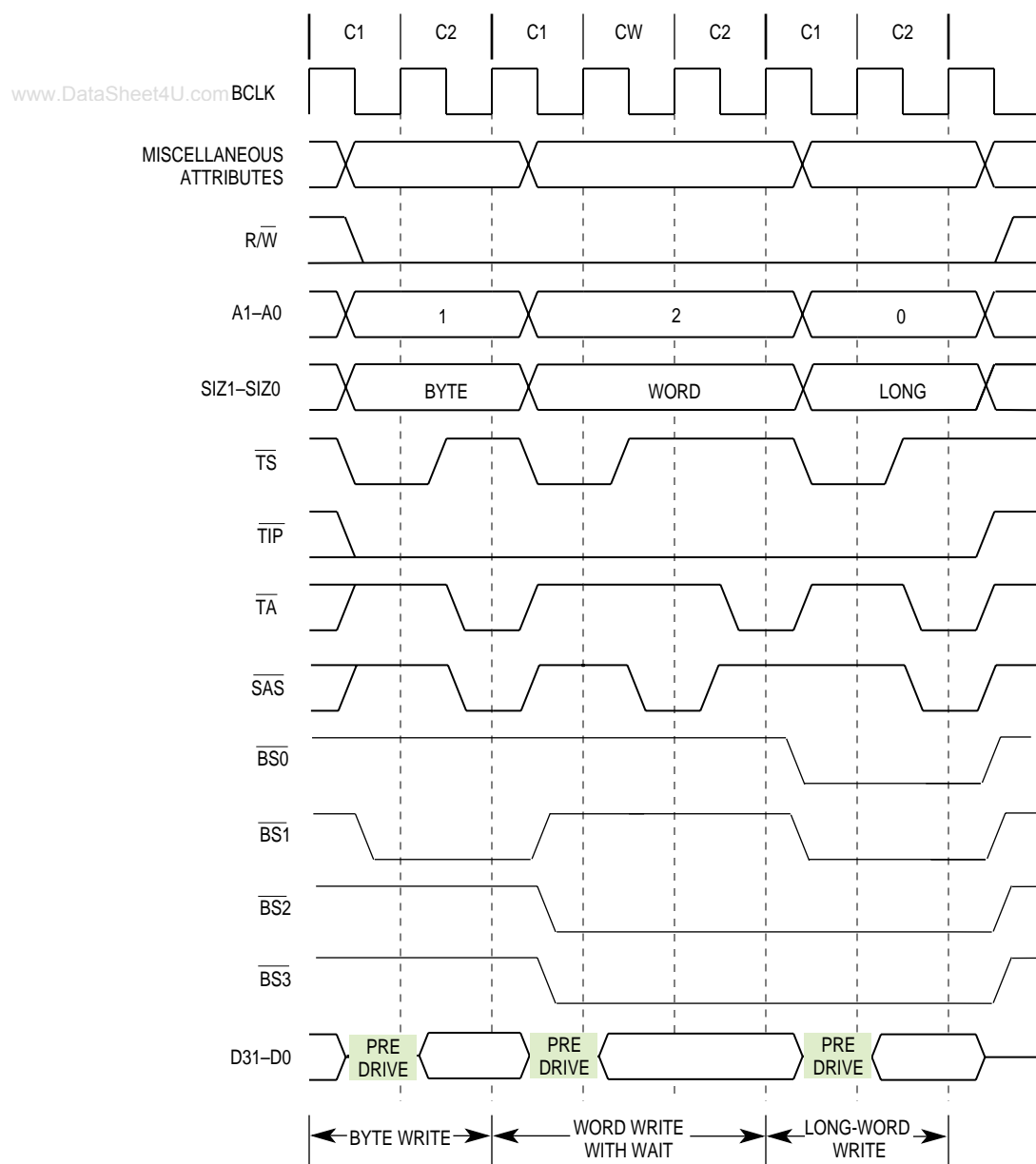
Figure 7-19. Long-Word Write Bus Cycle Timing
