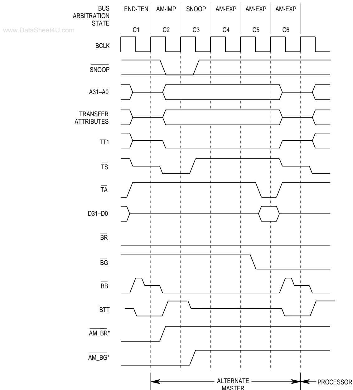
Figure 7-47. Snoop Bus Cycle
