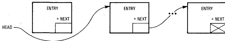
Figure 3-3. Linked List Deletion
