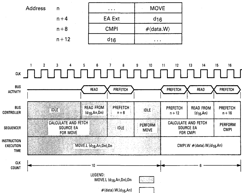
Figure 11-5. Processor Activity — Odd Alignment
