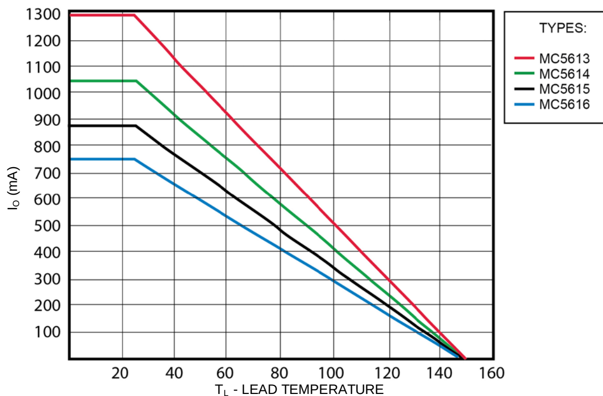
FIGURE 1 Average Rectified Current vs. Lead Temperature Lead Temperature (°C) (L=3/8 inch)
