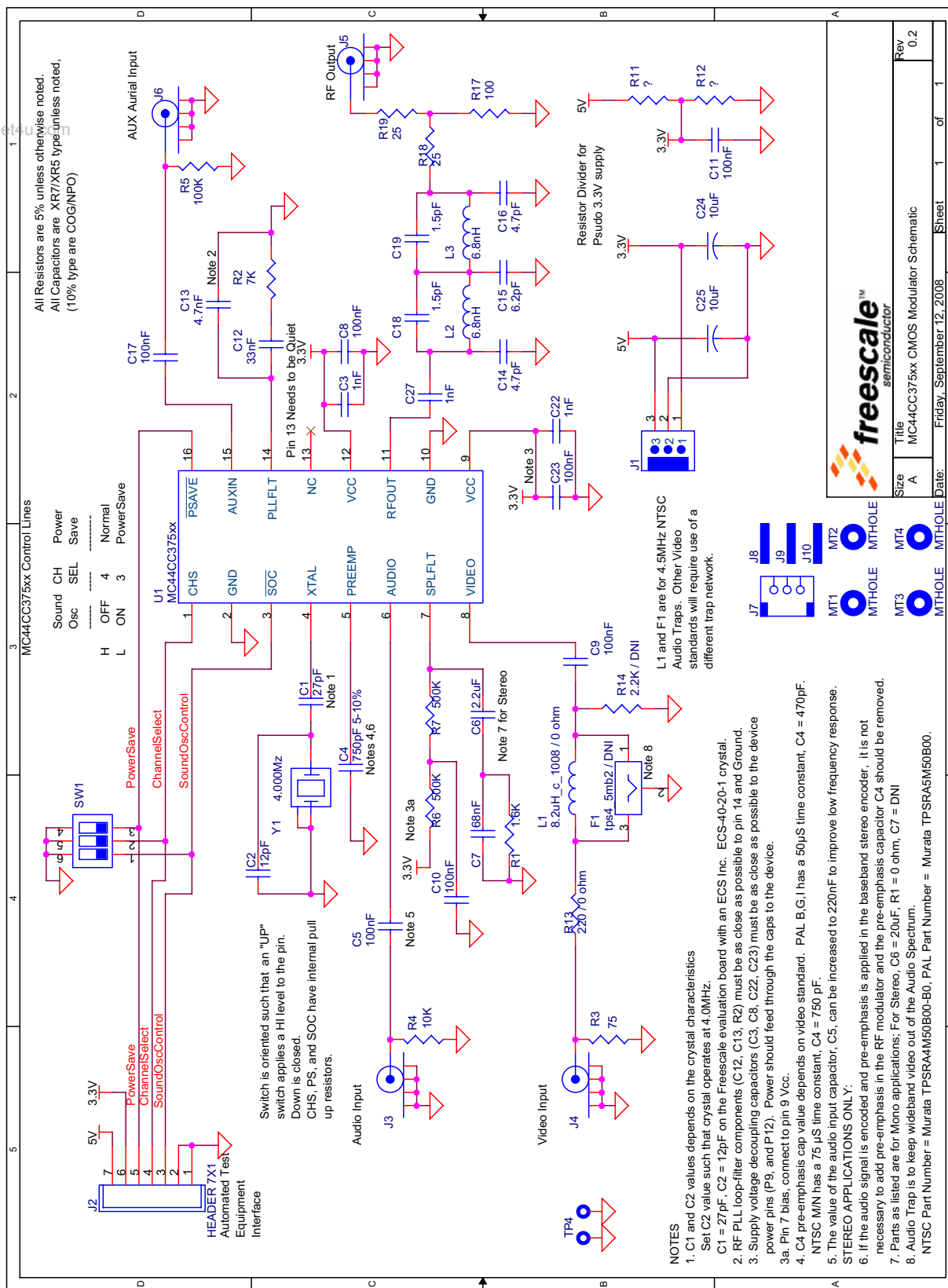
Figure 4. MC44CC375AV Application Schematic
