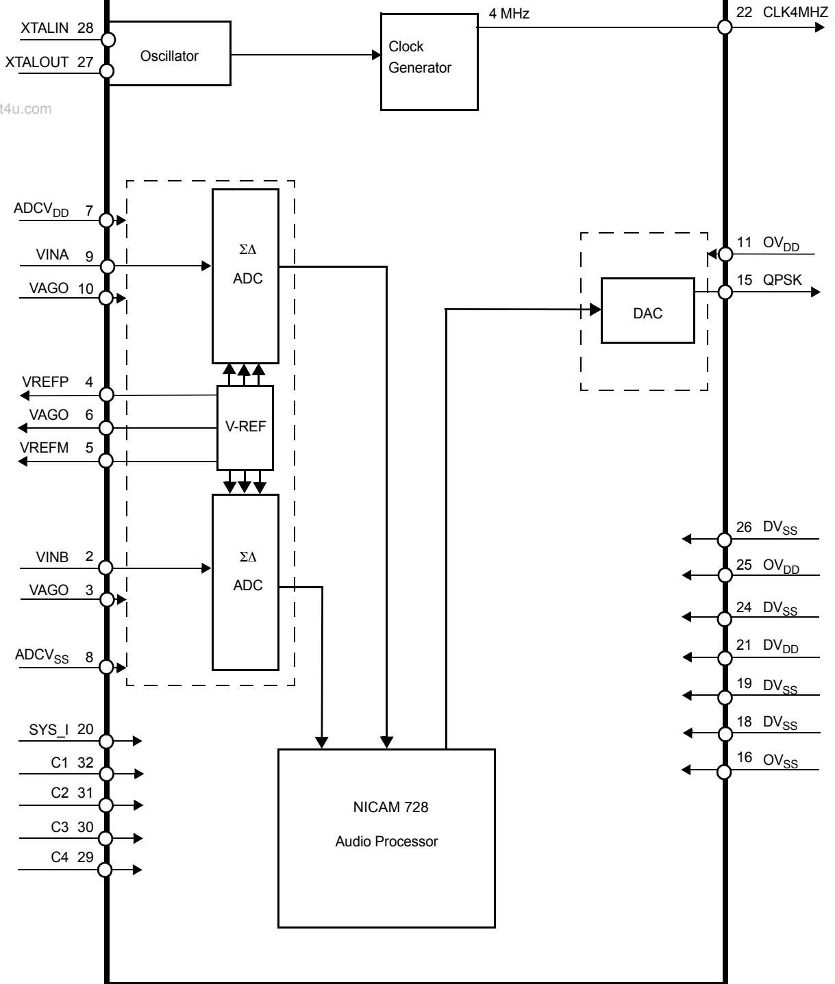
Figure 1. MC44C404 Block Diagram
