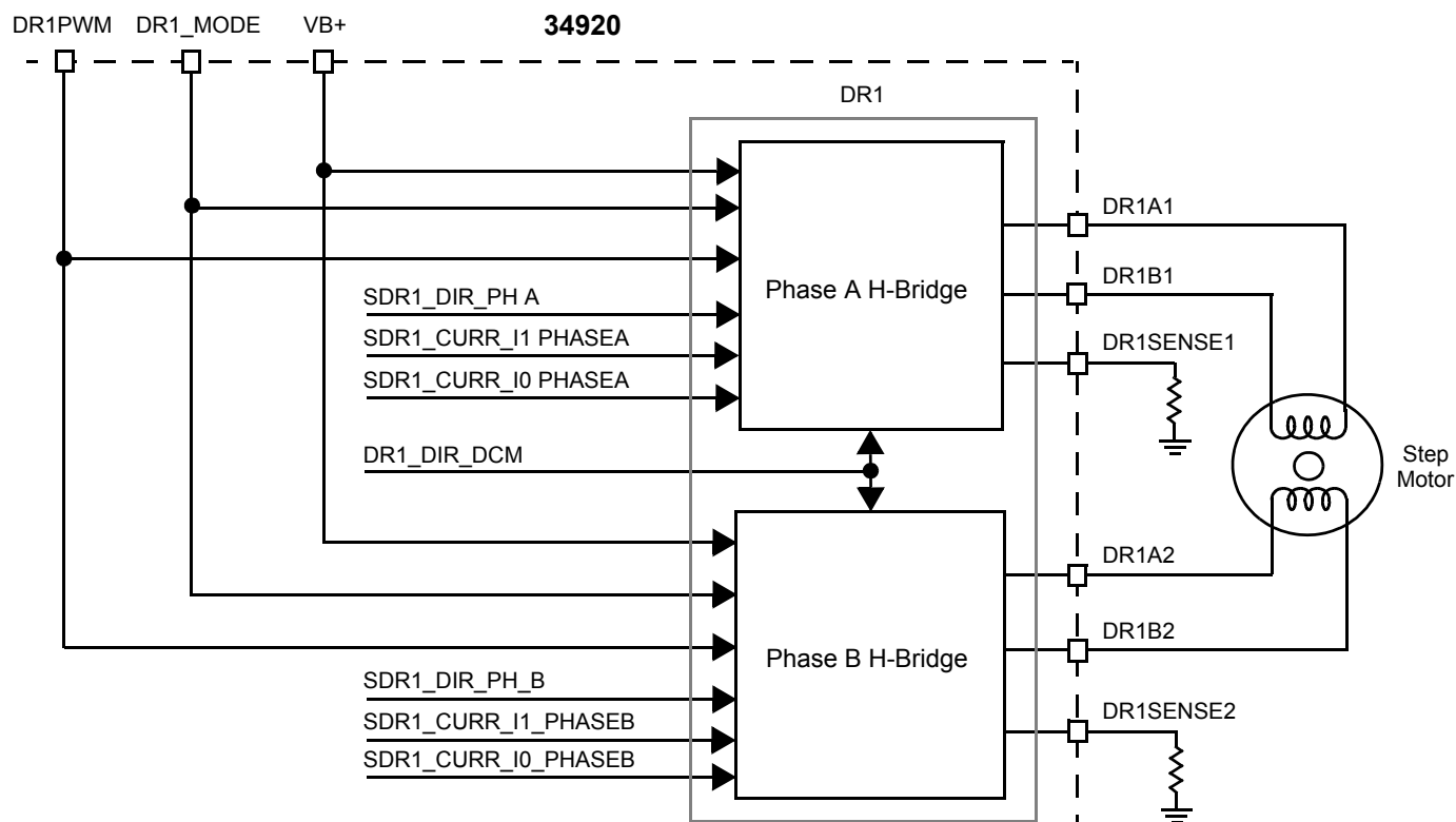
Figure 5. Simplified Step Application Diagram Showing 1 of 2 Step Drive Circuits
