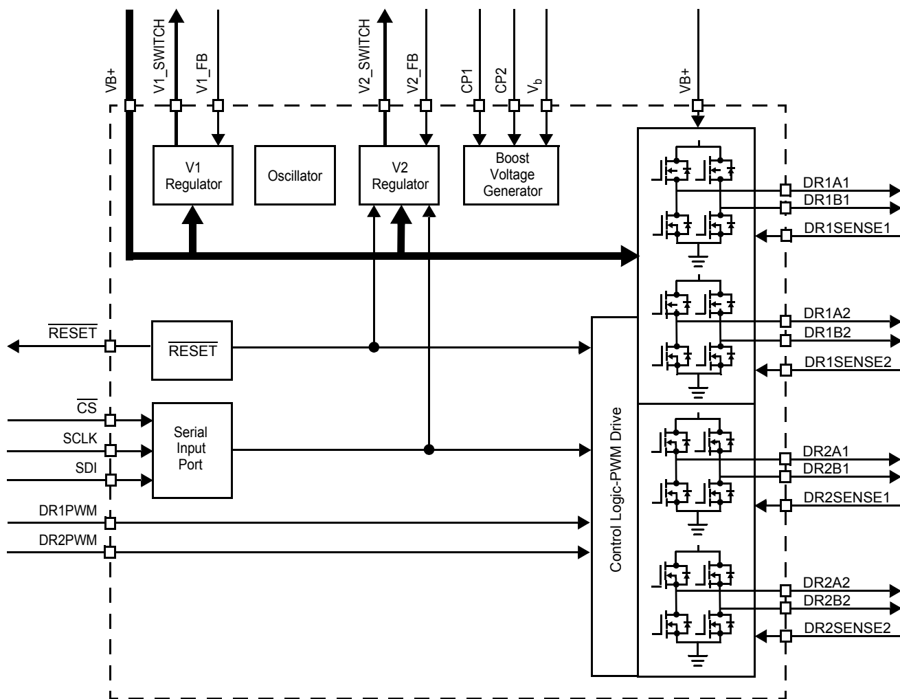
Figure 1. 34920 Simplified Internal Block Diagram
