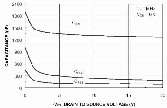
Figure 8. Capacitance Characteristic
