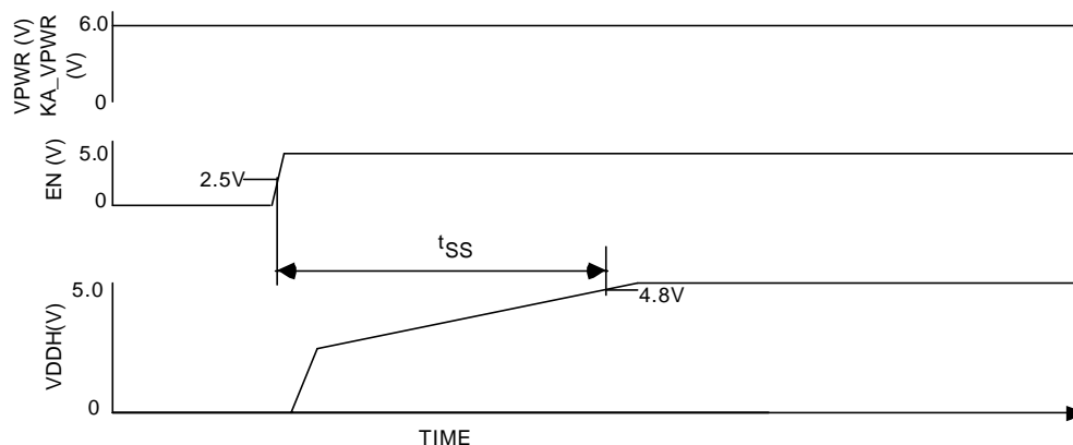
Figure 4. Soft-Start Time
