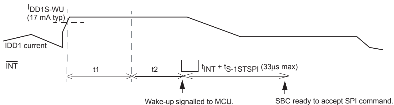
Figure 32. Overcurrent Wake-up
