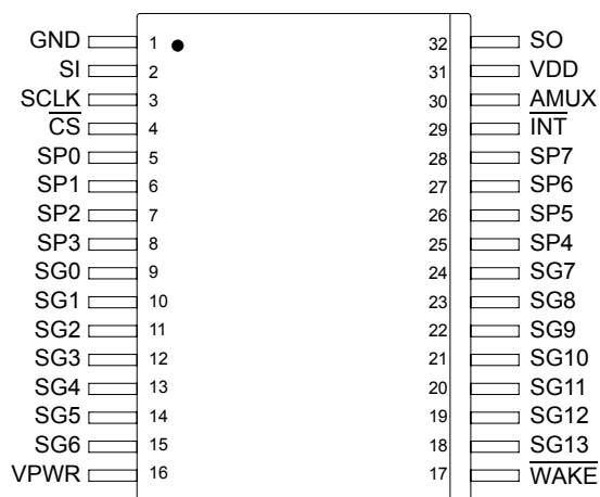
Figure 3. 33972 Pin Connections
