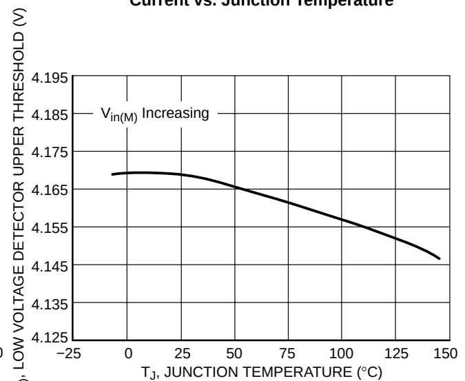
Figure 18. Low Voltage Detector Upper Threshold vs. Junction Temperature
