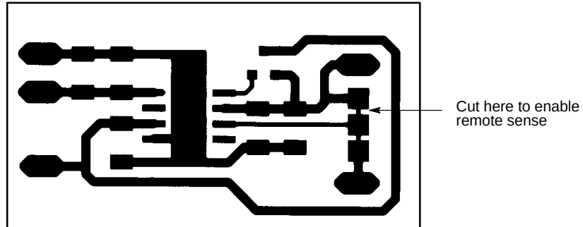
Figure 27. Demonstration Board Top Layer
